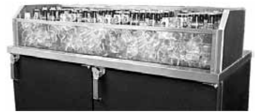
Factory installed GDU on 1.5" high insulated cooler top (not std 1" high) with built-in drain pan
