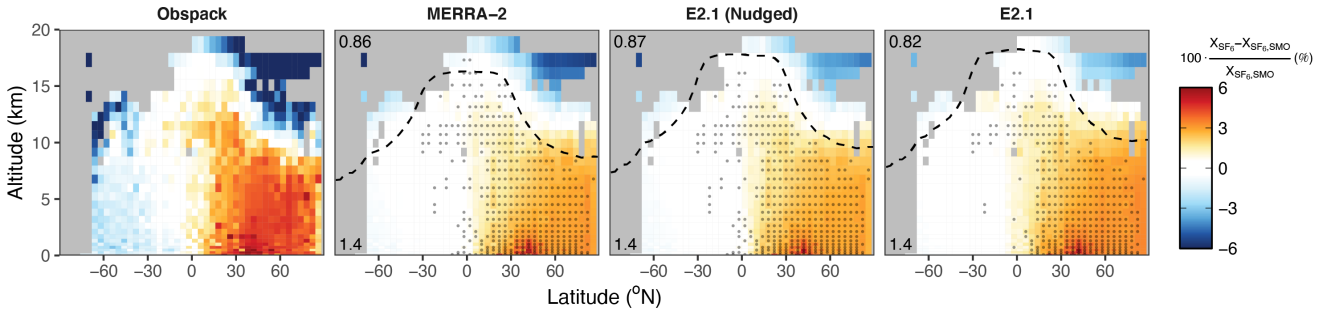
Figure 9. Lower atmospheric gradients of SF 6 shown as zonal mean percent difference with respect to Cape Matatula, American Samoa (SMO; 14.2°S, 170.6°W; 42 m.a.s.l.) for 2005-2014 C.E. The left panel shows observed values from version 2.1.1 of the NOAA SF 6 ObsPack aggregated at E2.1 vertical resolution. The right three panels show the values from the model driven by the three meteorology products sampled at each observation month and location. Gray dots indicate locations where the simulated gradient is statistically different than the observations with respect to interannual variability ( p -value < 0.05; n = 10 yr). The number in each model panel's top left shows the pattern correlation ( R ) of that simulation to the observations. The lower left number shows the mean absolute percent bias of each simulation relative to the observations. The dashed black line shows each simulation's climatological zonal mean tropopause height.
