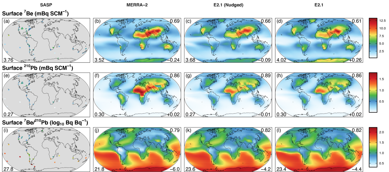
Figure 11. Surface mixing ratios of {}^7\text{Be} (top row; in \text{mBq SCM}^{-1} ; 4.05 \text{ mBq SCM}^{-1} = 1.0 \times 10^{-21} \text{ mol } {}^7\text{Be} / \text{mol air} ), {}^{210}\text{Pb} (middle row; in \text{mBq SCM}^{-1} ; 2.66 \text{ mBq SCM}^{-1} = 1.0 \times 10^{-19} \text{ mol } {}^{210}\text{Pb} / \text{mol air} ), and the \log_{10} -transformed ratio of the {}^7\text{Be} to {}^{210}\text{Pb} activities in surface air (bottom row; unitless). The left column shows long-term mean observations from the DOE Surface Air Sampling Program (SASP) program for 1969–1999 C.E. The {}^7\text{Be} observations have been selected for periods of average solar activity ( \Phi = 670 \pm 50 \text{ MV} from Usoskin et al., 2005). The right three columns show from left to right: values simulated by GEOS-Chem driven by meteorology archived for 2005–2014 C.E. from MERRA-2, E2.1 nudged to MERRA-2, and the free-running E2.1. The number in each panel’s lower left shows the mean value of the observations or models sampled at the observed locations. The top right number shows the pattern correlation ( R ) of the simulated values with the respective observations. The lower right number shows the mean bias of the simulated values with respect to the observations.
