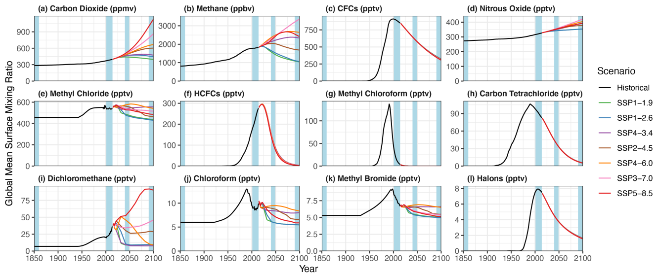
Figure 7. Time series of annual mean CMIP6 surface boundary conditions for 1850-2100 C.E. Individual panels show the temporal evolution of (a) carbon dioxide ( \text{CO}_2 ) in ppmv ( \equiv \mu\text{mol mol}^{-1} ), (b) methane ( \text{CH}_4 ) in ppbv ( \equiv \text{nmol mol}^{-1} ), (c) total chlorofluorocarbons (CFCs \equiv \text{CFC11} + \text{CFC12} + \text{CFC113} + \text{CFC114} + \text{CFC115} ) in pptv ( \equiv \text{pmol mol}^{-1} ), (d) nitrous oxide ( \text{N}_2\text{O} ) in pptv, (e) methyl chloride ( \text{CH}_3\text{Cl} ) in pptv, (f) total hydrochlorofluorocarbons (HCFCs \equiv \text{HCFC141b} + \text{HCFC142b} + \text{HCFC22} ) in pptv, (g) methyl chloroform ( \text{CH}_3\text{CCl}_3 ) in pptv, (h) carbon tetrachloride ( \text{CCl}_4 ) in pptv, (i) dichloromethane ( \text{CH}_2\text{Cl}_2 ) in pptv, (j) chloroform ( \text{CHCl}_3 ) in pptv, (k) methyl bromide ( \text{CH}_3\text{Br} ) in pptv, and (l) total halons ( \equiv \text{Halon1211} + \text{Halon1301} + \text{Halon2402} ) in pptv. Historical boundary conditions are from Meinshausen et al. (2017) and future boundary conditions are described by Riahi et al. (2017). The shaded blue rectangles indicate periods for which GCAP 2.0 input meteorology is available at the time of publication.
