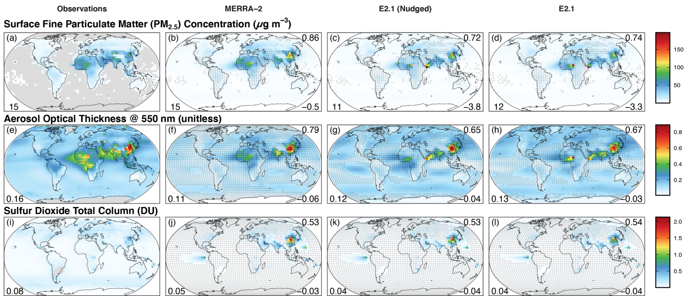
Figure 18. Annual average surface concentration of fine particulate matter (PM 2.5 ; in \mu\text{g m}^{-3} ; top row), aerosol optical thickness at 550 nm (unitless; middle row), and total column of sulfur dioxide (in Dobson Units; bottom row). The left column from top to bottom shows observations from Hammer et al. (2020), Aura MODIS, and OMI (Li et al., 2020), respectively. The right three columns show equivalent values determined from GEOS-Chem driven by MERRA-2, E2.1 nudged to MERRA-2, and free-running E2.1 meteorology. Gray dots show locations where the simulated values are statistically different from the observations with respect to interannual variability ( p -value < 0.05 ; n = 10 yr). The number in the lower left of each panel shows the global mean value. The number in each model panel’s top right shows the pattern correlation ( R ) between the simulated and observed values. The number in the lower left shows the mean bias of the model with respect to the observations.
