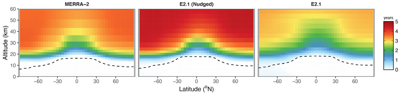
Figure 12. Average age of air in the stratosphere in GEOS-Chem simulations driven by MERRA-2, E2.1 nudged to MERRA-2, and E2.1, using the temporal lag in the simulated 2005–2014 C.E. time series of SF 6 relative to the tropical tropopause as a chronological tracer. The dashed black line shows the simulated zonal mean tropopause altitude.
