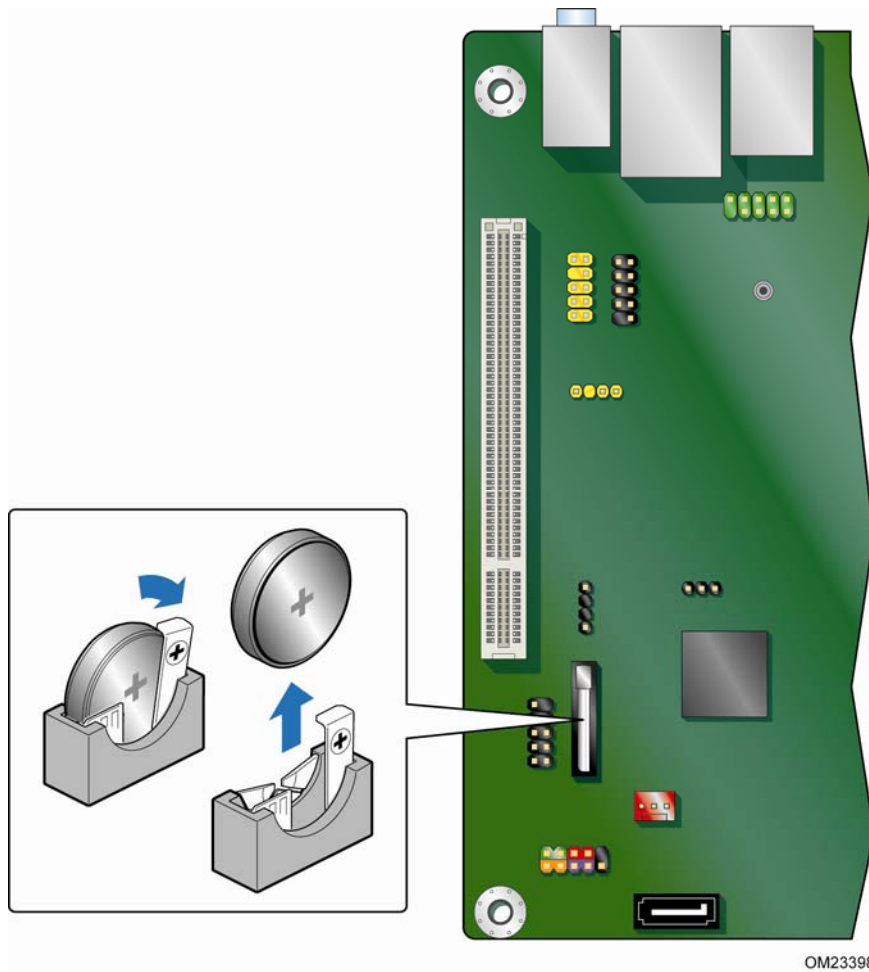
Figure 13. Removing the Battery
