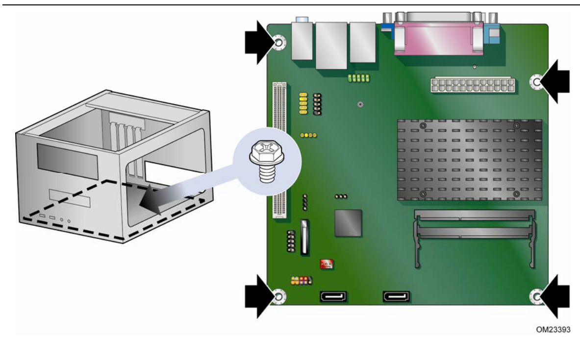
Figure 6. Intel Desktop Board D2500HN Mounting Screw Holes
