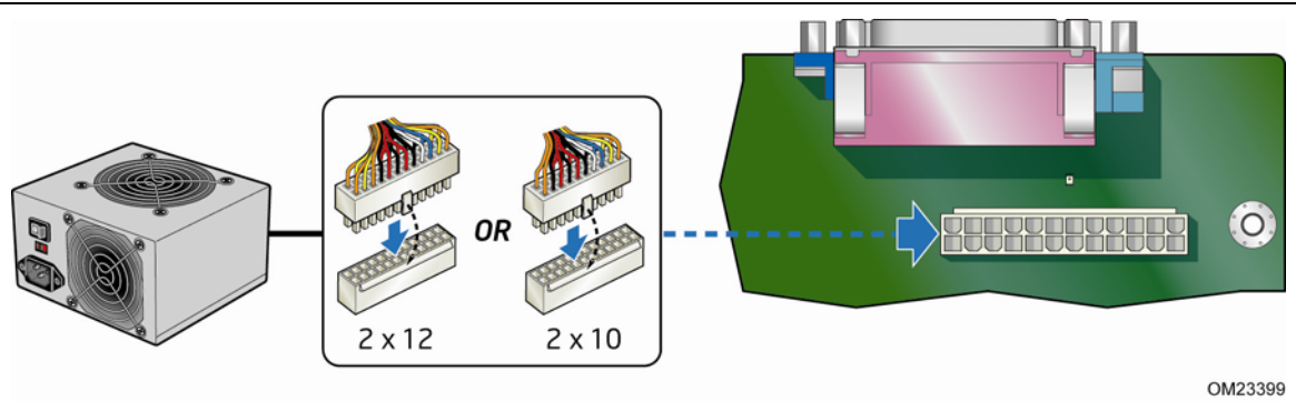
Figure 11. Connecting Power Supply Cables
