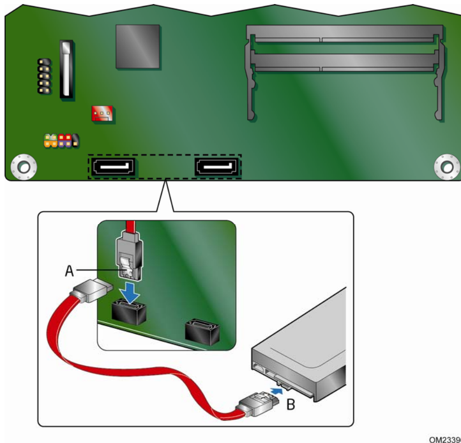
Figure 8. Connecting the Serial ATA Cable
