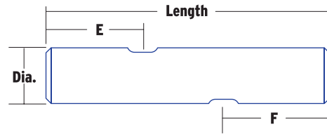
Style 2 Two Keyways
