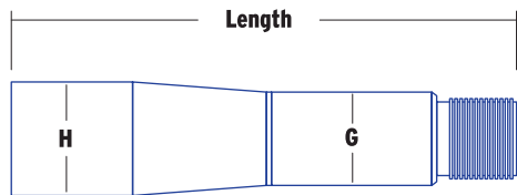
Style 5 Tapered & Threaded
