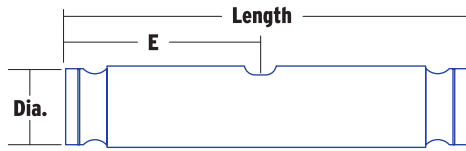
Style 3 One Keyway, Two Seal Grooves
