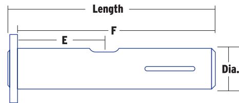
Style 6 One Keyway, One Oil Groove
