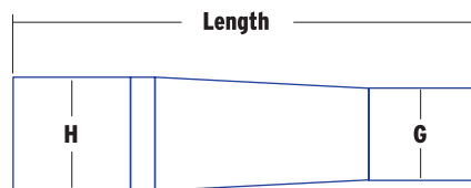
Style 6 One Keyway, One Oil Groove
