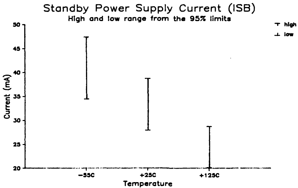
Figure 8: VCC Supply Current, ICC and ISB
