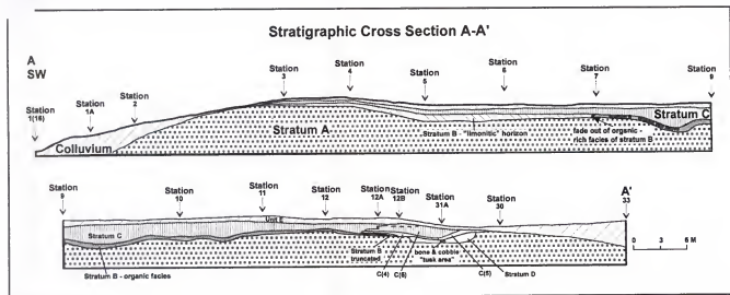
Figure 17. Stratigraphic section A-A' (by J. Albanese).
