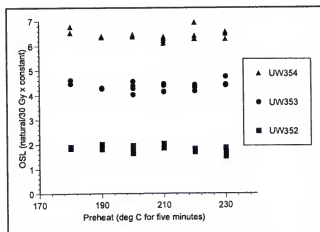
Figure 70. OSL vs. preheat temperatures.
