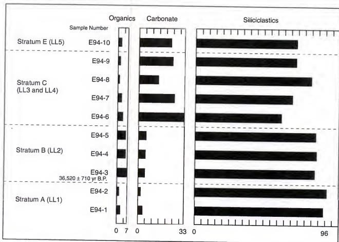
Figure 98. Results of Thermal Analysis (Loss-On-Ignition).
