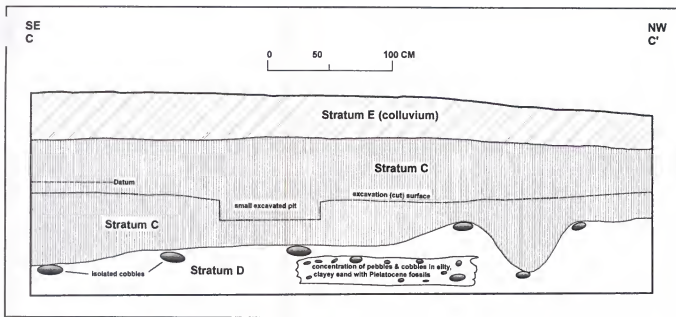
Figure 20. Stratigraphic section C-C' (by J. Albanese).
