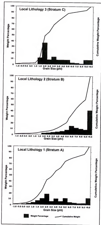
Figure 46. Grain size histograms for strata A-C.
