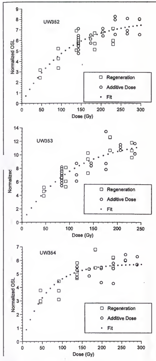
Figure 71. Normalized OSL vs. dose.
