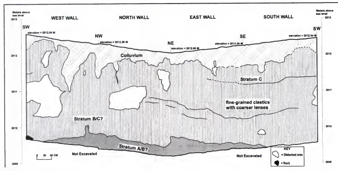
Figure 56. Generalized stratigraphy in Test Pit/Excavation Area C (near the North Block) (profile by C. L. Hill).
