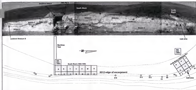
Figure 39. Map and photograph showing North and South Blocks, major strata, Merrell Locality (C. L. Hill photo and map).
