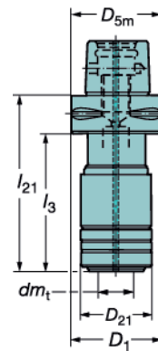
Cx-391.61
