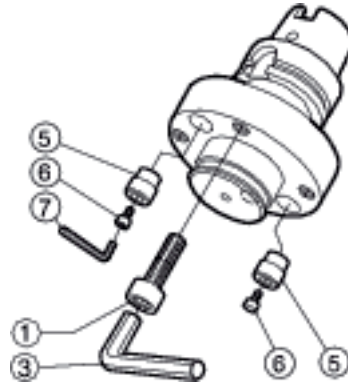
392.41005C-63 16 050 Driving ring
