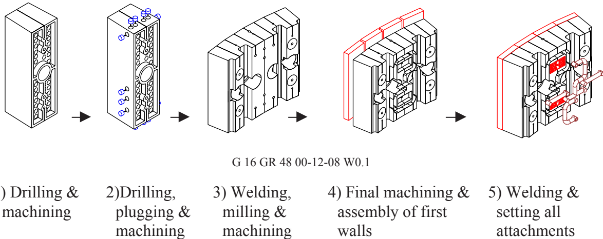
Figure 2.3.8-3 Fabrication Procedures Based on Using Solid Forged Blocks
