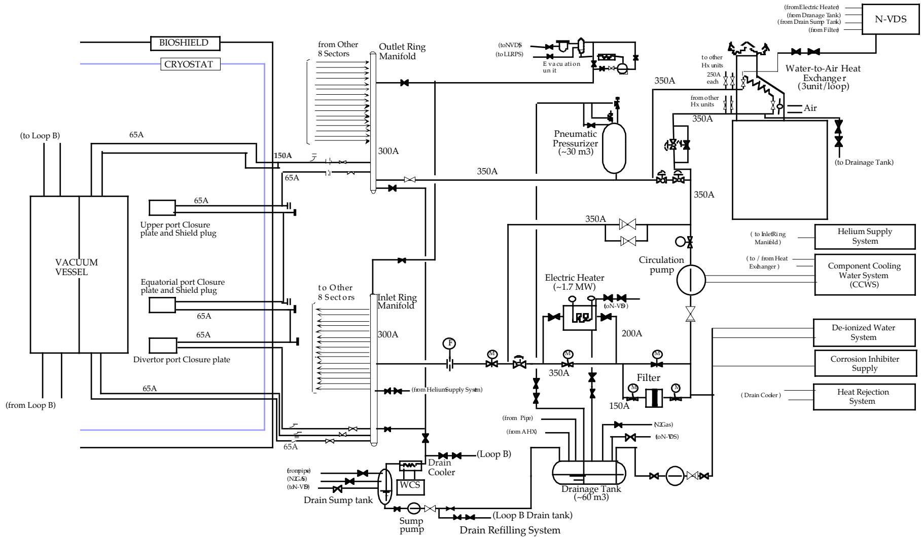
Figure 3.3.3-3 Flow Diagram of the VV PHTS
