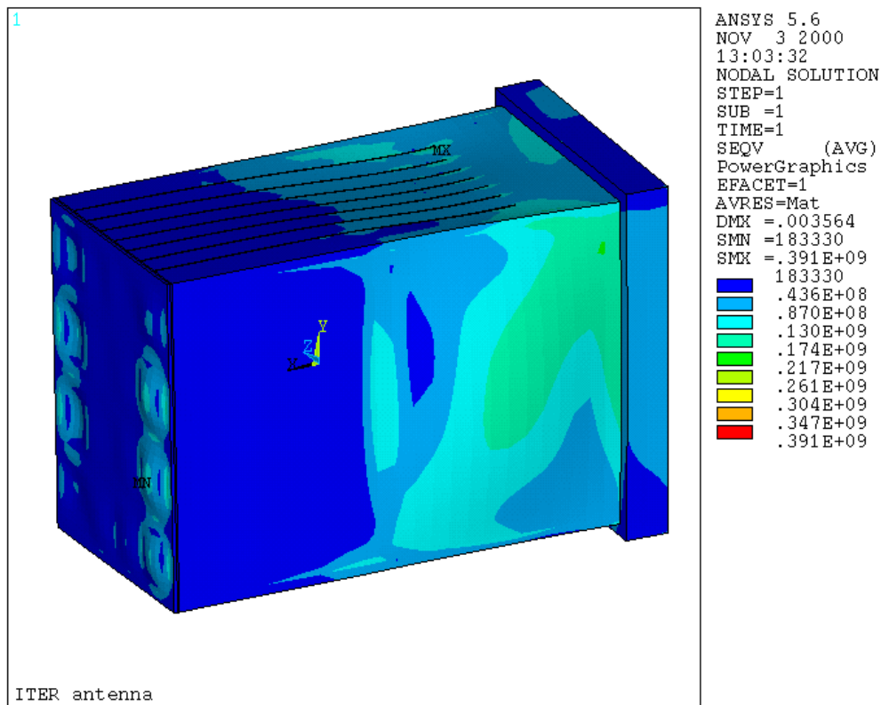
Figure 2.5.2-3(a) Example of IC Launcher von Mises Stress and Strain Map
