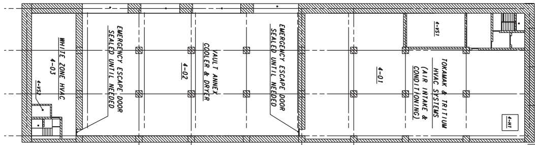
TRITIUM BUILDING PLAN VIEW AT ELEV. : +21.000
