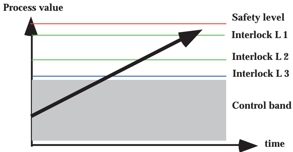
Figure 3.7.2-3 Interlock Level Set Point
