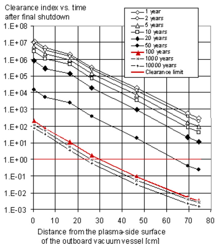
Figure 5.4.3-4 Profile Across the Outboard Vacuum Vessel Wall of the Total Clearance Index in the Structural and Shielding Steels for Various Decay Times After Final Shutdown
