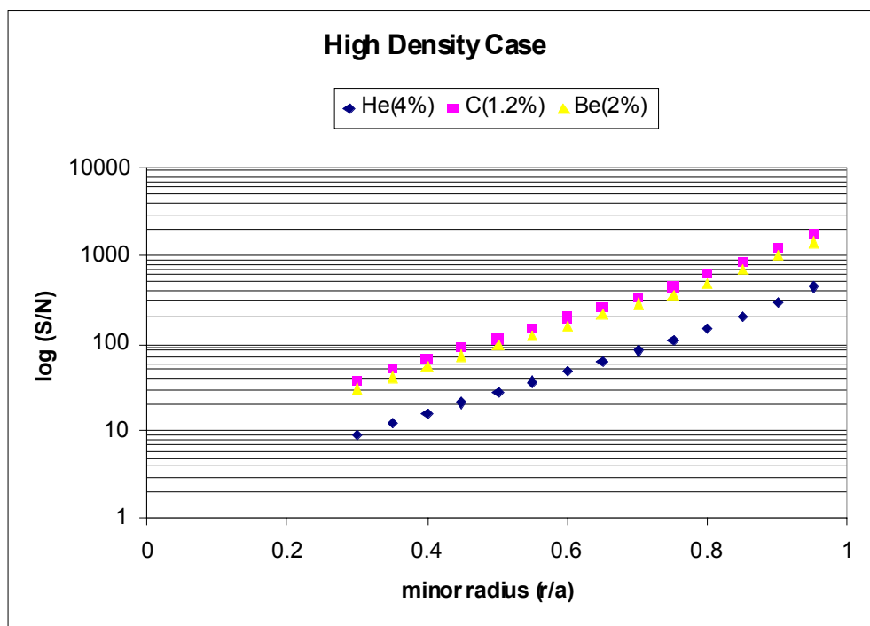
Figure 2.6-10 Signal-to-Noise Ratio at Spectral Half Maximum for the Measurement of 4% Helium, 1.2% C and 2% Be respectively versus Minor Radius for Standard ELMy H-mode Plasma Conditions
