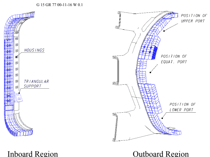
Figure 2.2-6 Layout of Shields
