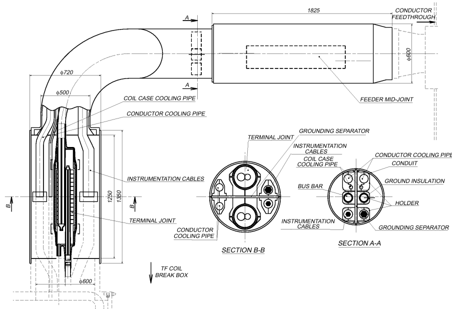
Figure 2.1.8-2 Typical Terminal Joint and Feeder Cross Section
