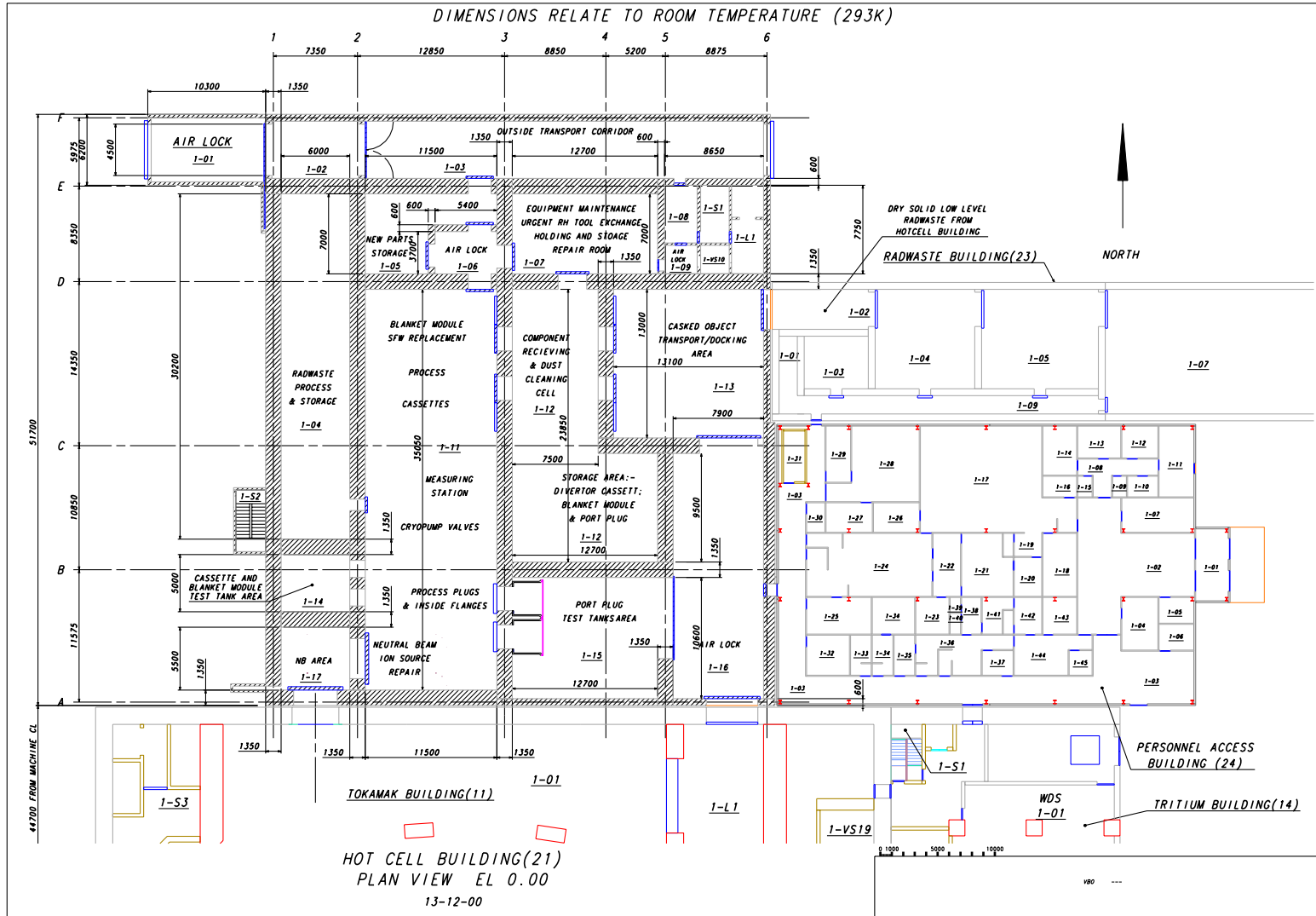
Figure 3.6.5-1 Hot Cell, Low Level Radwaste, and Personnel Access Control Buildings (plan view at grade level)
