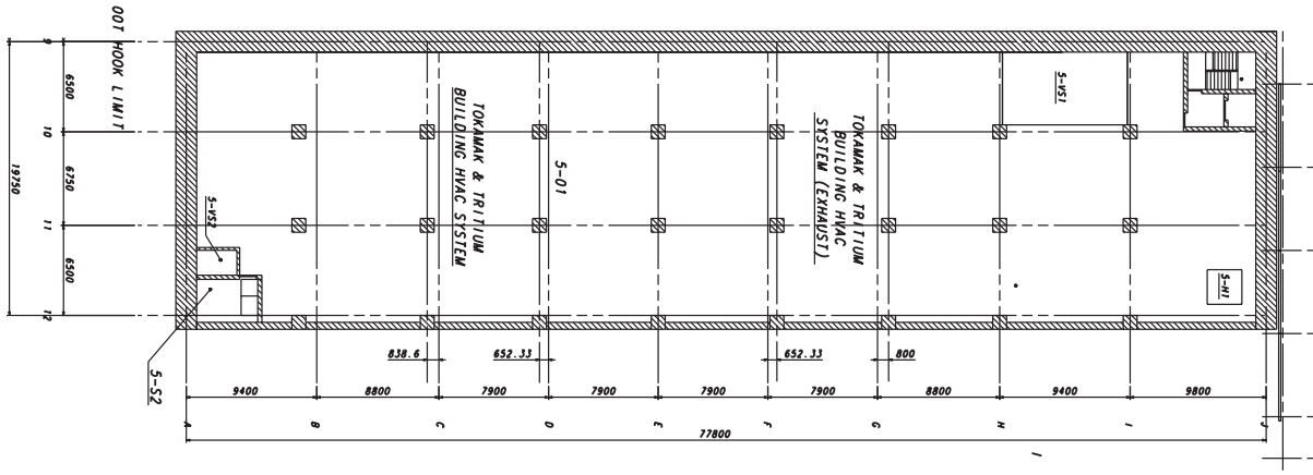
TRITIUM BUILDING PLAN VIEW AT ELEV. : +27.000
