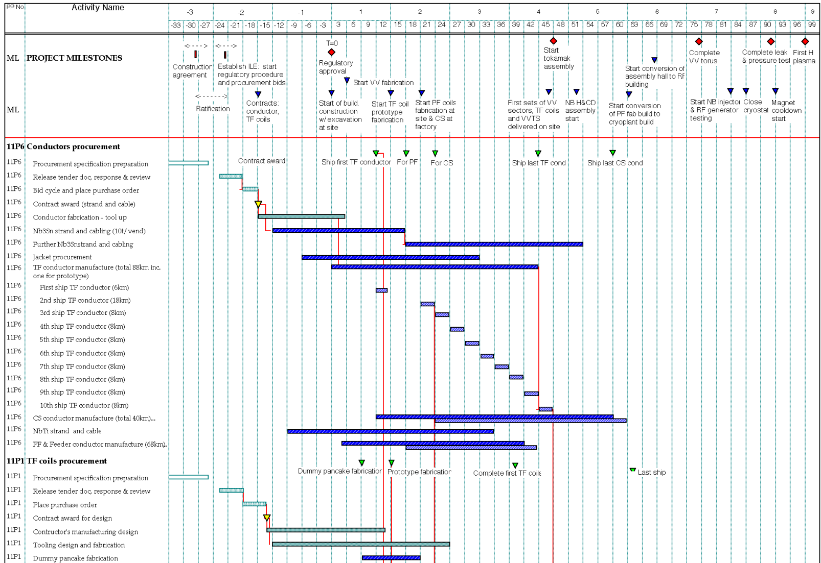
Figure 6.1.4-1 TF Coils and Vacuum Vessel Procurements to meet Assembly (1)
