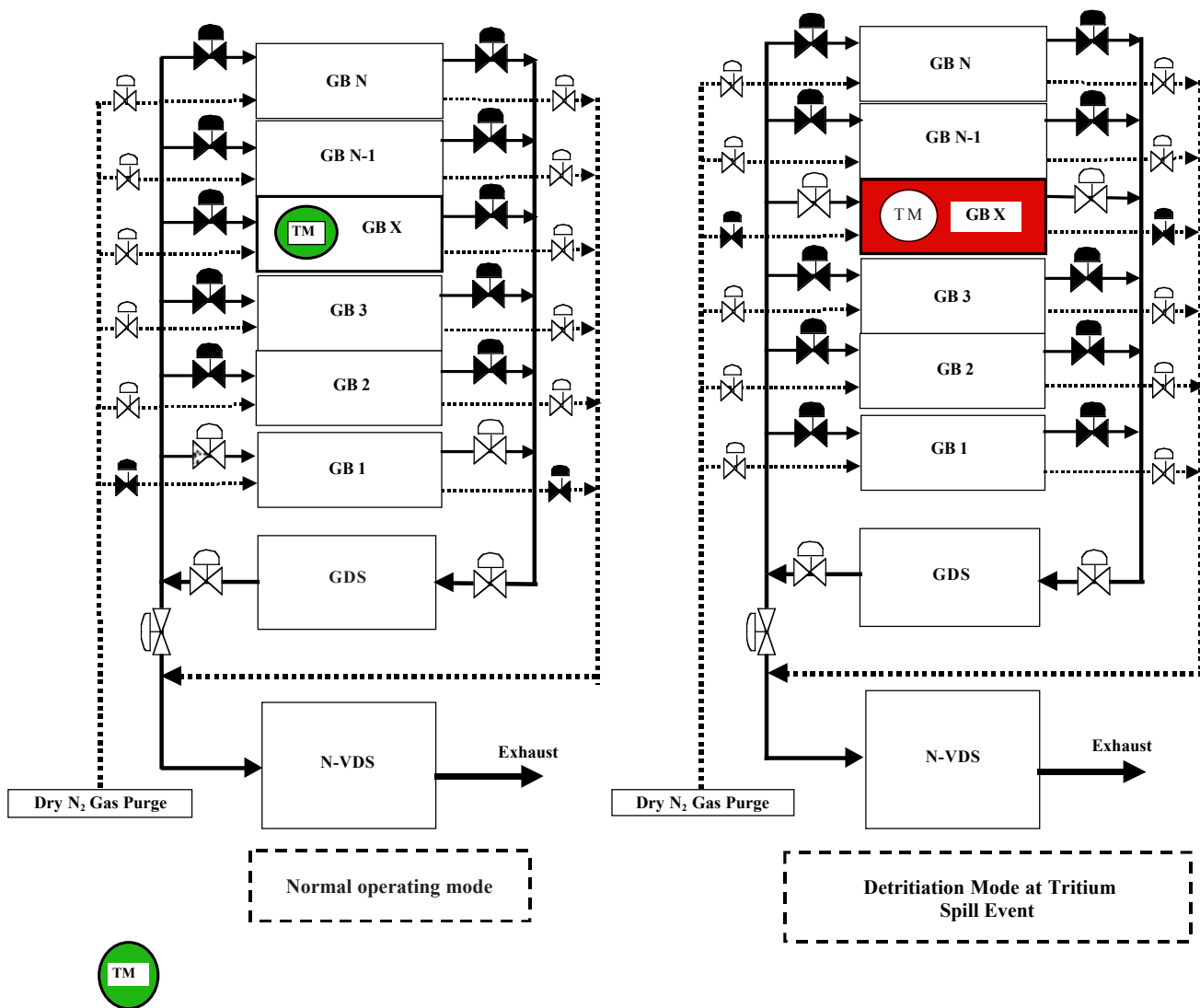
Figure 3.1-6 Integral System Configuration of the Glove Box Atmosphere Detritiation System, Glove Boxes and the Normal Vent Detritiation System
