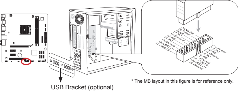
USB Bracket (optional)
