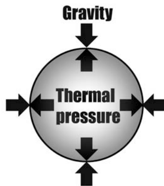
Gravity and thermal pressure remain in balance for most of a star's life.
