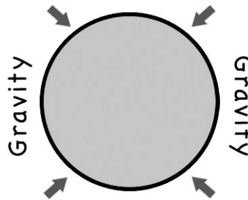
The lack of fusion energy inside the star to balance the gravity causes the final collapse of the star.
