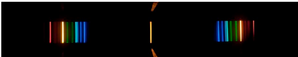
These nice orderly lines represent a fully aligned spectroscope. If this is what you are seeing through yours, you can tape the slit end in place.
