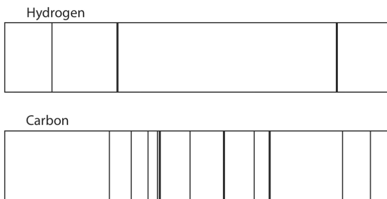
The spectra of hydrogen and carbon, illustrating how different two different elemental spectra can be.
