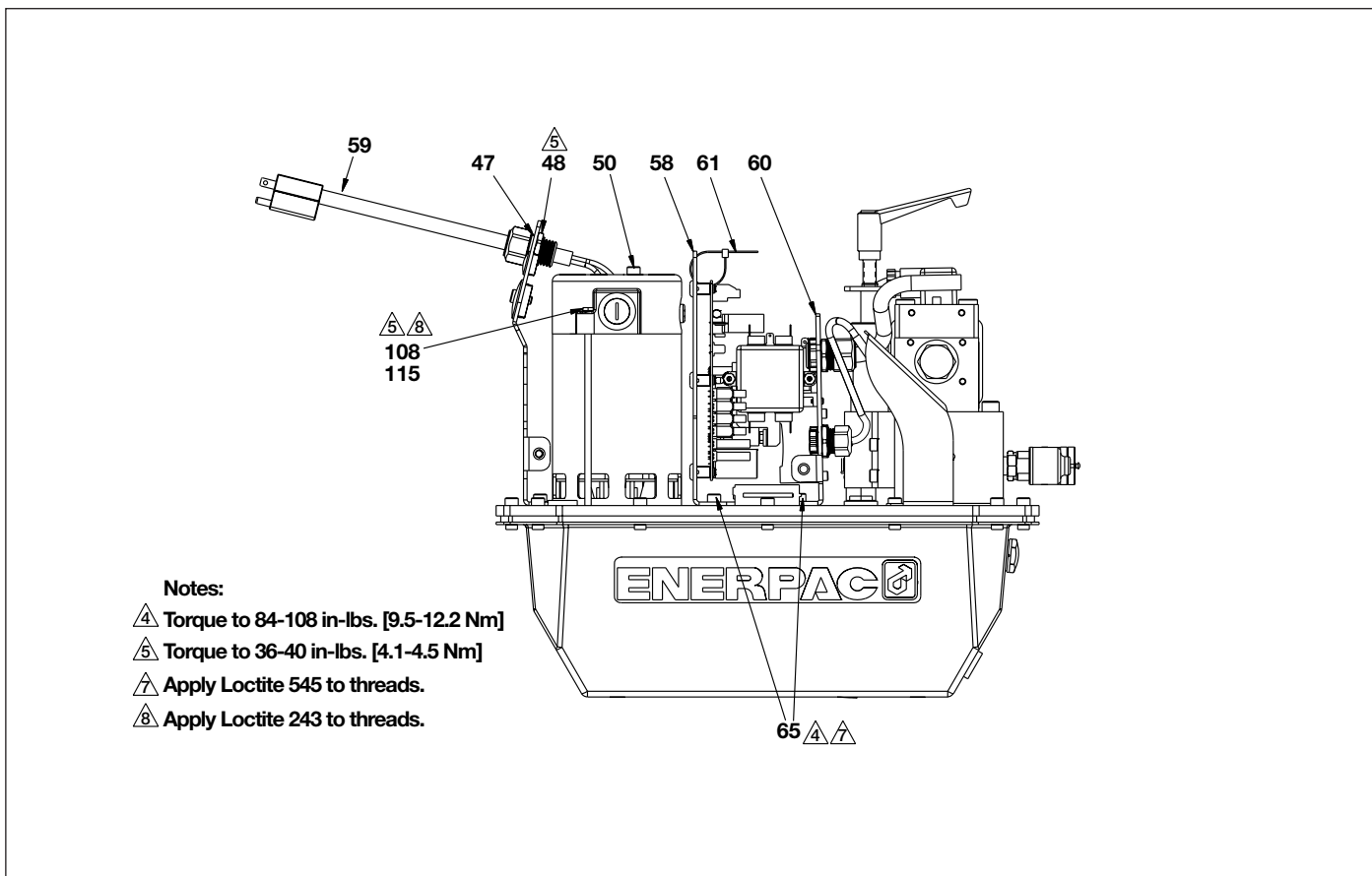
Figure 2B, Pump Assembly (side view)
