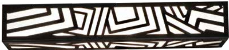
WF-STCUS-LCM-927M-MBK ADA Wall Fixture – Finish: Matte Black Material: Laser Cut Steel/Opal Acrylic Length: 24" Width: 4" Depth: 2 1/2" Canopy: 24" L x 4" W Shade: (4" x 2 1/2") x (4" x 2 1/2") x 24" H LED: Available in 3000K, 3500K and 4000K
