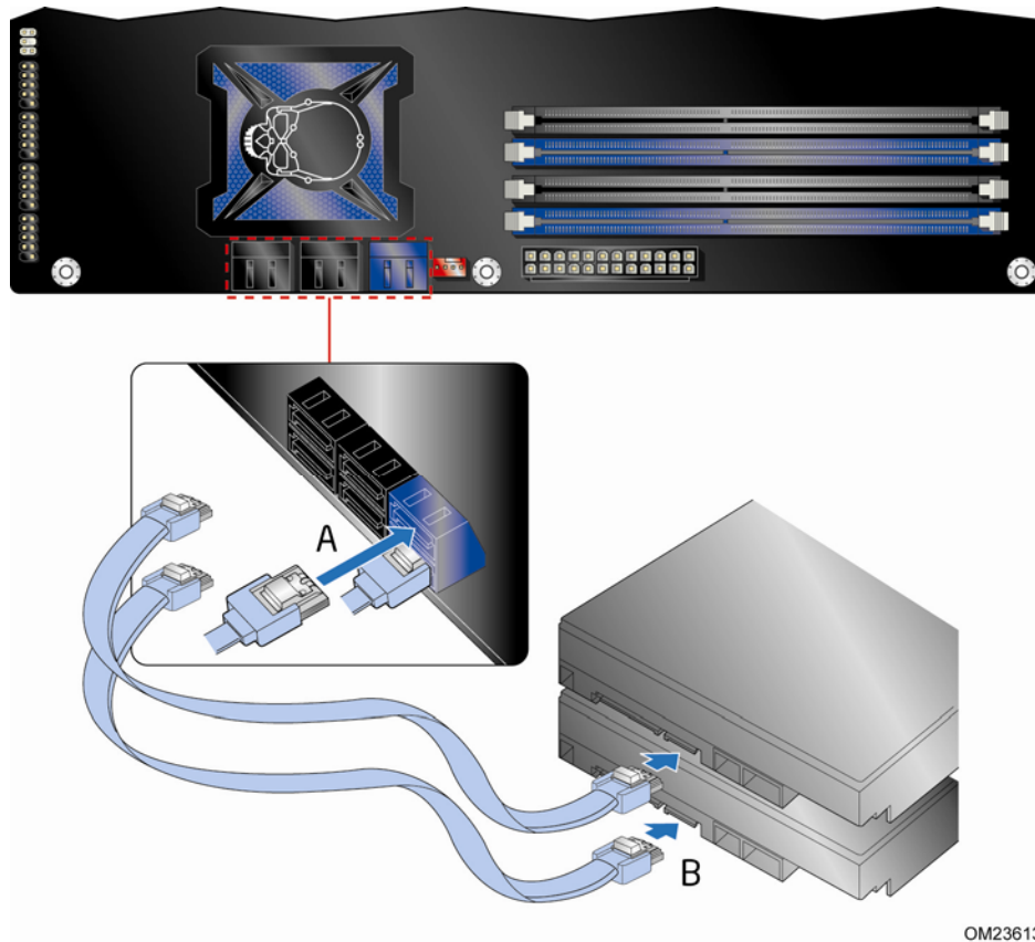
Figure 19. Connecting the Serial ATA Cables
