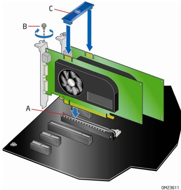
Figure 18. Installing Linked PCI Express Graphics Cards
