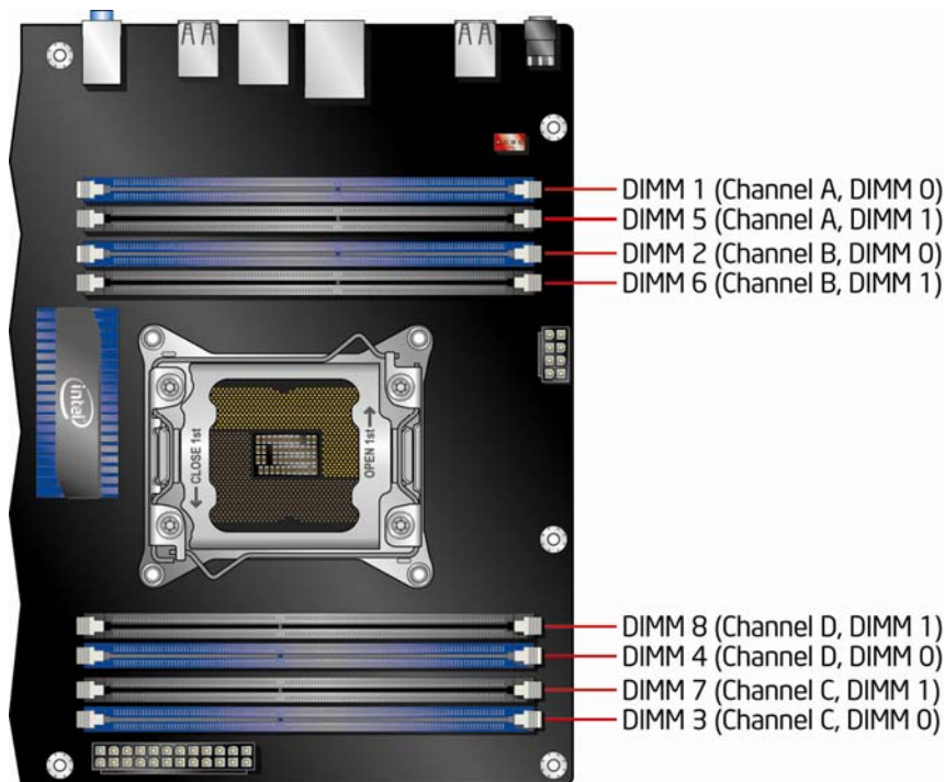
Figure 2. Memory Channel and DIMM Configuration
