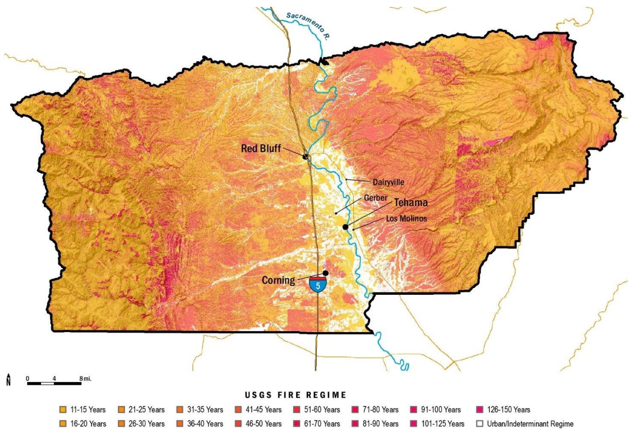
Figure 4-44: USGS Fire Regime Map for Tehama County
