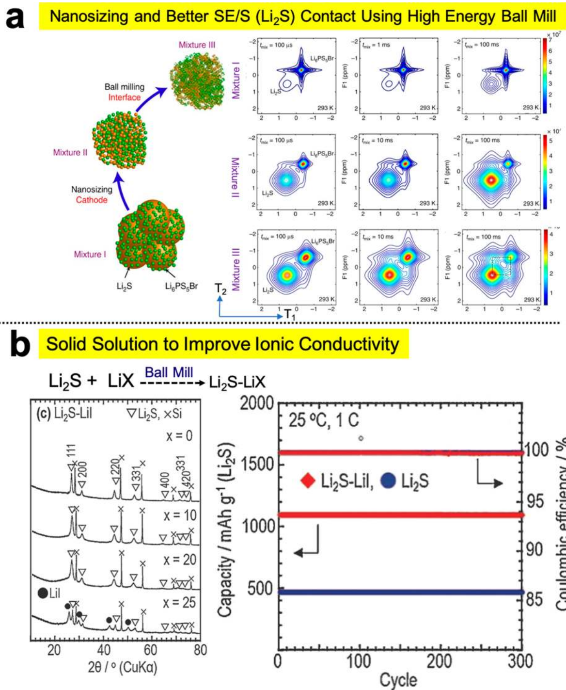
Figure 22. (a) \text{Li}_2\text{S} – \text{Li}_6\text{PS}_5\text{Br} composites were made by high-energy ball milling. Solid-state two-dimensional (2D) ^7\text{Li} – ^7\text{Li} exchange spectra (2D-EXSY) measured at a ^7\text{Li} resonance frequency of 155.506 MHz with a spinning speed of 20 kHz for short (100 \mu\text{s} ) to long mixing times (100 ms) at RT for different mixtures. Off-diagonal cross-peak intensity was observed only for mixtures III at t_{\text{mix}} = 10 ms, was most pronounced at t_{\text{mix}} = 100 ms, and represents Li-ion exchange from \text{Li}_2\text{S} to \text{Li}_6\text{PS}_5\text{Br} and vice versa. 171 (b) Ball-milling synthesis of a \text{Li}_2\text{S} – \text{LiI} solid solution and an all-solid-state Li–S battery operating at 25 ^\circ\text{C} with this \text{Li}_2\text{S} – \text{LiI} solid solution. Reproduced with permission from ref 174. Copyright 2015 Wiley-VCH Verlag.
