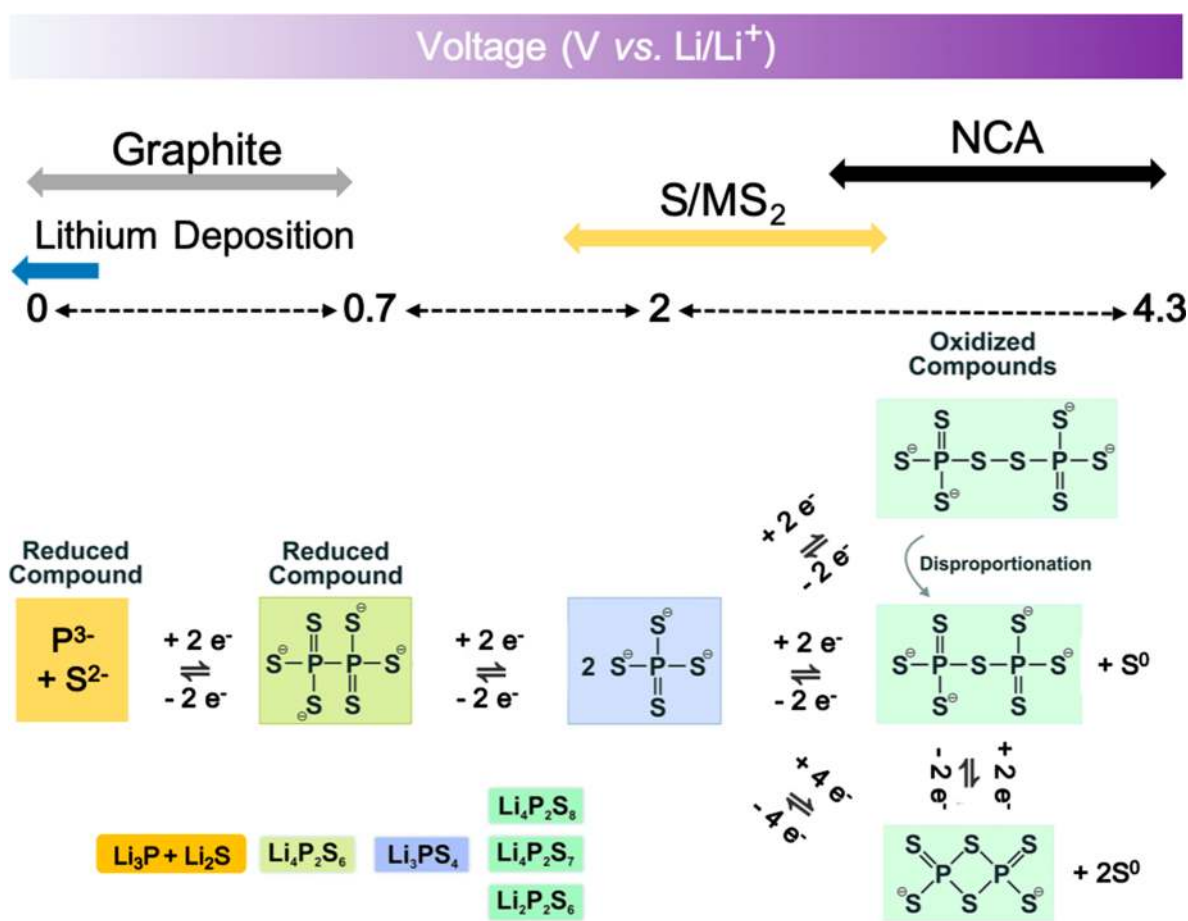
Figure 4. Possible interfacial reactions of sulfide SEs at a wide range of operating voltages. Top: The arrows correspond to the voltage ranges when using graphite, Li metal deposition, layered oxide cathode (NCA), Li–S, or metal sulfide. Bottom: The possible redox reactions at the corresponding voltage windows to illustrate the possible oxidation or reduction species. Reproduced with permission from ref 45. Copyright 2017 American Chemical Society.
