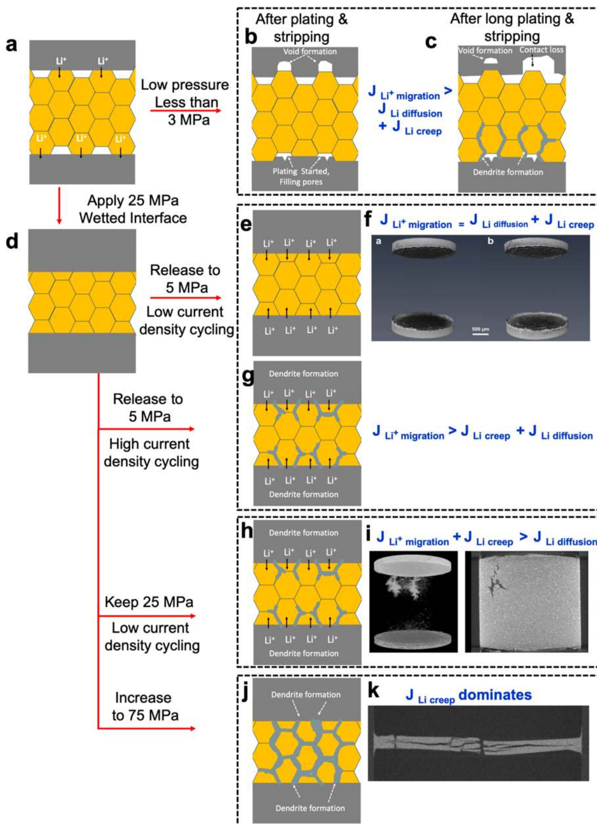
Figure 32. (a) Schematic of Li metal placed on both sides of a SE pellet. Many gaps are present if the applied pressure is < 3\text{ MPa} . (b) Li plating and stripping at < 3\text{ MPa} where significant void formation occurs on the stripping side (top right) and Li deposition on the plating side (bottom) fills the pores. (c) Isolated void formation and contact losses occur on the stripping side whereas selective area Li metal deposition (promoting dendrite growth) at the plating side over prolonged plating and stripping. (d) The interface is mechanically wetted with 25 MPa. (e) Afterward, if a 5 MPa stack pressure is used, uniform plating and stripping occurs at 0.075\text{ mA/cm}^2 (a low current) without any Li metal dendrite growth. (f) Verification with Nano-CT where no cracks were found between two plungers (Li metal is not visible by Nano-CT). (g) Even at a low stack pressure of 5 MPa, dendrite growth takes place if the current density is more than 0.1\text{ mA/cm}^2 . (h) If a 25 MPa stack pressure is kept, further dendrite growth takes place at a low current density of 0.075\text{ mA/cm}^2 . (i) Cracks were found in Nano-CT, which are caused by Li metal dendrite growth. (j) High stack pressure of 75 MPa
