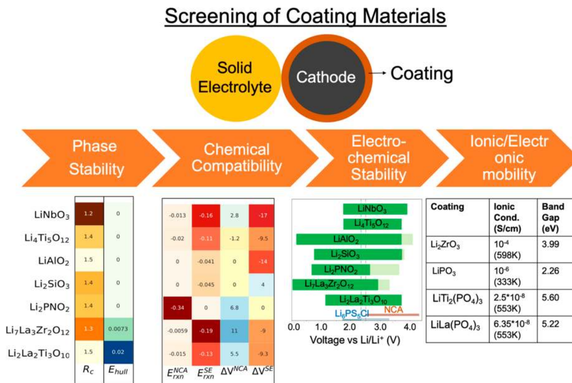
Figure 17. Necessary criteria for an effective cathode coating for ASSBs. Reproduced with permission from ref 51. Copyright 2019 American Chemical Society.
