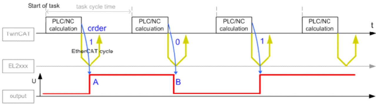
Fig. 16: Output of output channel information, standard
