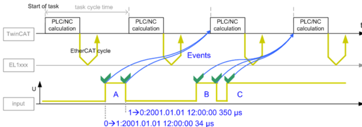
Fig. 19: Query of input channel information, with multi-timestamp
