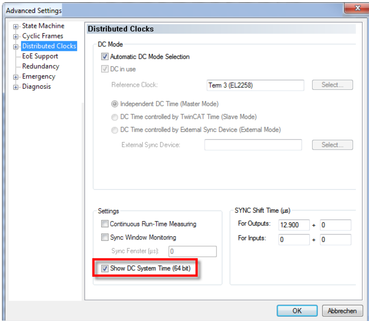
Fig. 173: Activation of the master distributed clock display
