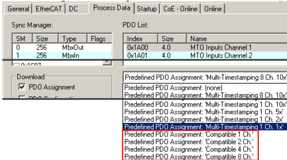
Fig. 172: Predefined PDOs for compatibility mode
