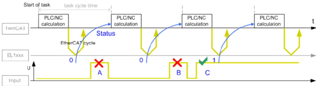
Fig. 13: Query of input channel information, standard
