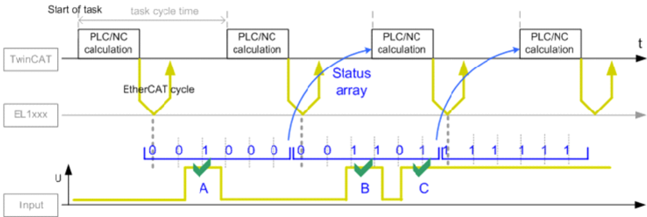
Fig. 14: Query of input channel information, oversampling
