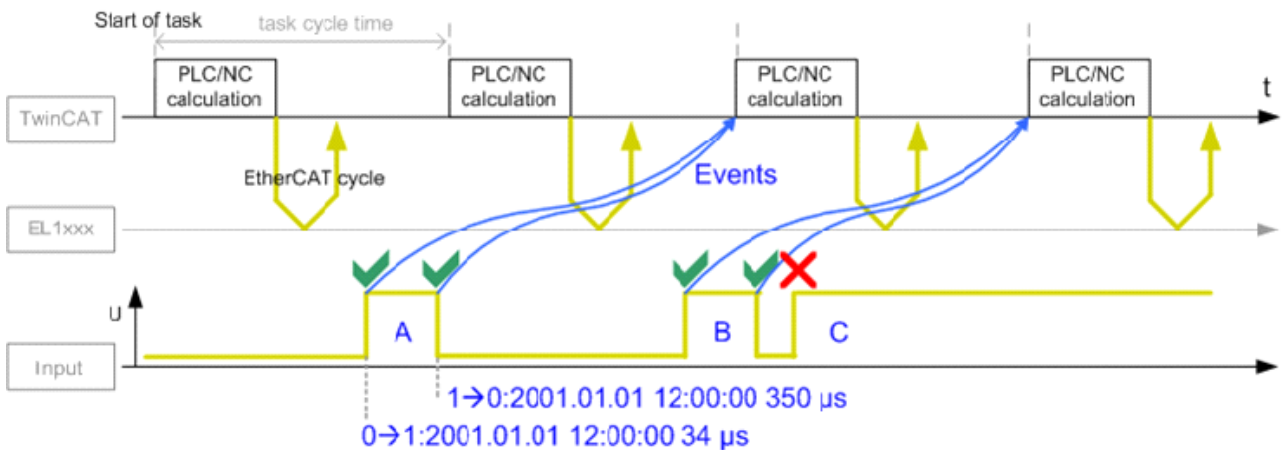
Fig. 15: Query of input channel information, with timestamp
