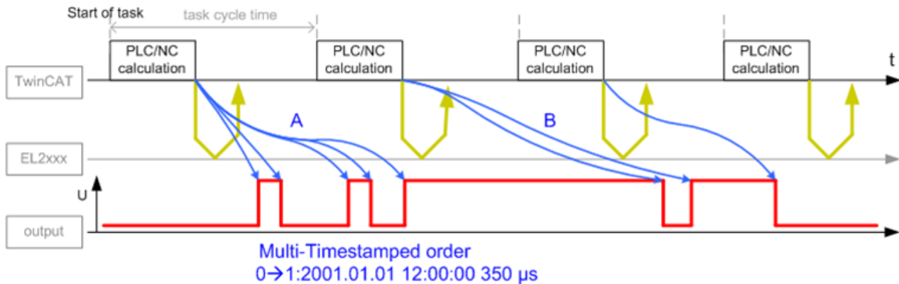
Fig. 20: Output of output channel information, with multi-timestamp
