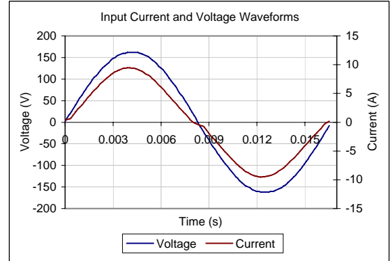
Input AC Current Waveform (ITHD = 14.2%, 50% Load)
