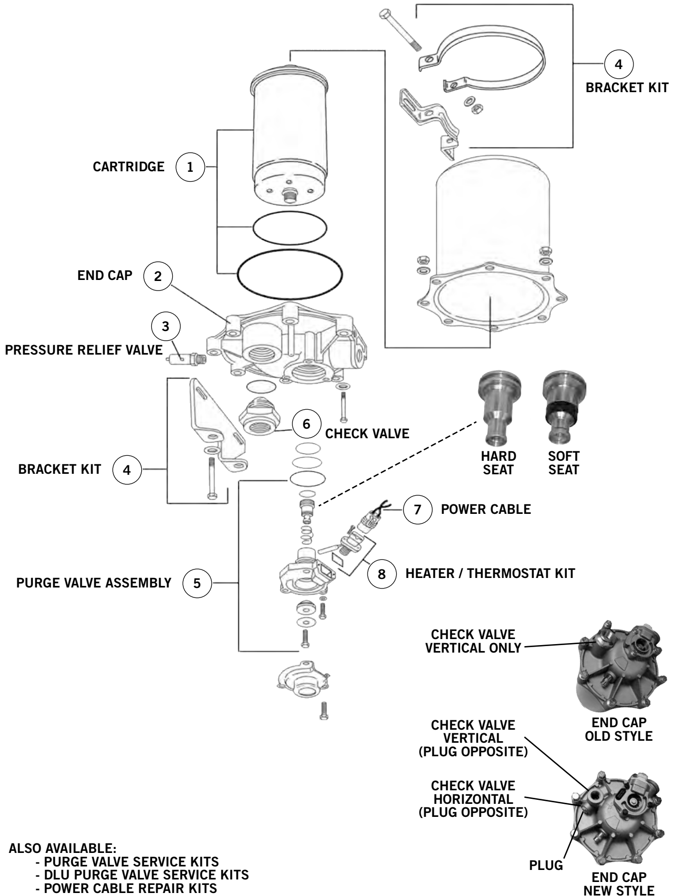
Figure 4-3. AD9 Air Dryer
