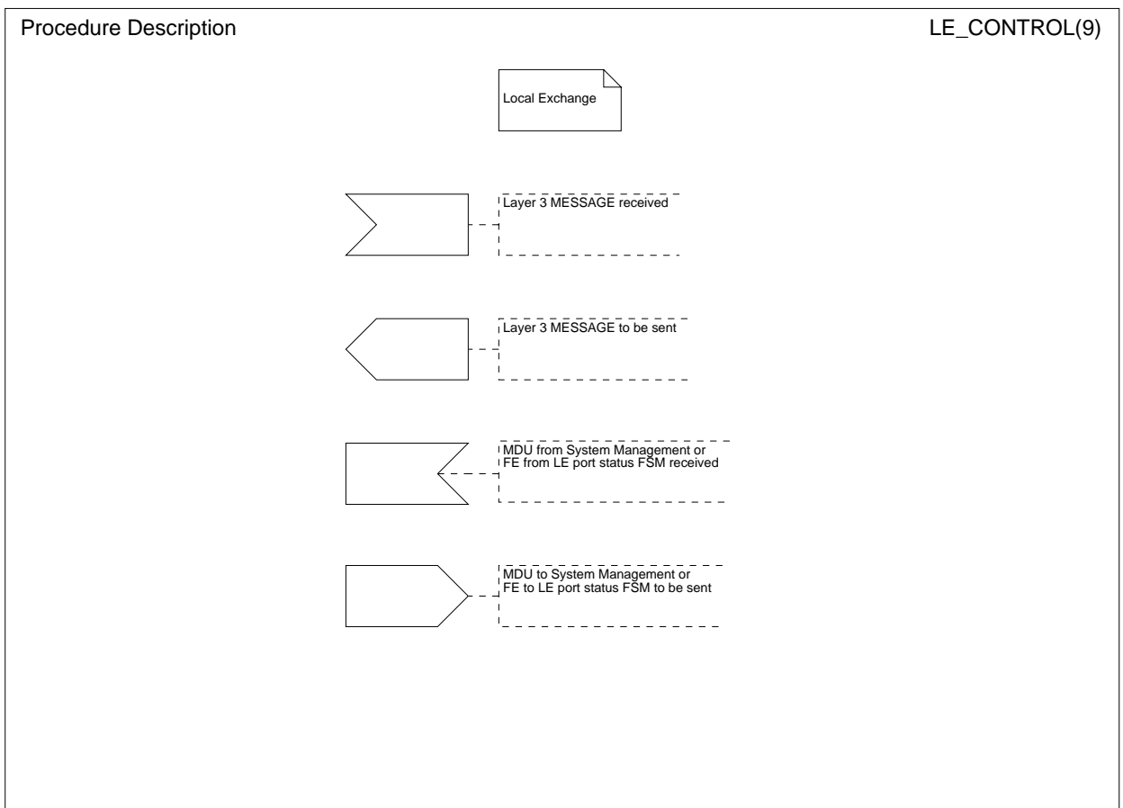
Figure L.26: Input and output symbols application - control protocol (LE-side)
