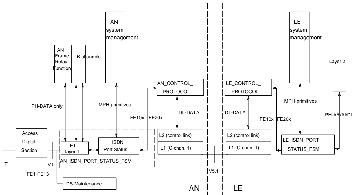
Figure N.1: Protocol architecture for ISDN basic access port control functions
