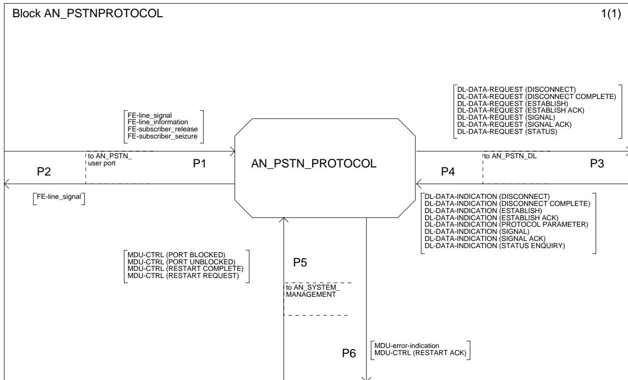
Figure L.2: PSTN protocol block description AN-side
