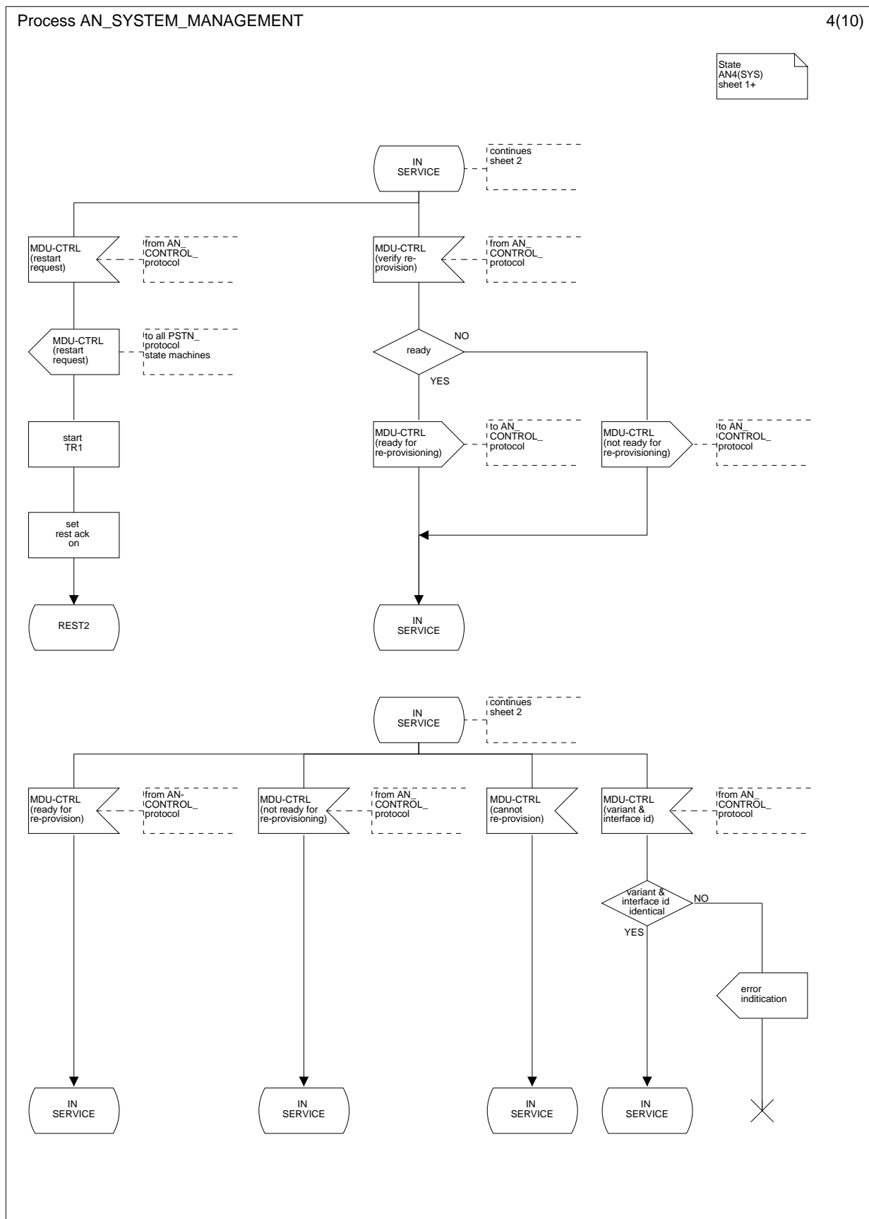
Figure L.17.4: System management AN-side; state IN SERVICE (AN4(SYS)) (sheet 1 of 3)
