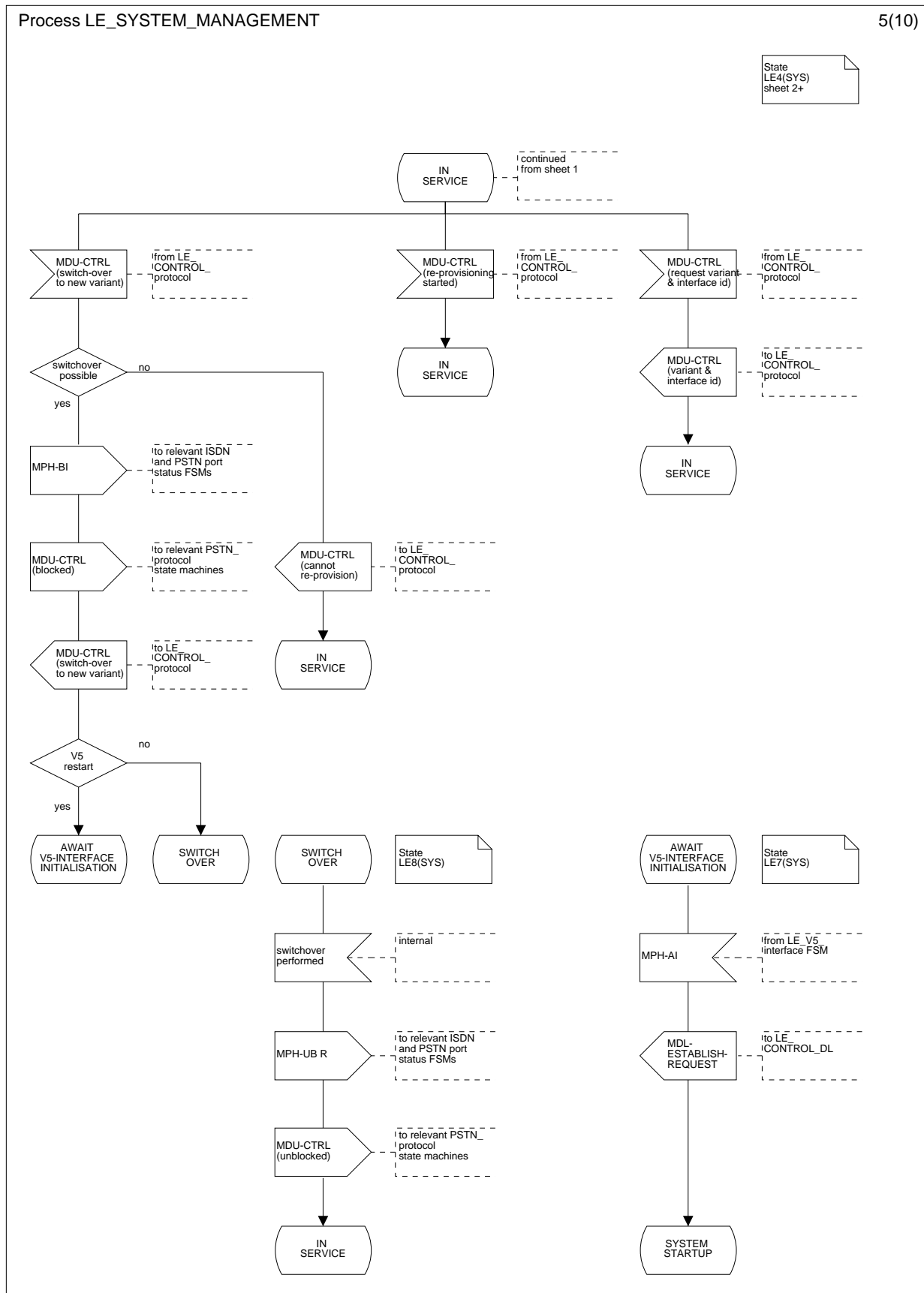
Figure L.33.5: System management LE-side; states IN SERVICE (LE4(SYS)) (sheet 2), AWAIT V5-INTERFACE INITIALISATION (LE7(SYS)) and SWITCH OVER (LE8(SYS))
