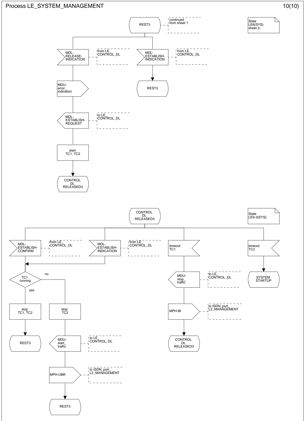
Figure L.33.10: System management LE-side; states CONTROL DL RELEASED3 (LE9-3(SYS)) and REST3 (LE6(SYS)) (sheet 2)
