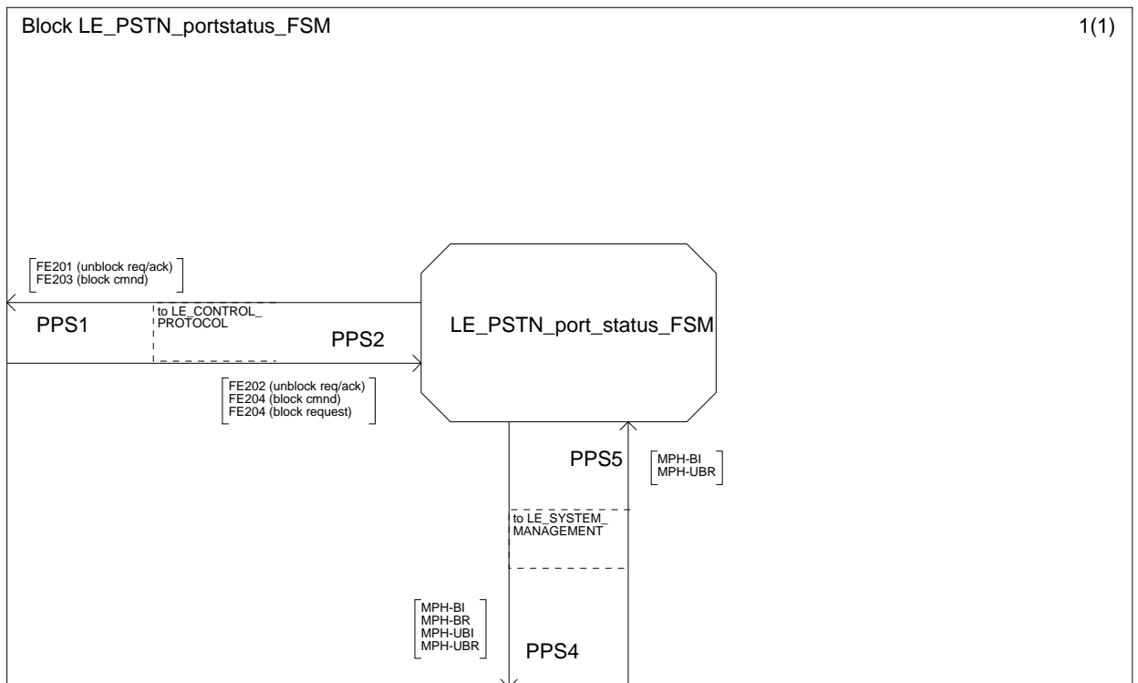
Figure L.22: PSTN port status FSM block description LE-side
