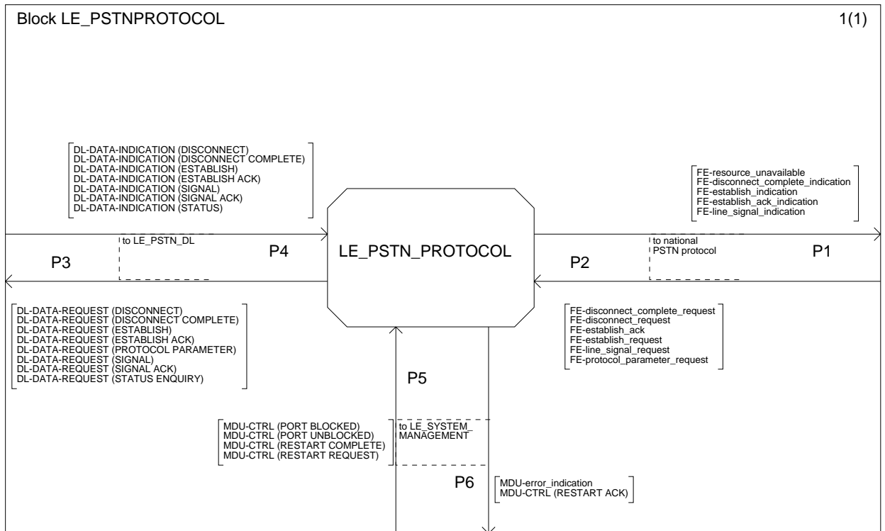
Figure L.19: PSTN protocol block description LE-side
