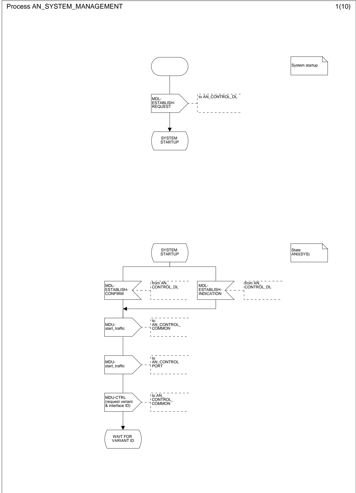
Figure L.17.1: System management AN-side; system startup and state OUT OF SERVICE (AN0(SYS))
