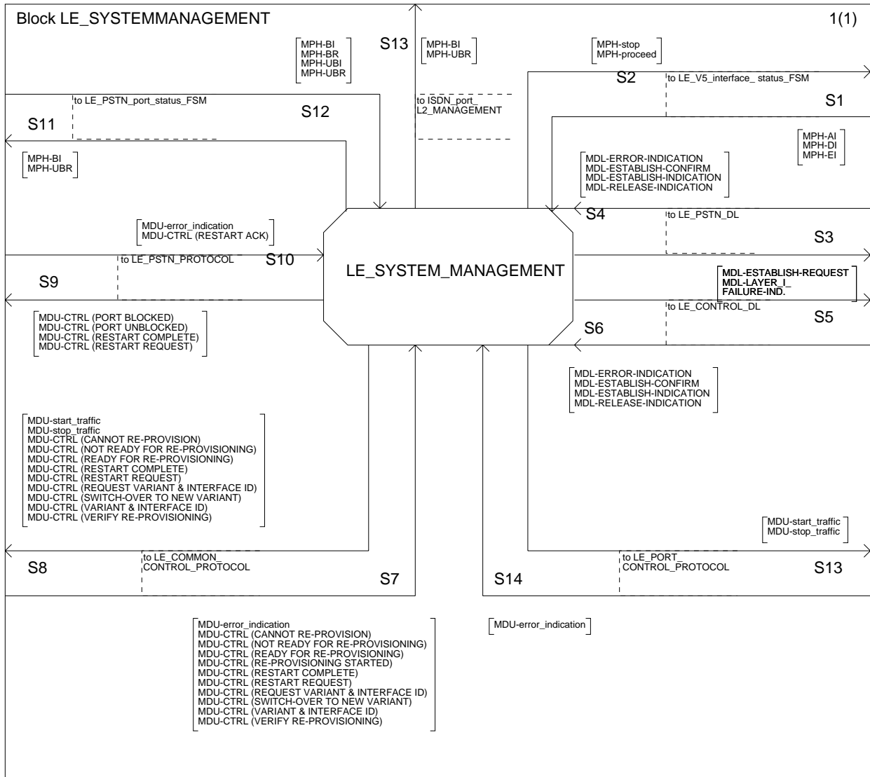
Figure L.23: System management block description LE-side
