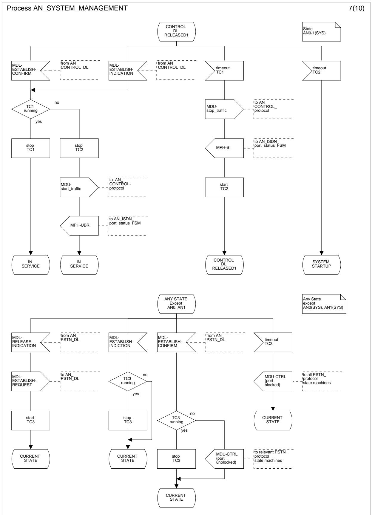
Figure L.17.7: System management AN-side; state CONTROL DL RELEASED1 (AN9-1(SYS)) and any state except AN0(SYS) and AN1(SYS)
