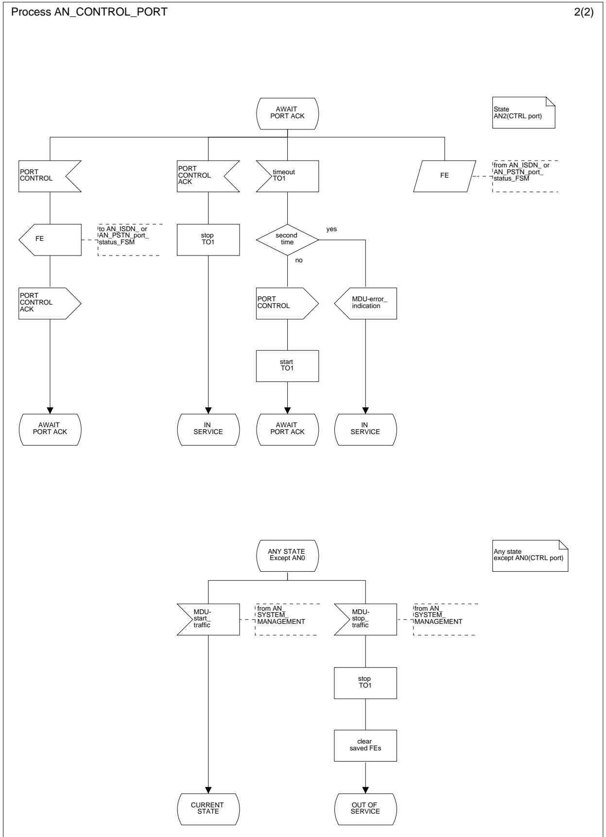
Figure L.11.2: Port control protocol AN-side; state AWAIT PORT ACK (AN2(CTRL port)) and any state except AN0(CTRL port)
