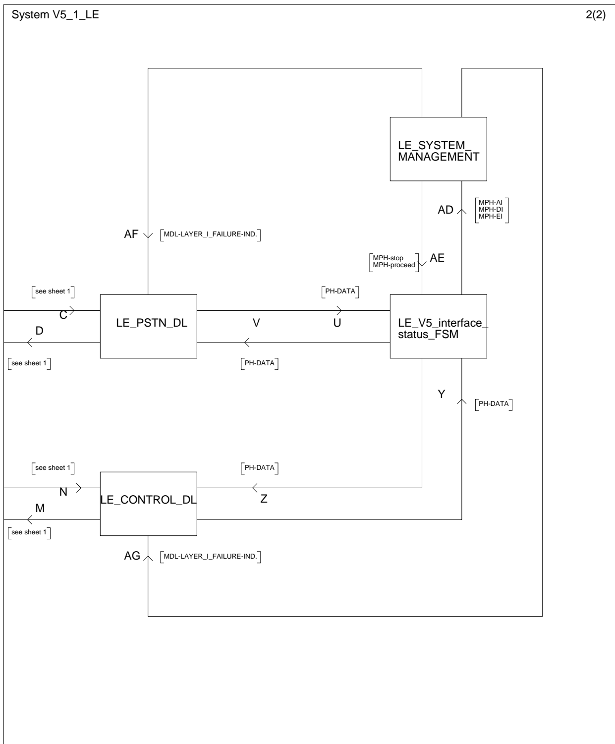
Figure L.18.2: V5.1 system overview LE-side (sheet 2)
