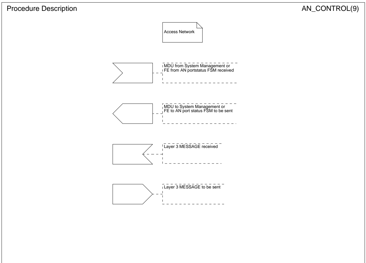
Figure L.10: Input and output symbols application - control protocol (AN-side)
