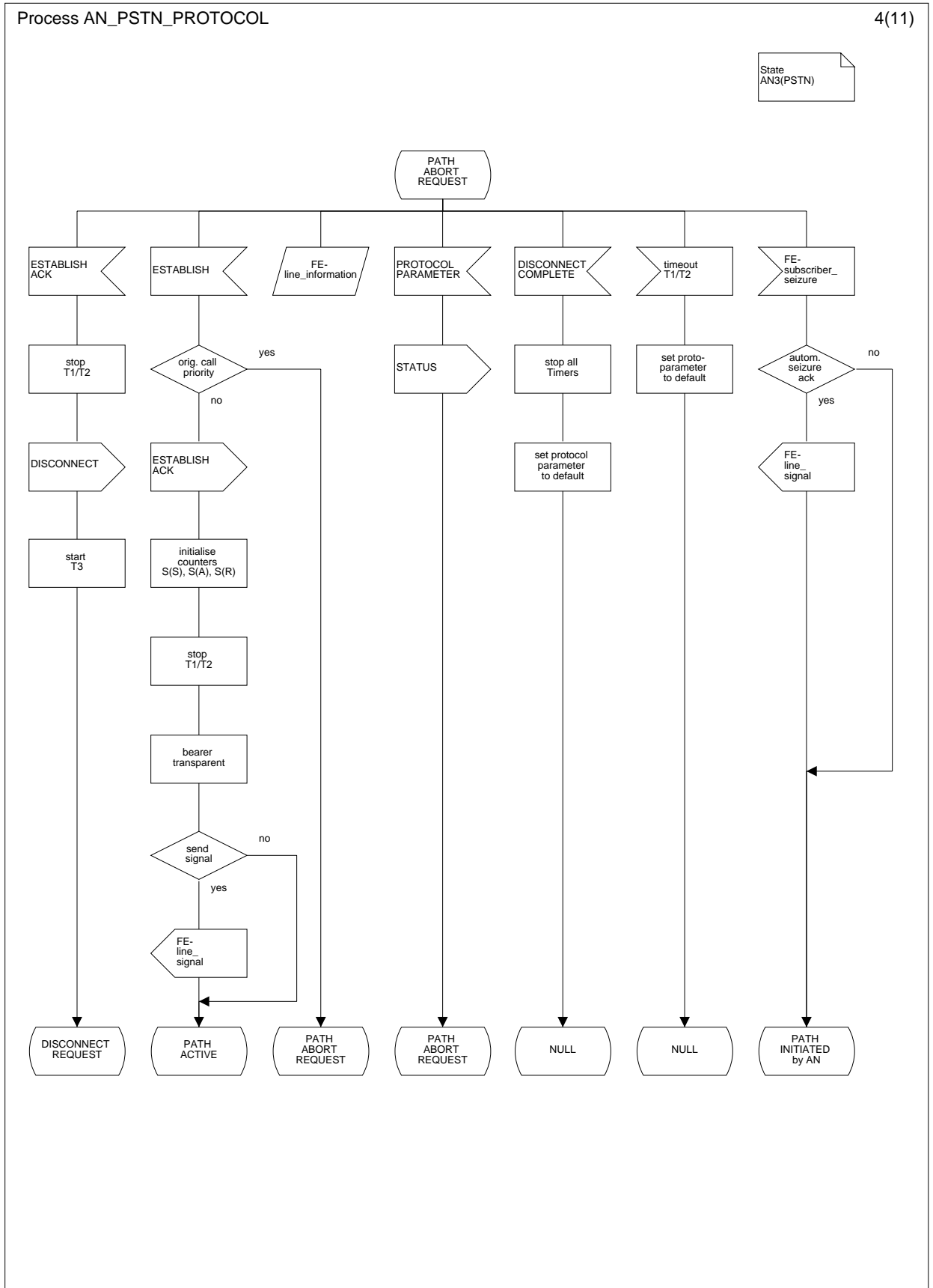
Figure L.9.4: PSTN protocol AN-side; state PATH ABORT REQUEST (AN3(PSTN))
