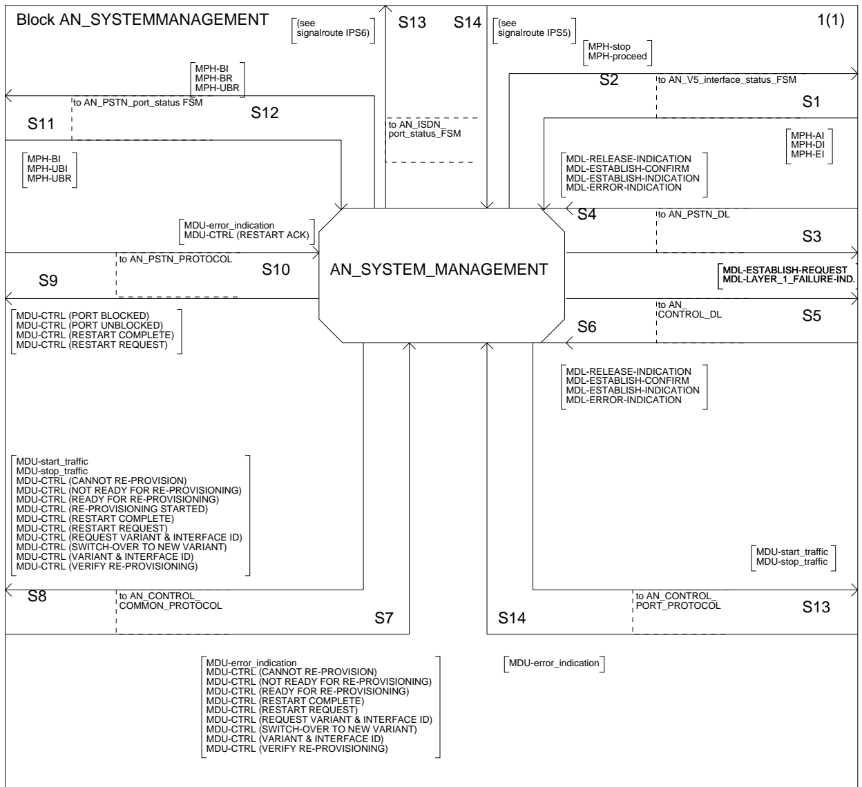
Figure L.6: System management block description AN-side
