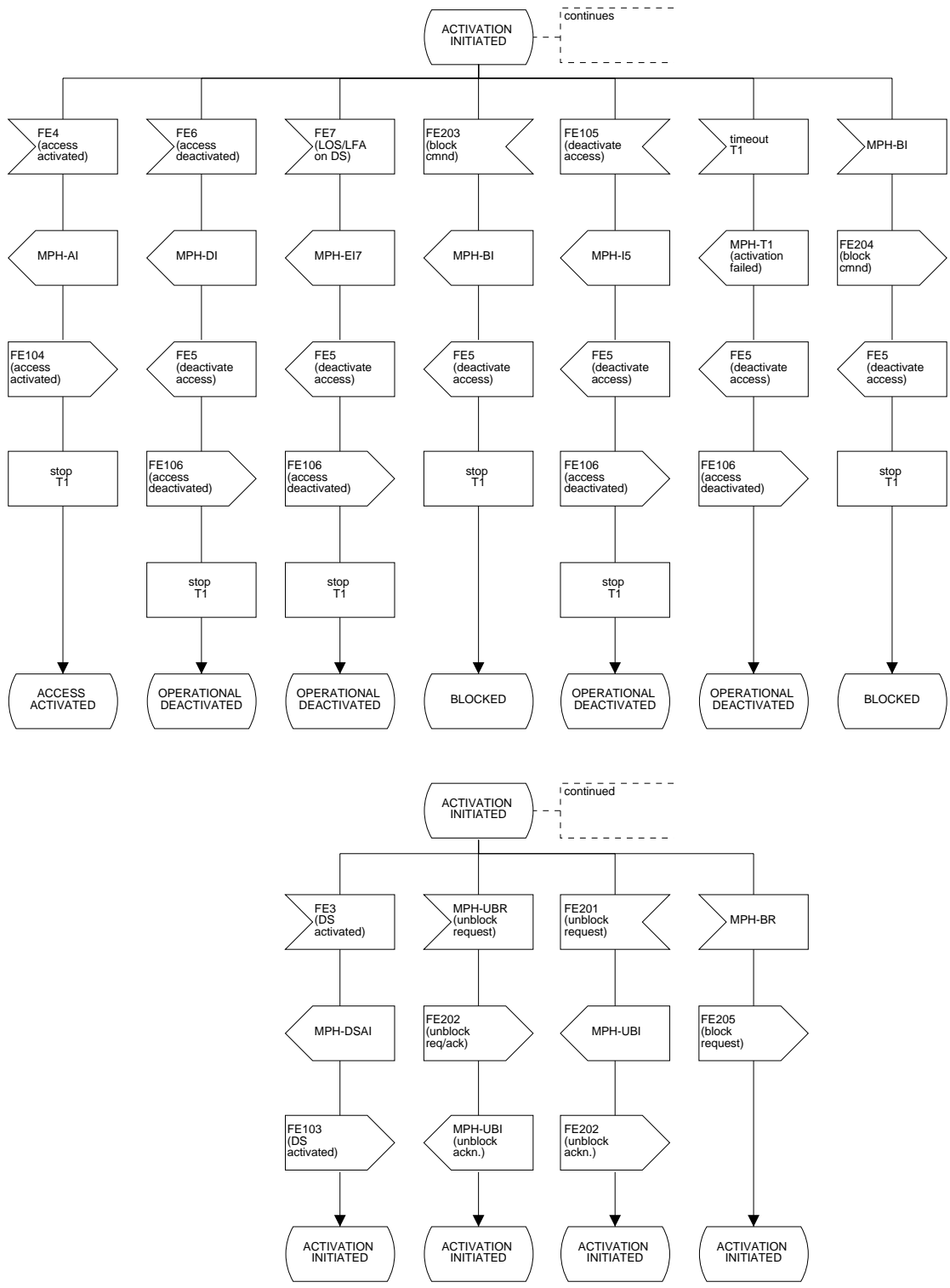
Figure L.14.5: ISDN port status FSM control AN-side; state ACTIVATION INITIATED (AN2.1 (ISDN port))
