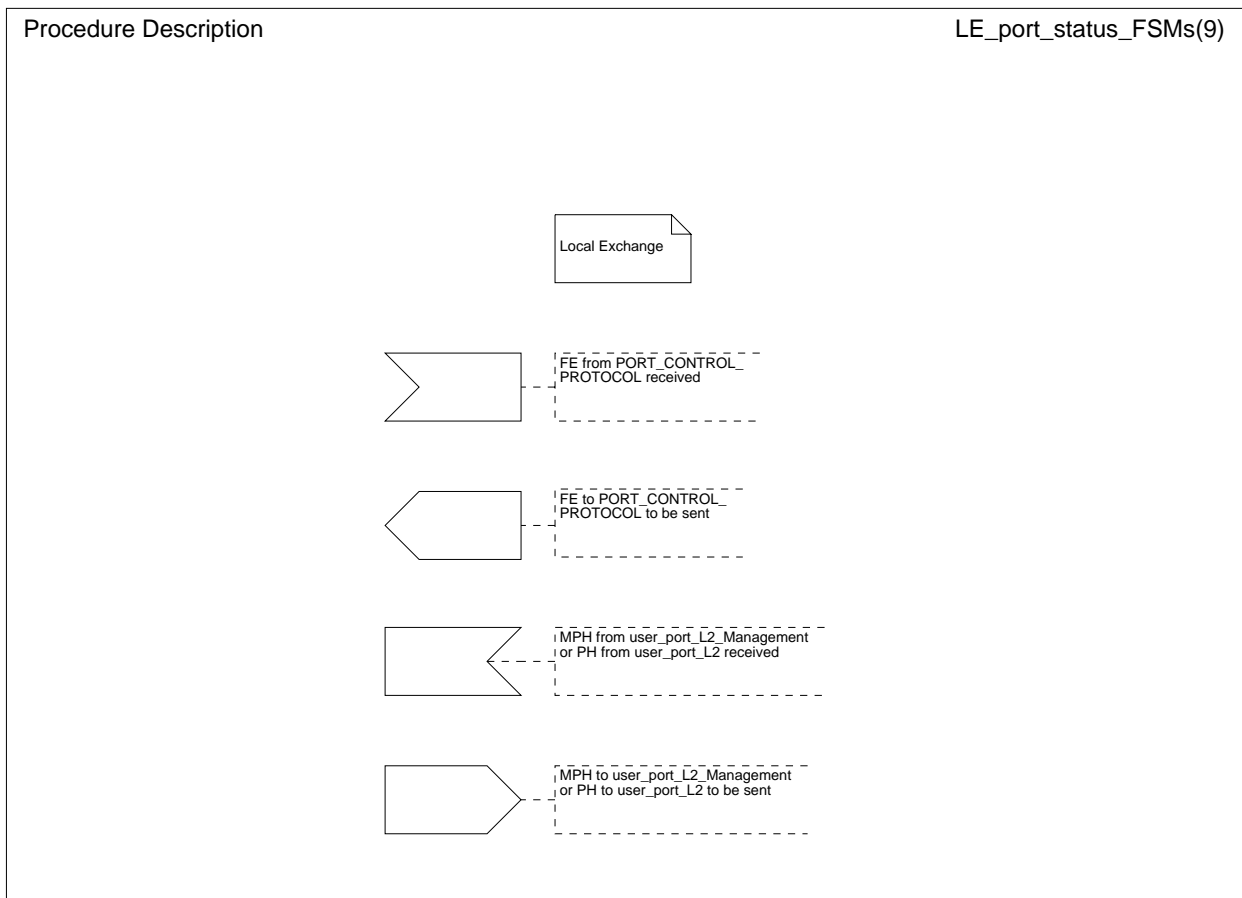
Figure L.29: Input and output symbols application - port status FSM control (LE-side)
