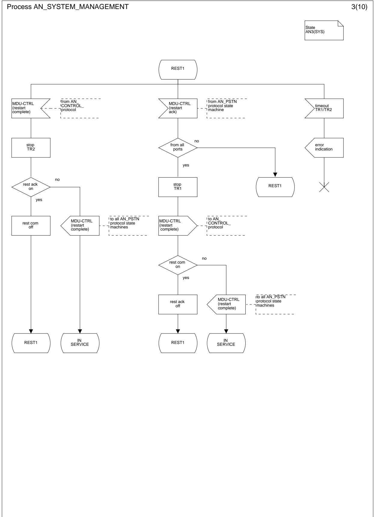
Figure L.17.3: System management AN-side; state REST1 (AN3(SYS))
