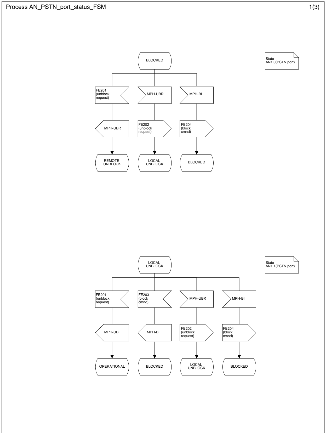
Figure L.15.1: PSTN port status FSM control AN-side; states BLOCKED (AN1.0(PSTN port)) and LOCAL UNBLOCK (AN1.1(PSTN port))
