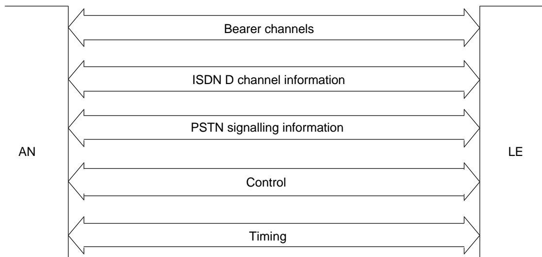
Figure 5: Functional description of the V5.1 interface
