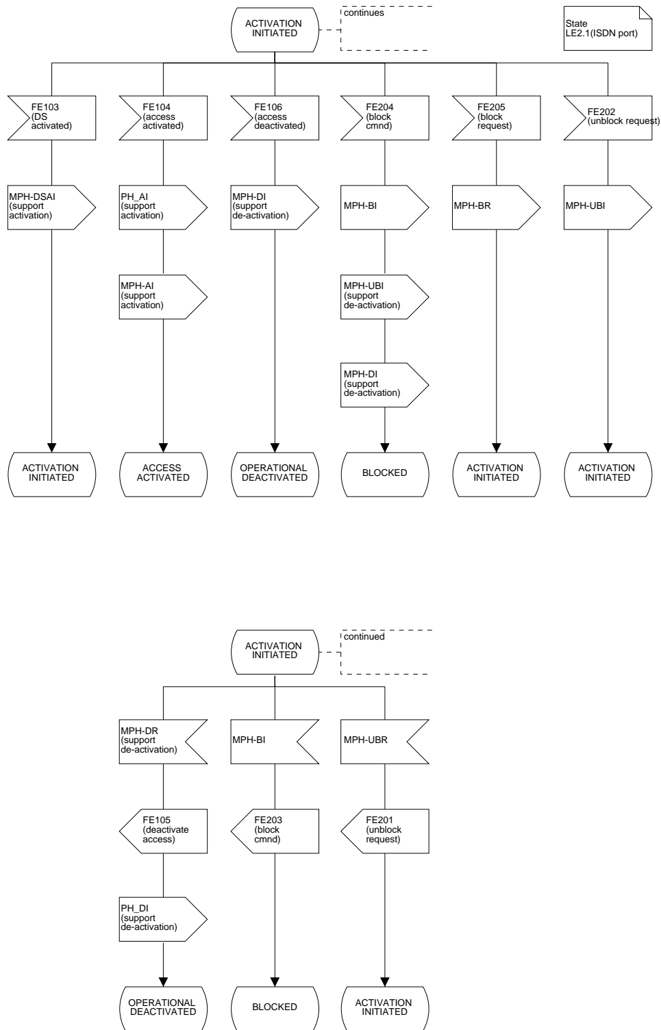
Figure L.30.4: ISDN port status FSM control LE-side; state ACTIVATION INITIATED (LE2.1(ISDN port))
