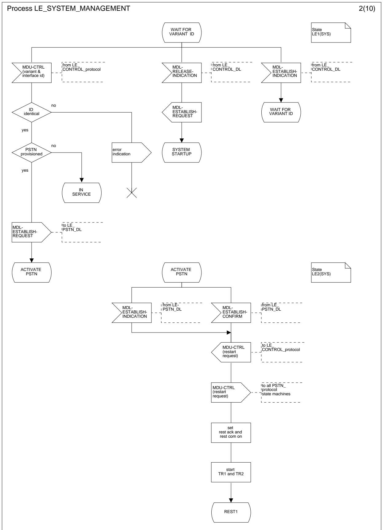
Figure L.33.2: System management LE-side; states WAIT FOR VARIANT ID (LE1(SYS)) and ACTIVATE PSTN (LE2(SYS))
