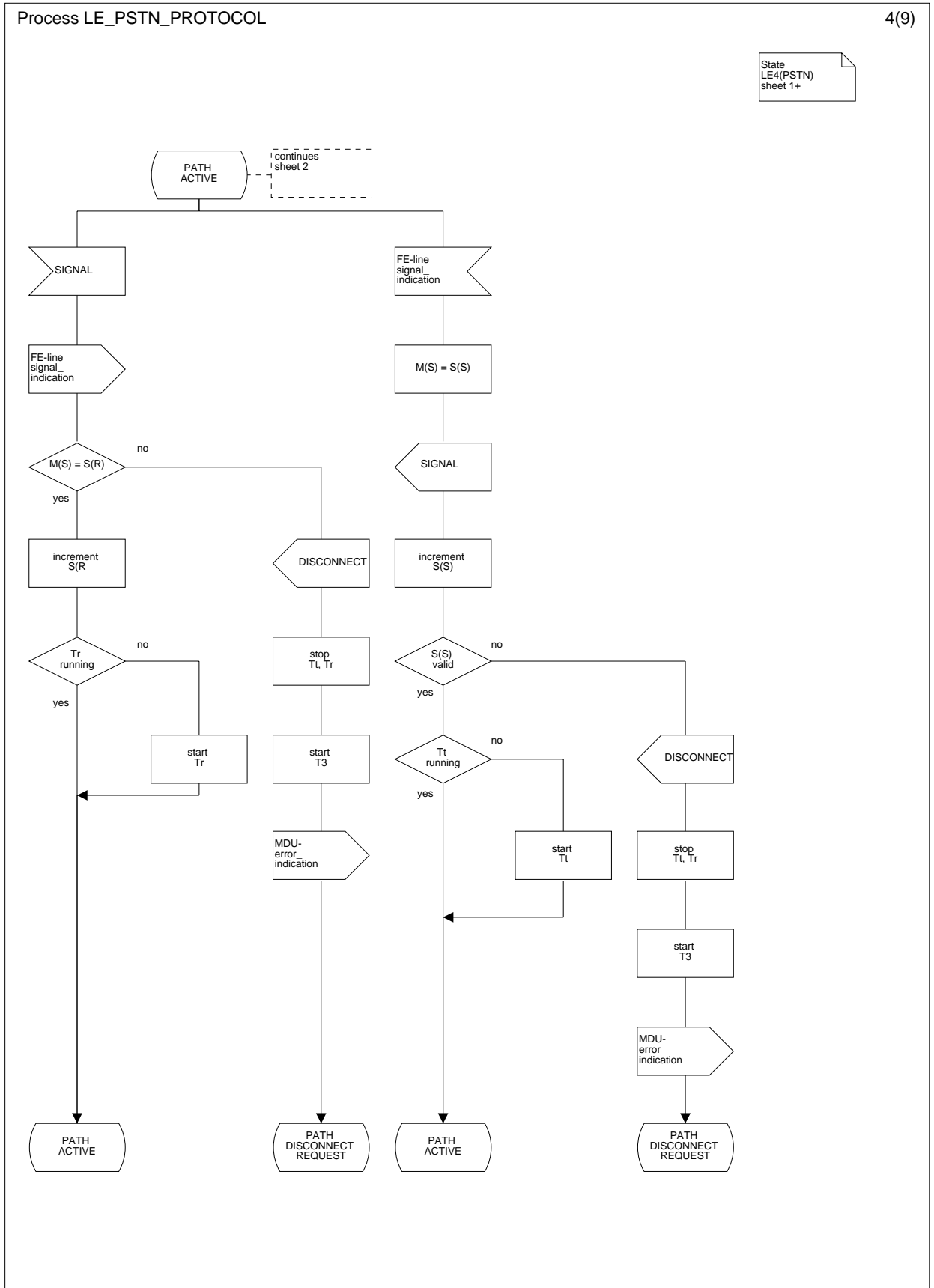
Figure L.25.4: PSTN protocol LE-side; state PATH ACTIVE (LE4(PSTN)) (sheet 1)
