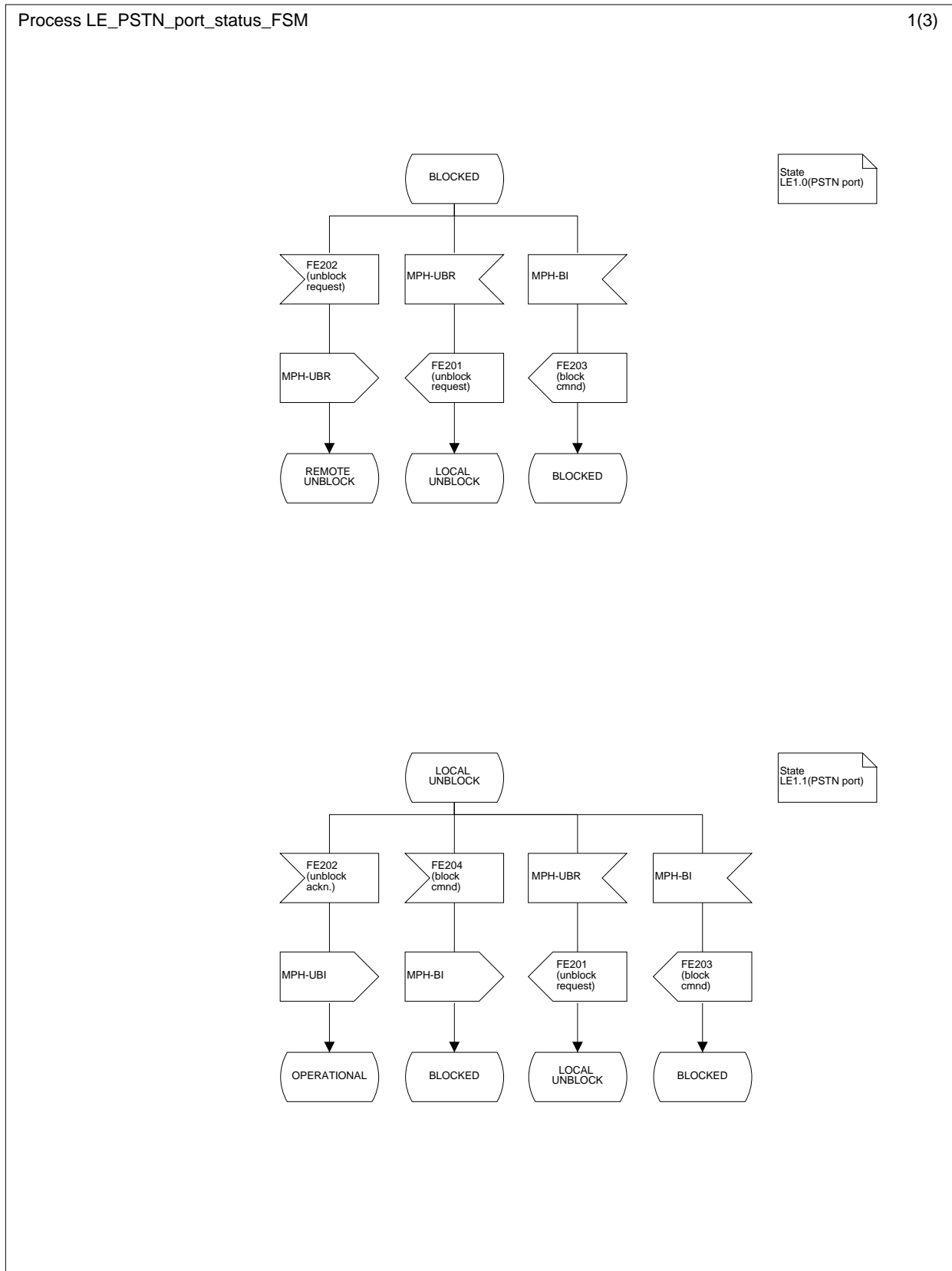
Figure L.31.1: PSTN port status FSM control LE-side; states BLOCKED (LE1.0(PSTN port)) and LOCAL UNBLOCK (LE1.1(PSTN port))
