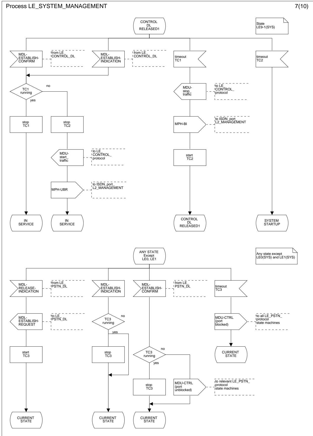
Figure L.33.7: System management LE-side; state CONTROL DL RELEASED1 (LE9-1(SYS)) and any state except LE0(SYS) and LE1(SYS)
