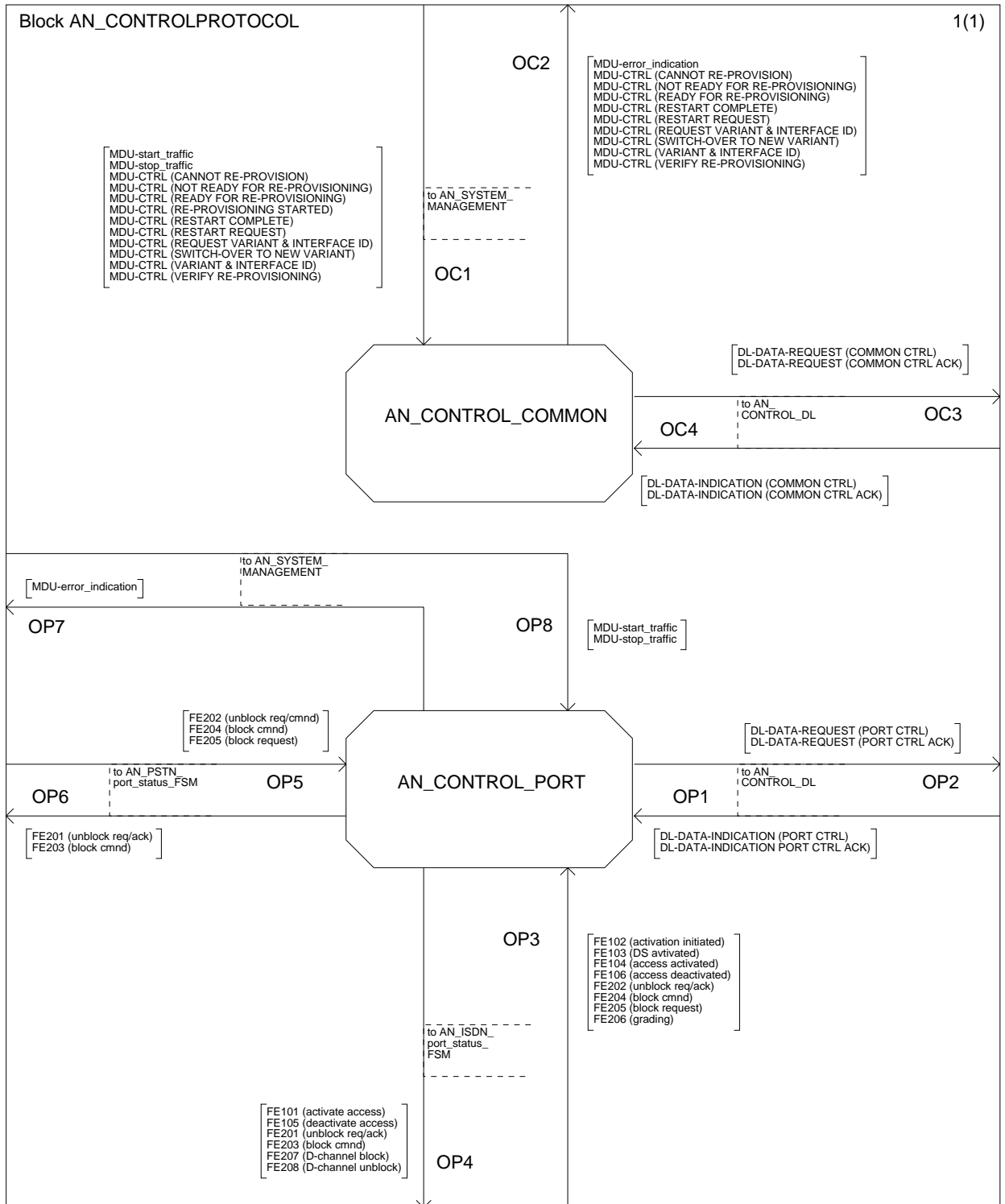
Figure L.3: Control protocol block description AN-side
