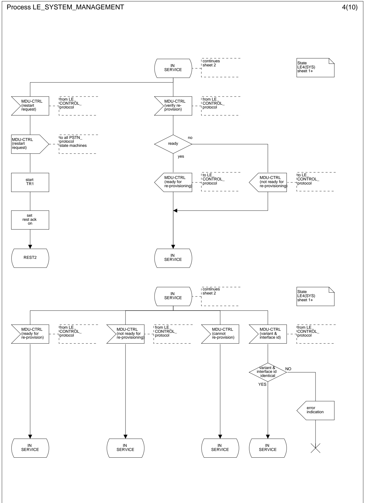
Figure L.33.4: System management LE-side; state IN SERVICE (LE4(SYS)) (sheet 1)
