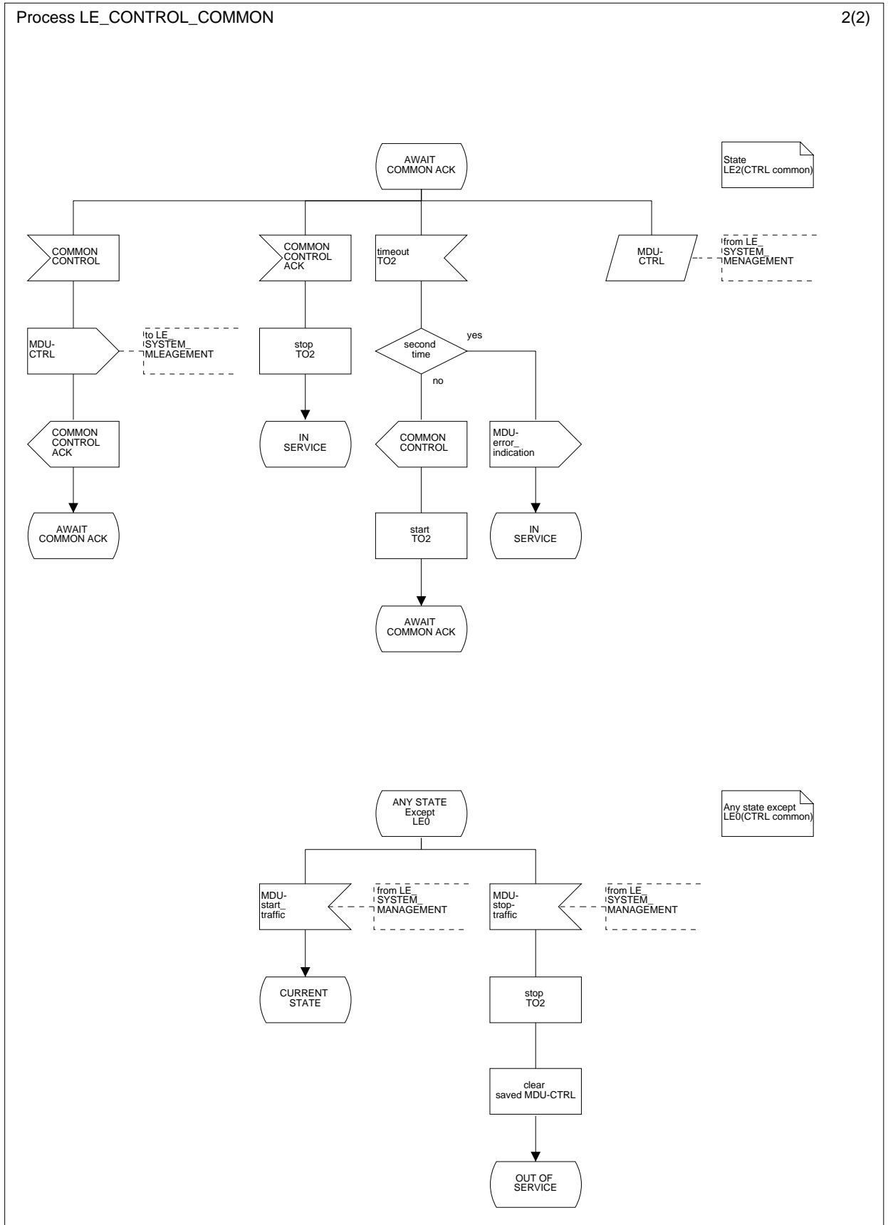
Figure L.28.2: Common control protocol LE-side; state AWAIT COMMON ACK (LE1(CTRL common)) and any state except LE0(CTRL common)
