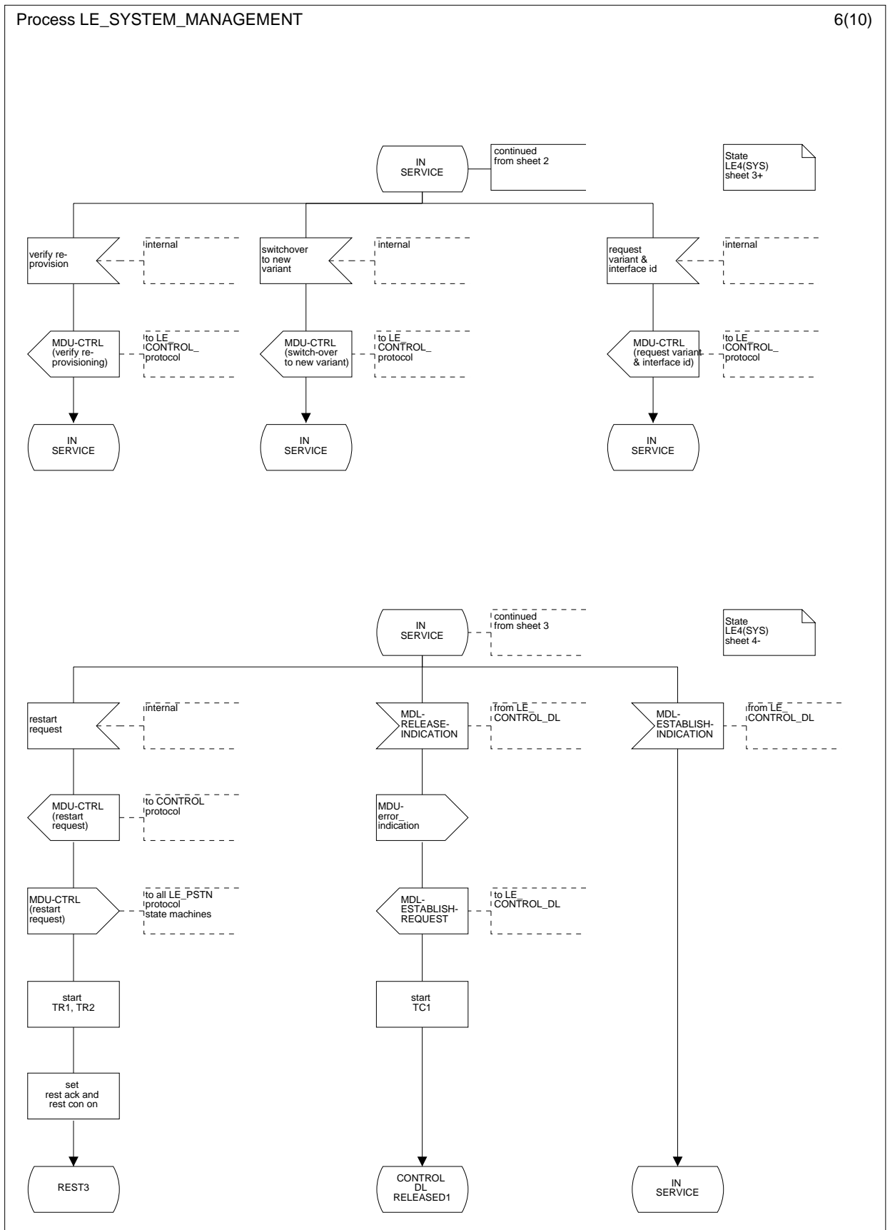
Figure L.33.6: System management LE-side; states IN SERVICE (LE4(SYS)) (sheet 3)
