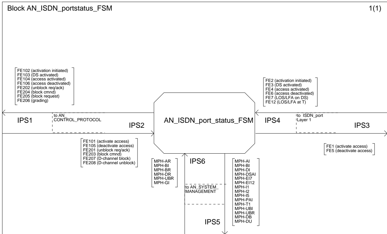
Figure L.4: ISDN port status FSM block description AN-side
