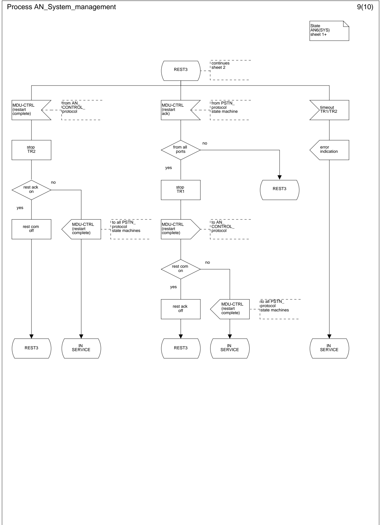
Figure L.17.9: System management AN-side; state REST3 (AN6(SYS)) (sheet 1)
