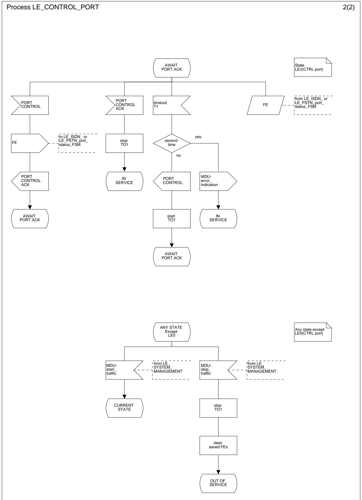
Figure L.27.2: Port control protocol LE-side; state AWAIT PORT ACK (LE2(CTRL port)) and any state except LE0(CTRL port)
