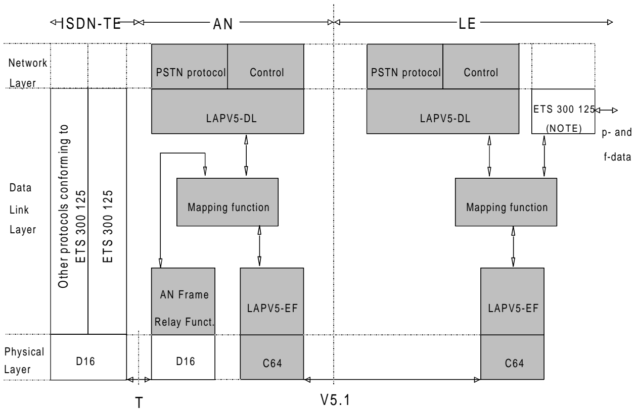
Figure 6: Protocol architecture
