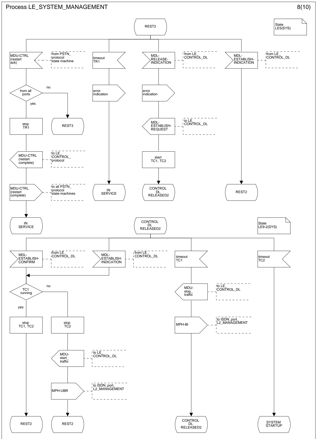
Figure L.33.8: System management LE-side; states REST2 (LE5(SYS)) and CONTROL DL RELEASED2 (LE9-2(SYS))
