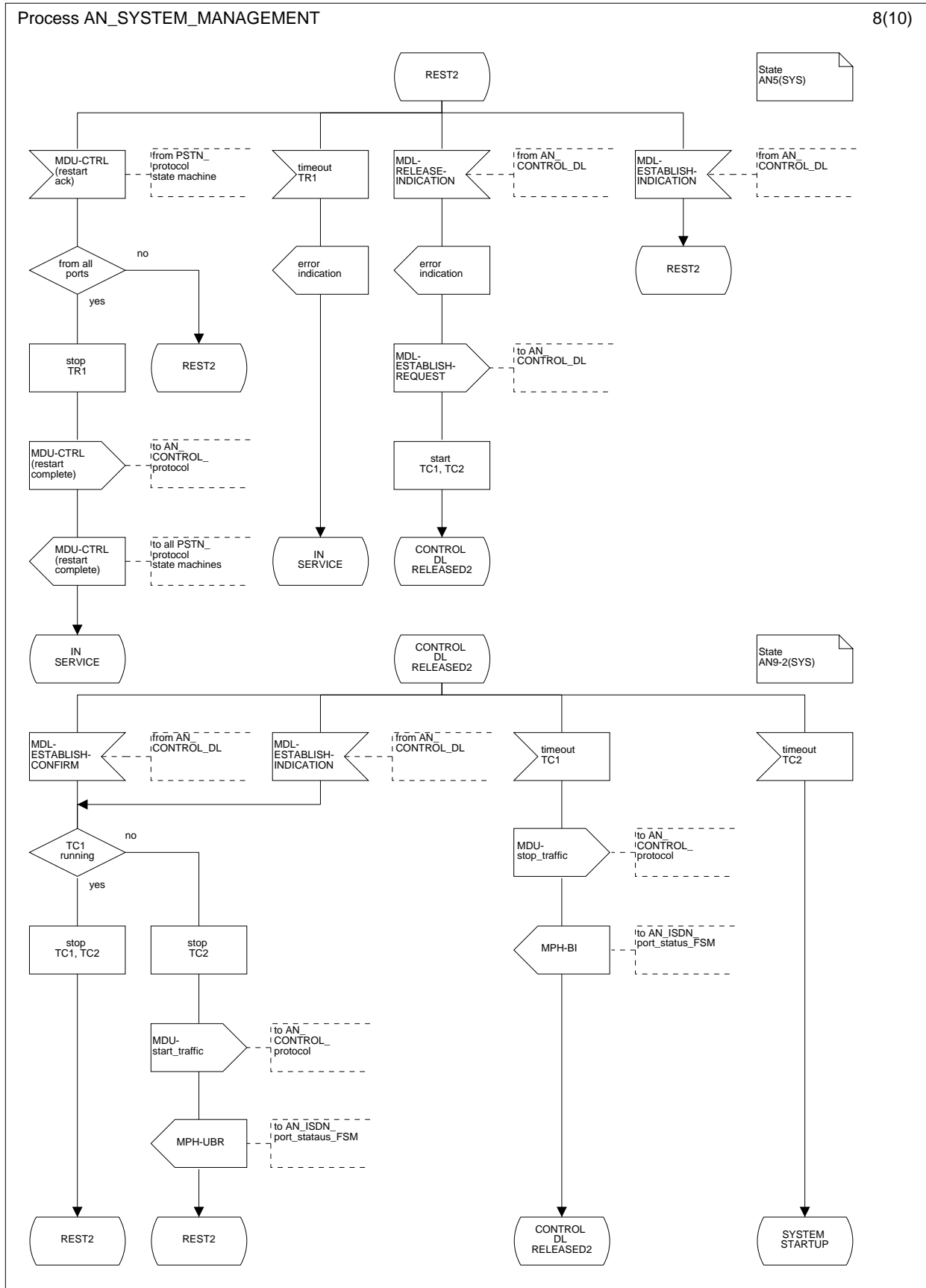
Figure L.17.8: System management AN-side; states REST2 (AN5(SYS)) and CONTROL DL RELEASED2 (AN9-2(SYS))
