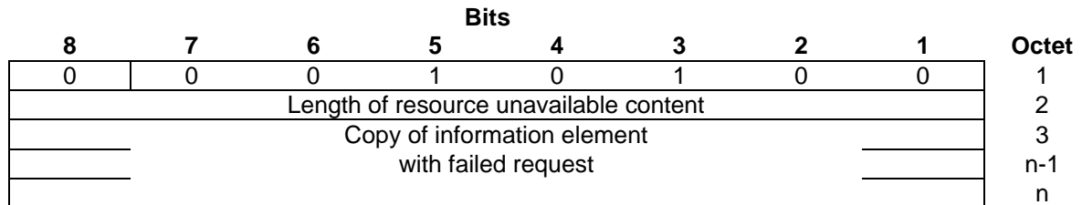
Figure 30: Resource-unavailable information element
