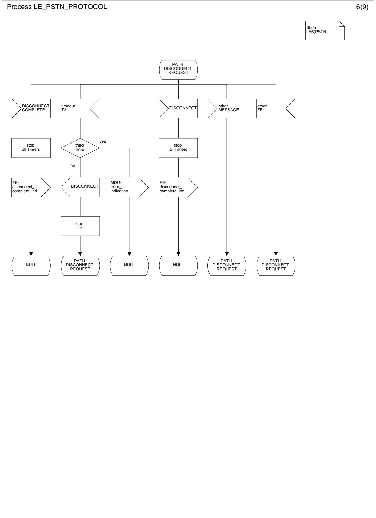
Figure L.25.6: PSTN protocol LE-side; state PATH DISCONNECT REQUEST (LE5(PSTN))
