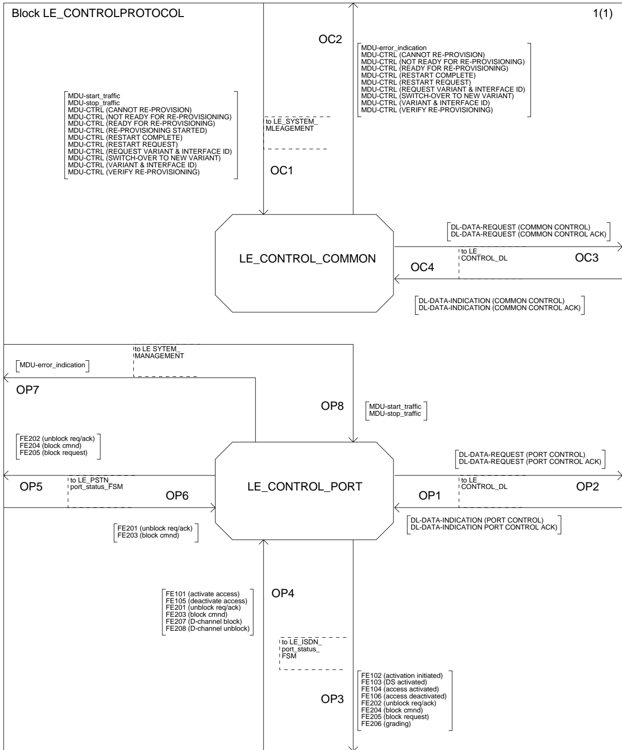
Figure L.20: Control protocol block description LE-side
