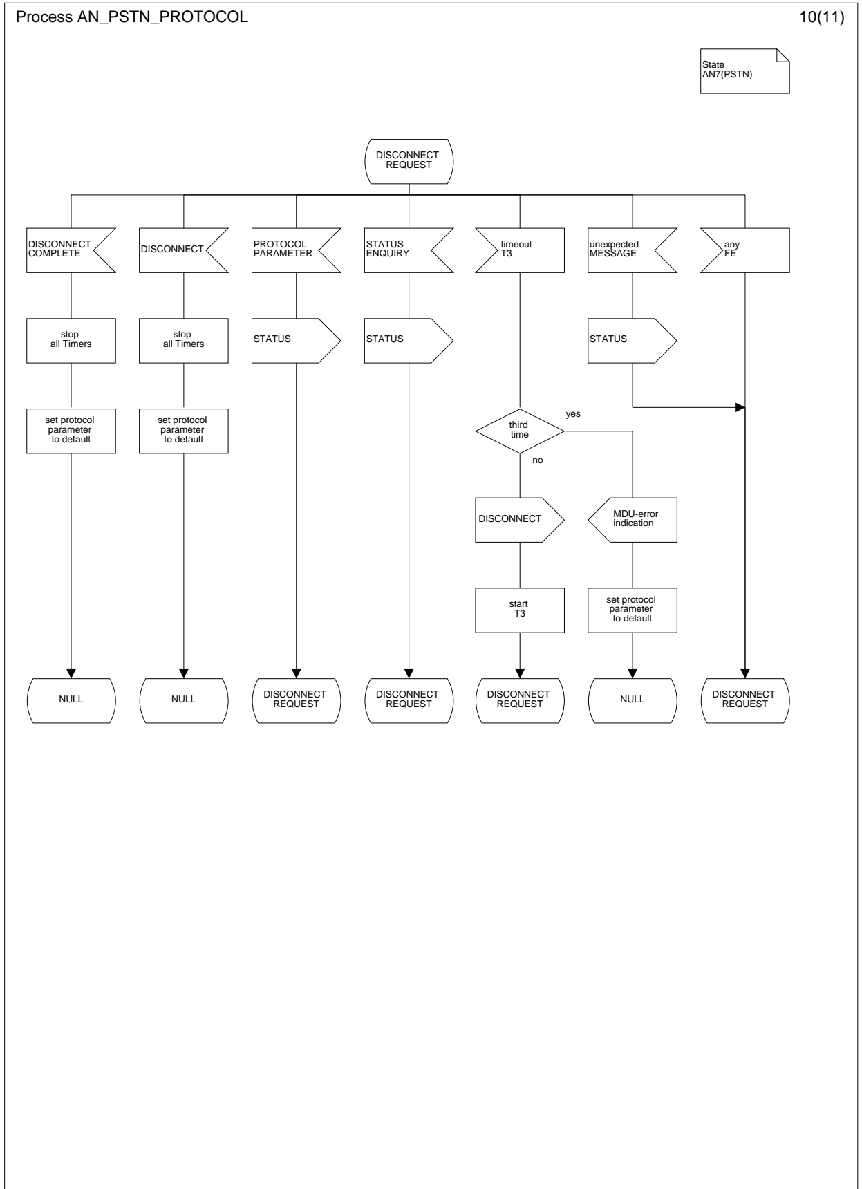
Figure L.9.10: PSTN protocol AN-side; state DISCONNECT REQUEST (AN7(PSTN))
