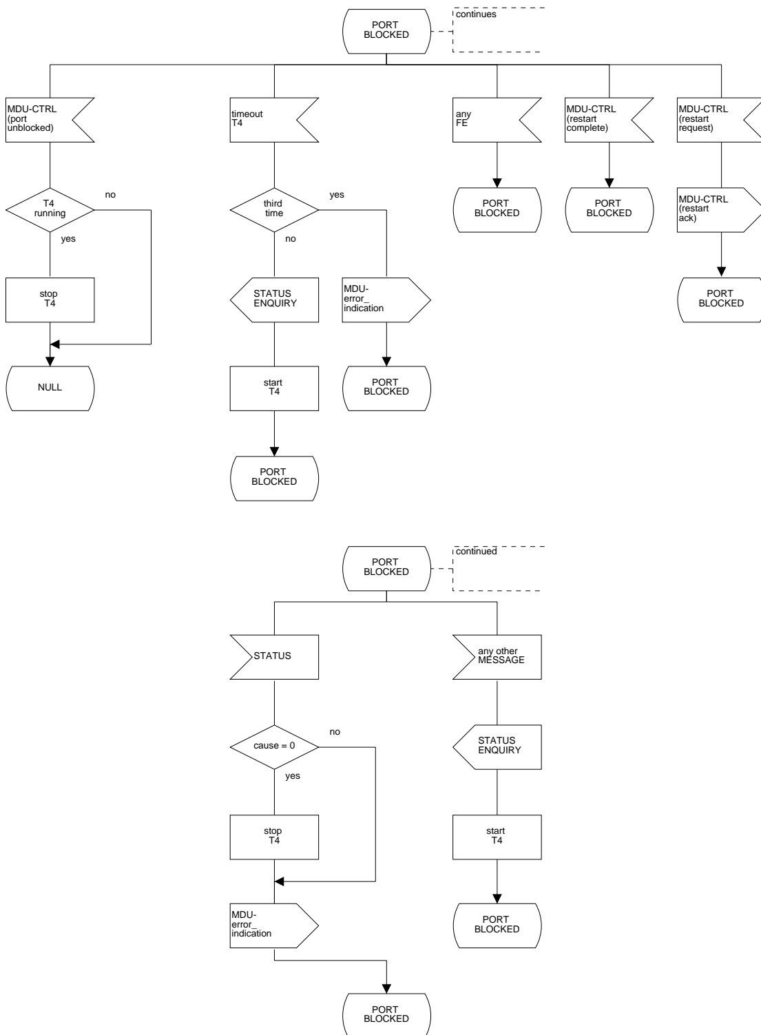
Figure L.25.7: PSTN protocol LE-side; state PORT BLOCKED (LE6(PSTN))
