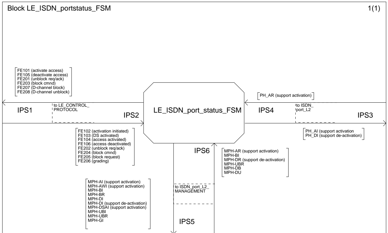
Figure L.21: ISDN port status FSM block description LE-side
