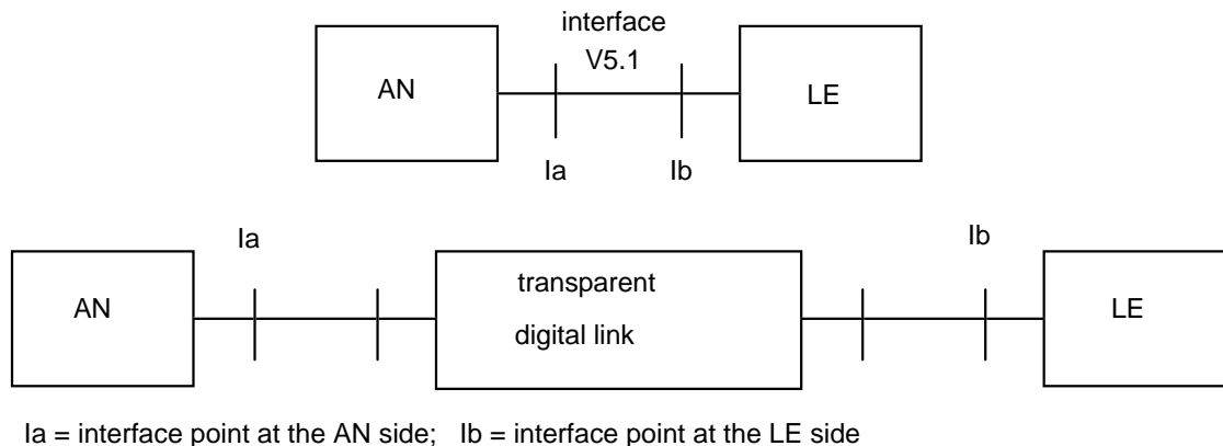
Figure 1: V5.1 application with and without transparent digital link
