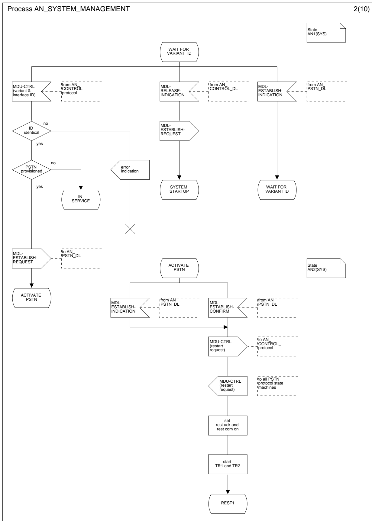
Figure L.17.2: System management AN-side; states WAIT FOR VARIANT ID (AN1(SYS)) and ACTIVATE PSTN (AN2(SYS))
