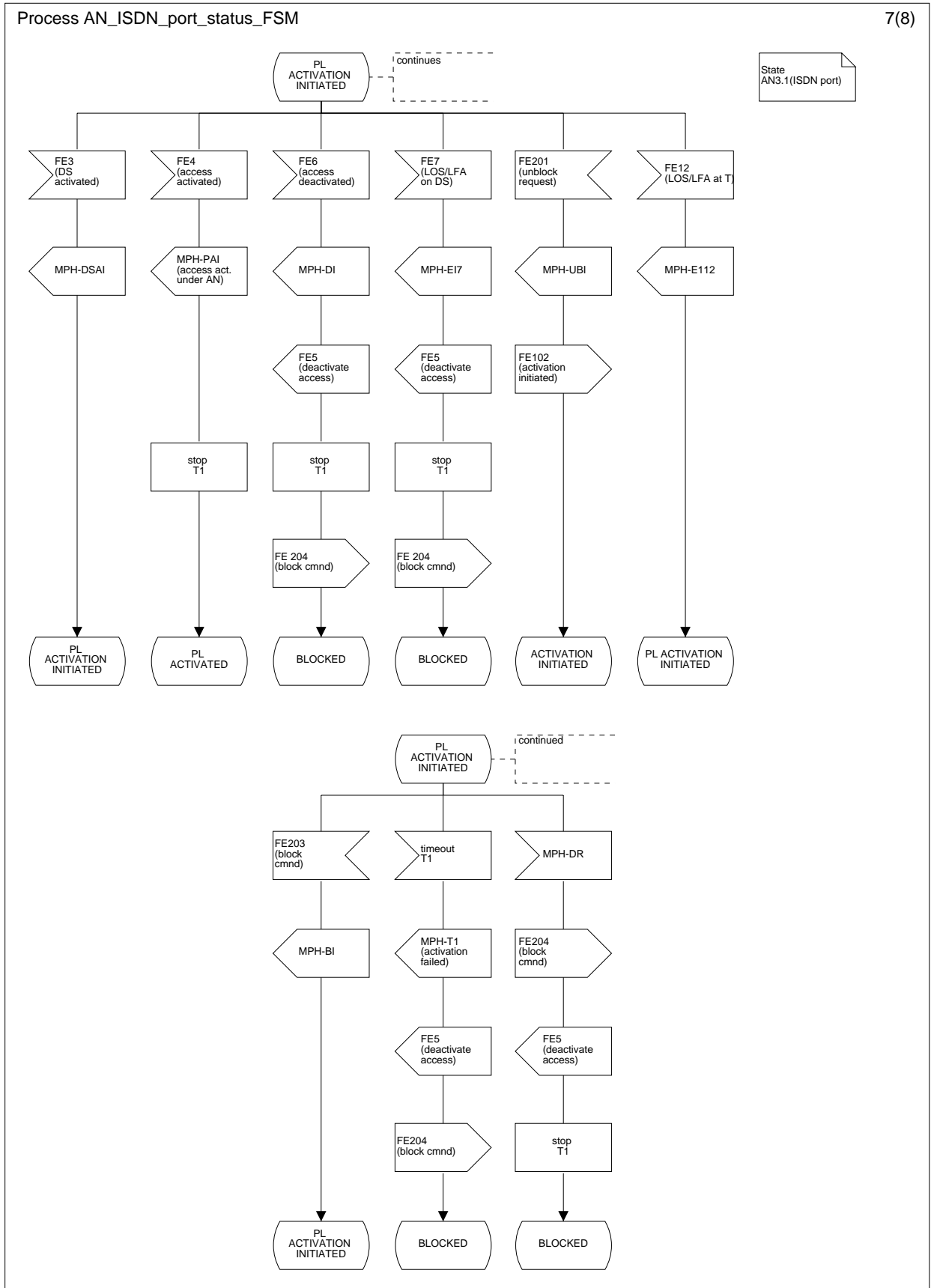
Figure L.14.7: ISDN port status FSM control AN-side; state PL ACTIVATION INITIATED (AN3.1 (ISDN port))
