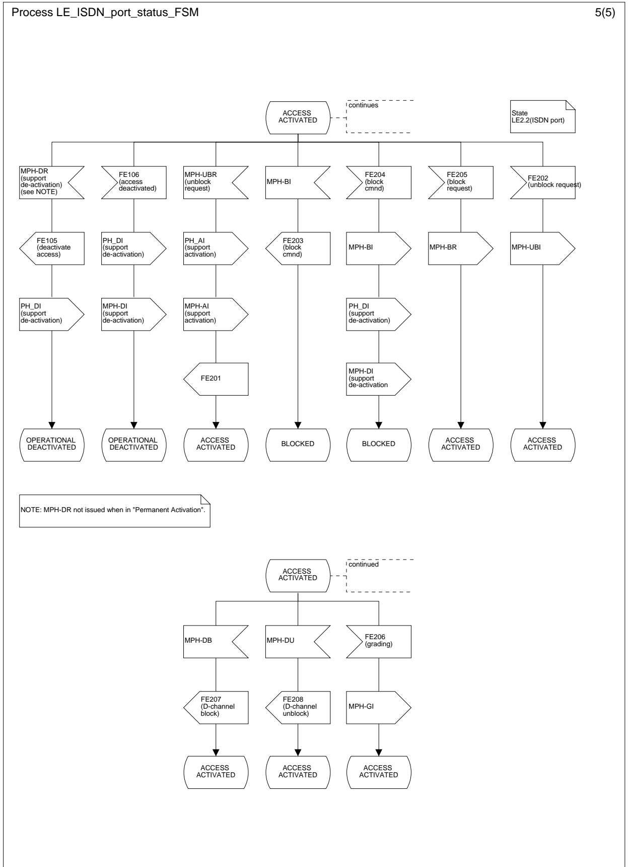
Figure L.30.5: ISDN port status FSM control LE-side; state ACCESS ACTIVATED (LE2.2(1SDN port))
