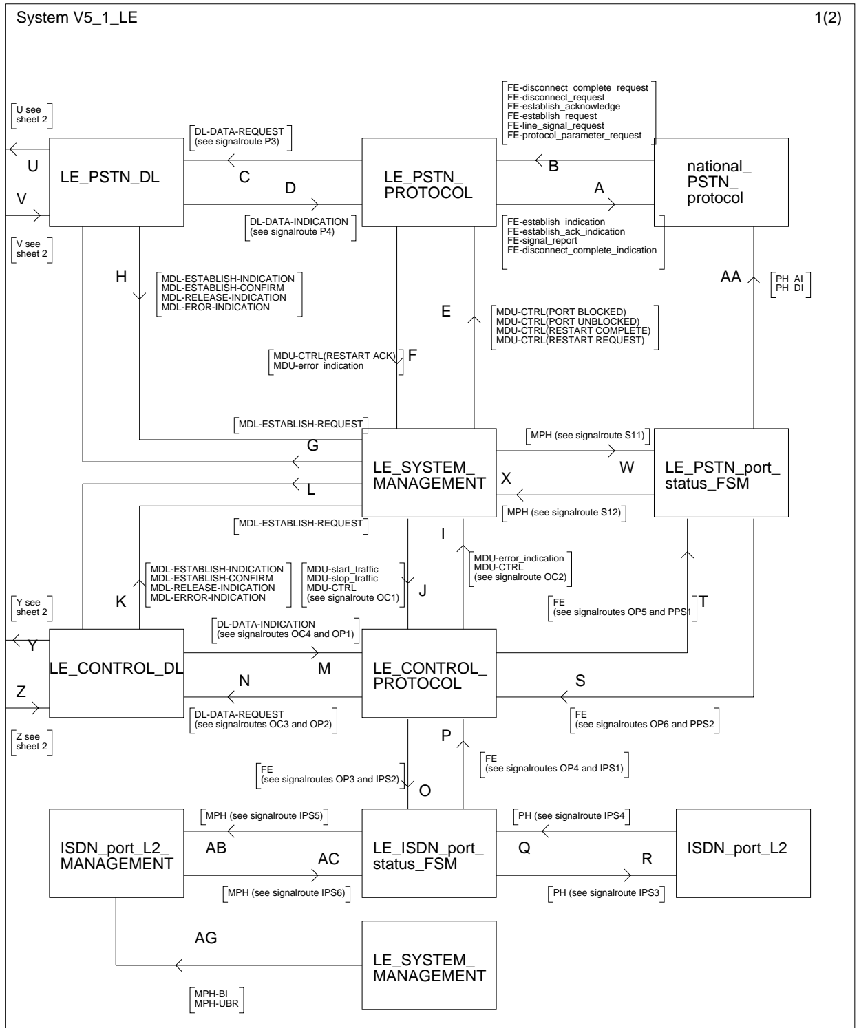
Figure L.18.1: V5.1 system overview LE-side (sheet 1)
