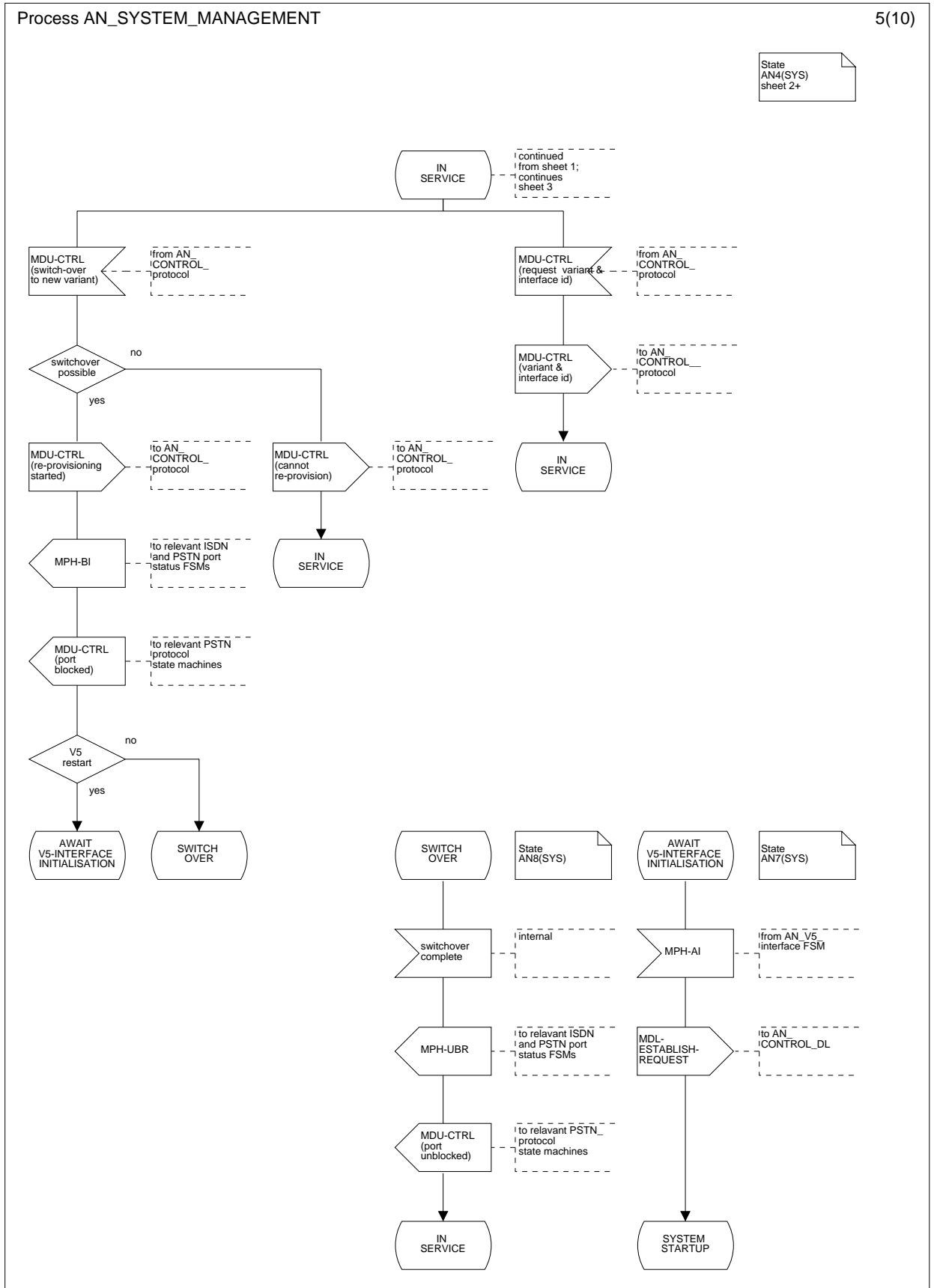
Figure L.17.5: System management An-side; state IN SERVICE (AN4(SYS)) (sheet 2 of 3), and states AWAIT V5-INTERFACE INITIALISATION (AN7(SYS)) and SWITCH OVER (AN8(SYS))
