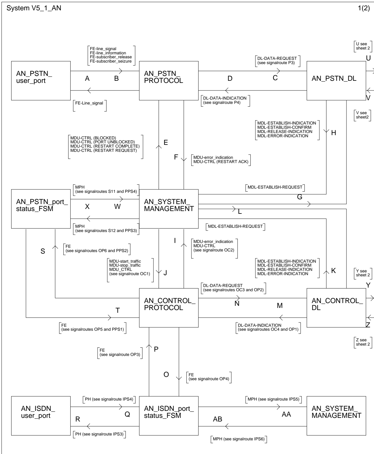
Figure L.1.1: V5.1 system overview AN-side (sheet 1 of 2)
