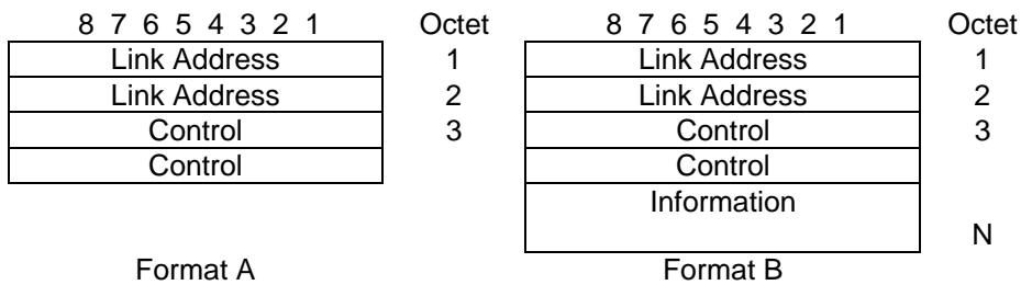
Figure 9: Data-link sublayer frame formats
