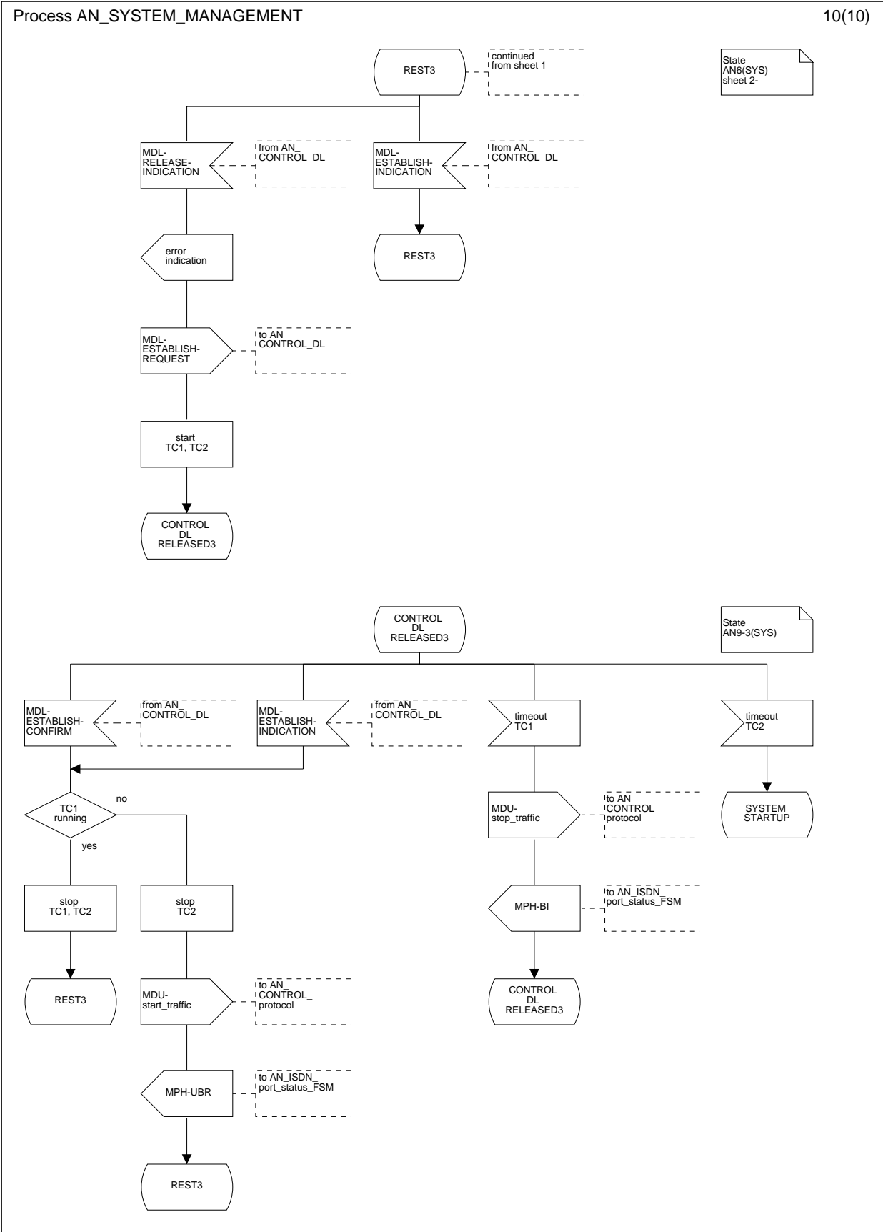
Figure L.17.10: System management AN-side; states CONTROL DL RELEASED3 (AN9-3(SYS)) and REST3 (AN6(SYS))
