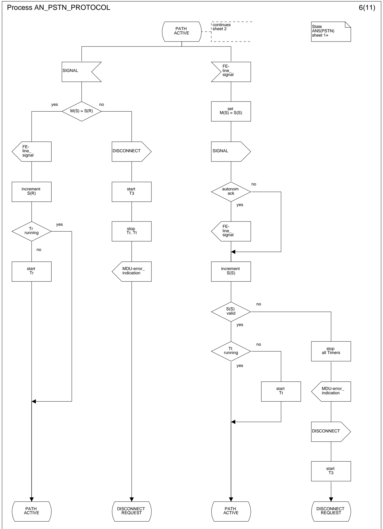
Figure L.9.6: PSTN protocol AN-side; state PATH ACTIVE (AN5(PSTN)) (sheet 1 of 3)
