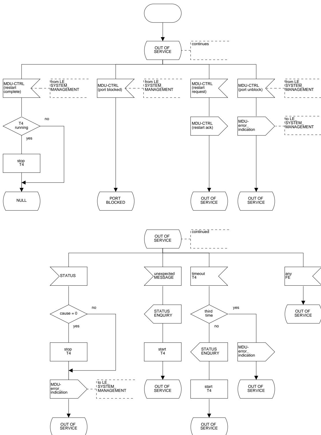
Figure L.25.1: PSTN protocol LE-side; state OUT OF SERVICE (LE0(PSTN))
