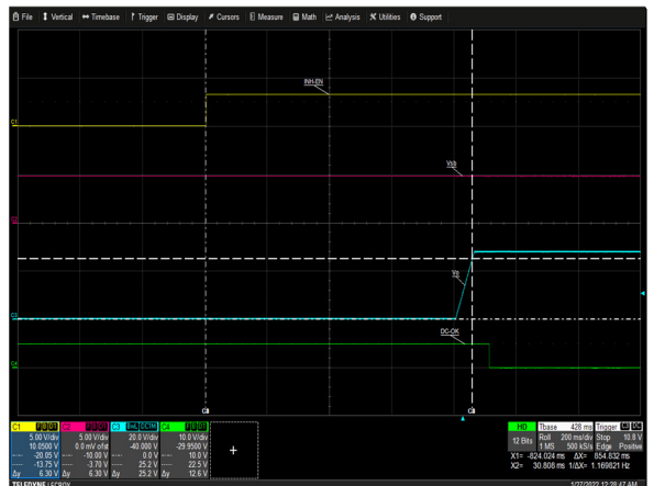
Figure 4: LCC1200-28U-9P Turn-on delay via INH_EN Vin = 264Vac Load: Io = 42.9A (12V), I SB = 1.5A (5V) Ch 1: INH_EN Ch 2: V SB Ch 3: V 0 CH 4: G_DCOK_C
