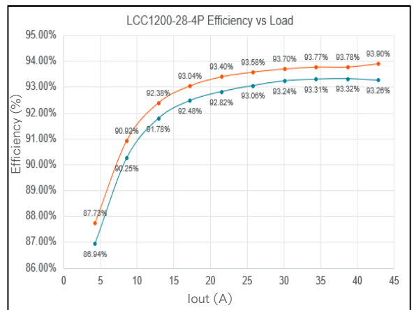
Figure 12: LCC1200-28U-4P Efficiency Curve @ 25°C Loading: I o,main = 10% I o,max increment to 1200W@180/230Vac
