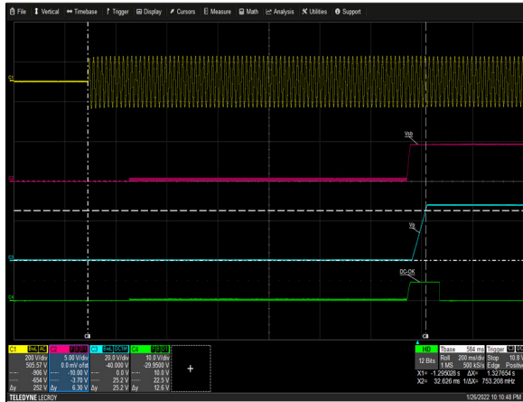
Figure 1: LCC1200-28U-9P Turn-on delay via AC mains Vin = 90Vac Load: Io = 25A (28V), I SB = 1.5A (5V) Ch 1: AC Mains Ch 2: V SB Ch 3: V 0 CH 4: G_DCOK_C
