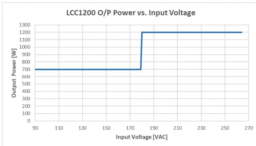
Figure 15. Output Power Vs Input Voltage
