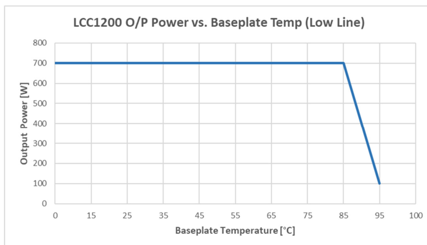
Figure 13. Output Power Vs Baseplate Temperature (low line: 90 Vac to 179 Vac)
