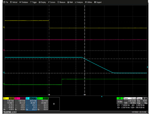
Figure 8: LCC1200-28U-9P Turn Off Characteristic via INH_EN Load: Io = 42.9A (12V), I SB = 1.5A (5V) Ch 1: INH_EN Ch 2: V SB Ch 3: V O CH 4: G_DCOK_C
