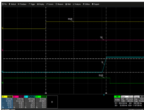
Figure 3: LCC1200-28U-9P Turn-on delay via INH_EN Vin = 90Vac Load: Io = 25A (12V), I SB = 1.5A (5V) Ch 1: INH_EN Ch 2: V SB Ch 3: V 0 CH 4: G_DCOK_C
