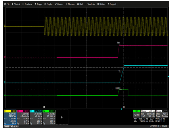
Figure 2: LCC1200-28U-9P Turn-on delay via AC mains Vin = 264Vac Load: Io = 42.9A (28V), I SB = 1.5A (5V) Ch 1: AC Mains Ch 2: V SB Ch 3: V 0 CH 4: G_DCOK_C
