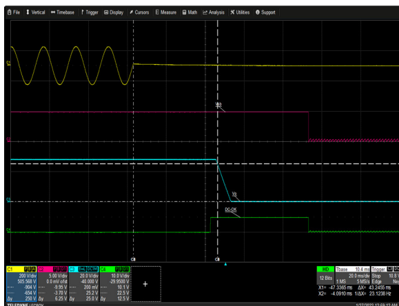
Figure 5: LCC1200-28U-9P Hold-up Time Vin = 90Vac Load: Io = 25A (12V), I SB = 1.5A (5V) Ch 1: AC Mains Ch 2: V SB Ch 3: V 0 CH 4: G_DCOK_C
