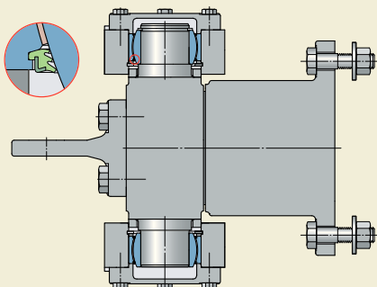
Road roller articulation joint
