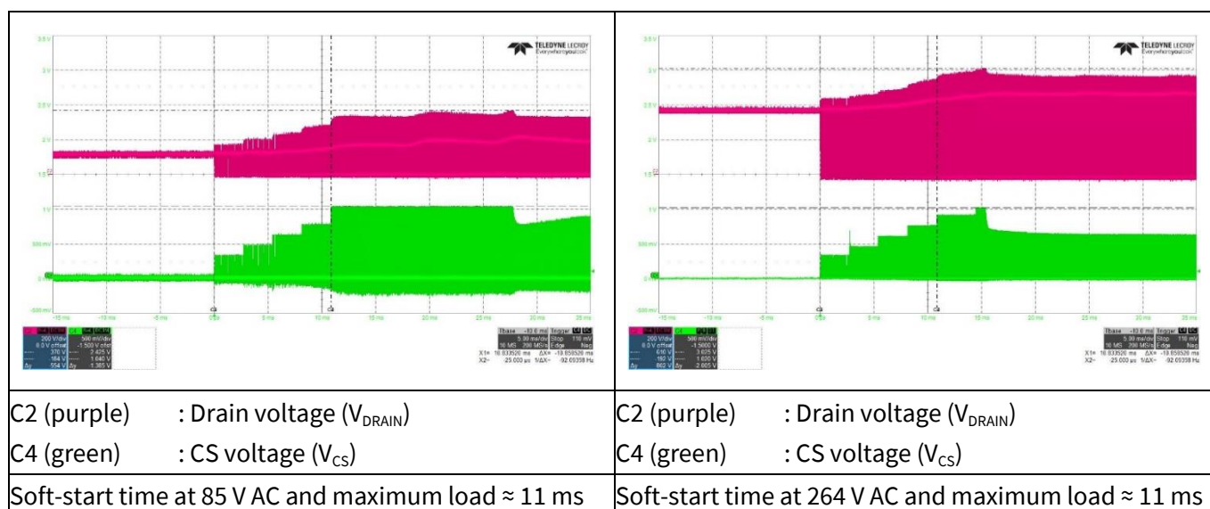
Figure 15 Soft-start
