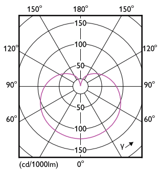
Light Distribution Diagram - BC8.8A19/AMB/927-22 WG 120V LA
