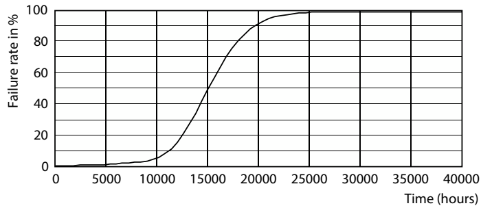
Life Expectancy Diagram - BC8.8A19/AMB/927-22 WG 120V LA
