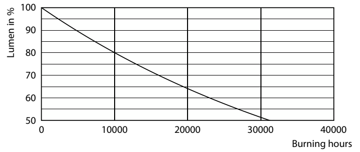
Lumen Maintenance Diagram - BC8.8A19/AMB/927-22 WG 120V LA
