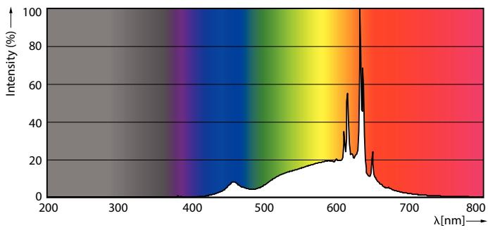
Spectral Power Distribution Colour - BC8.8A19/AMB/927-22 WG 120V LA
