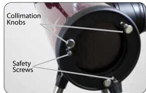
FIGURE 6-2 Collimation Knobs
