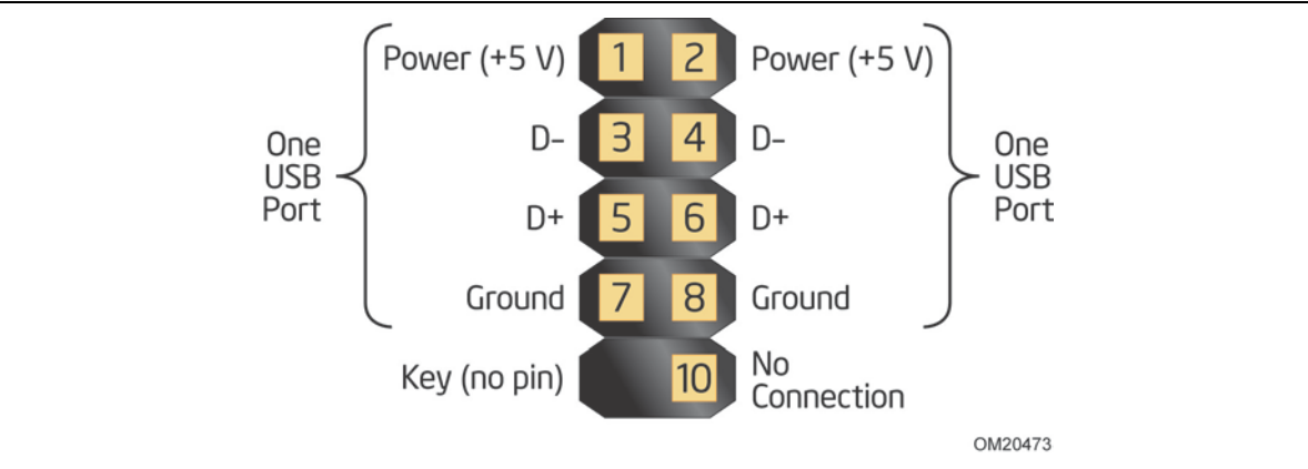
Figure 12. Connection Diagram for Front Panel USB 2.0 Headers
