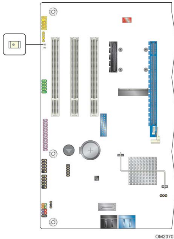
Figure 7. Location of the Standby Power LED
