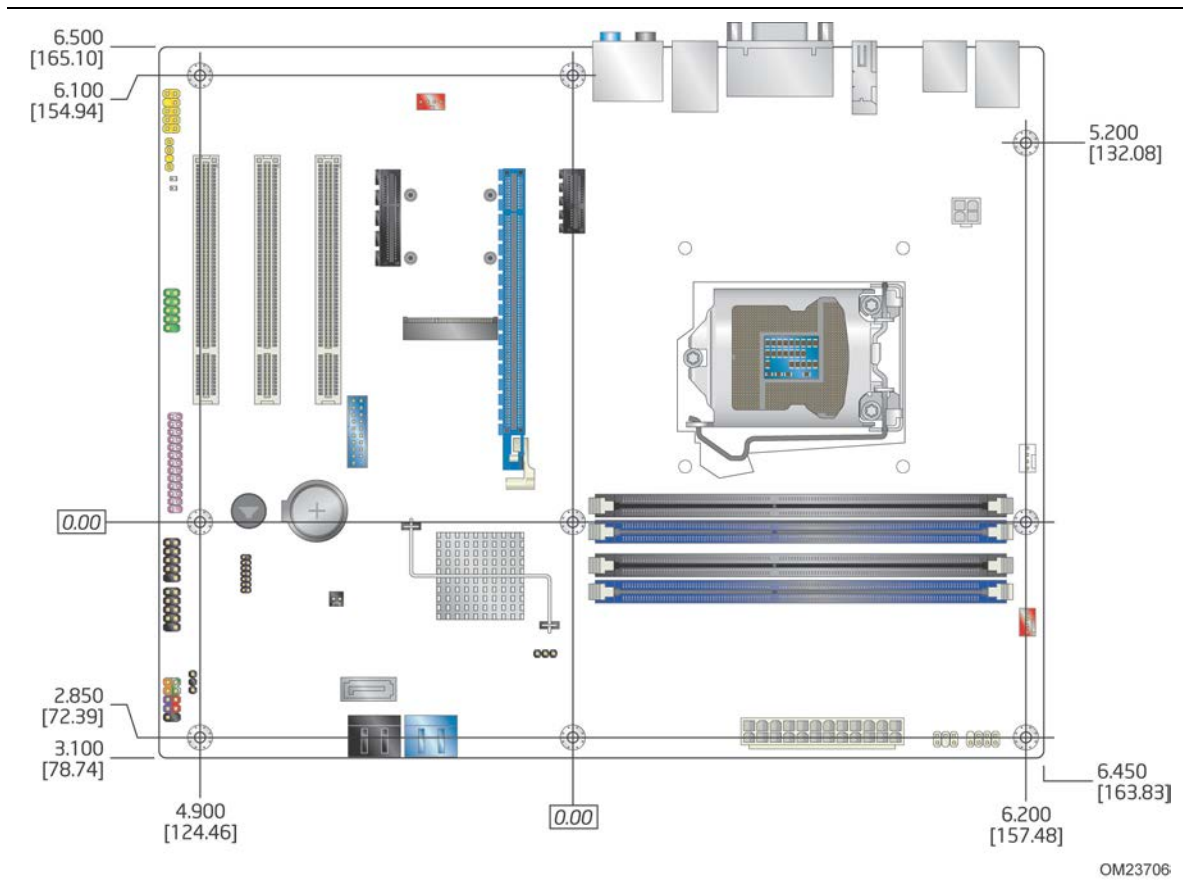
Figure 14. Board Dimensions
