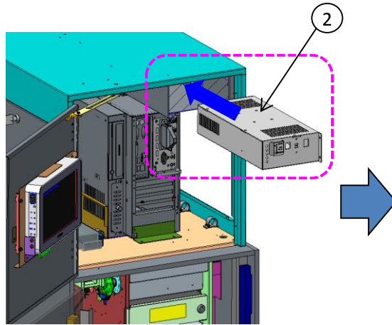
2-1. Install power supply in the system
