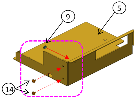
1-1. Assemble CE Brkt using Screw - fasten 3 points(No.9,14)
