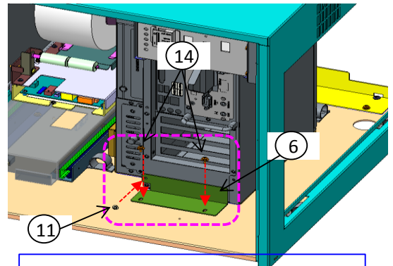
1-4. Install brkt in the system - fasten 3 points(No.11,14)
