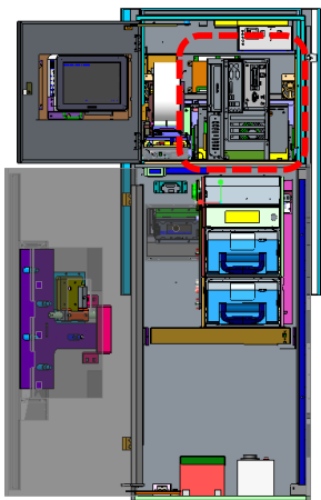
1-1. Assemble CE Brkt using Screw - fasten 3 points(No.9,14)
