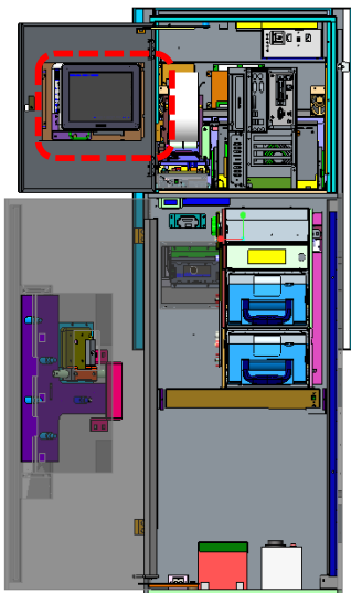
3-1. Install SPL brkt in the system - fasten 5 points(No.12,14)
