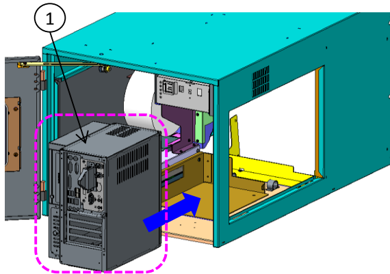
1-3. Install CE Assy in the system
