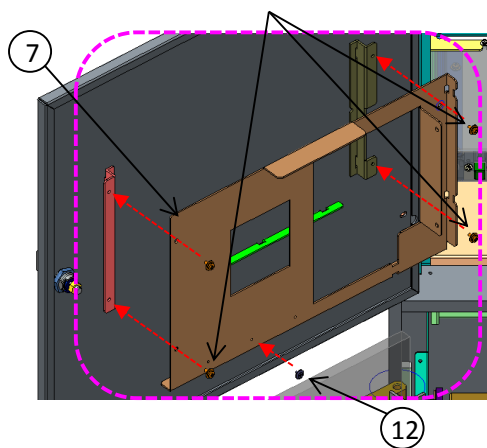
3-1. Install SPL brkt in the system - fasten 5 points(No.12,14)
