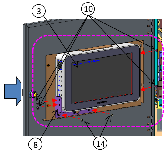
3-2 Install SPL in the system(w/Brkt) - fasten 6 points(No.10,14)
