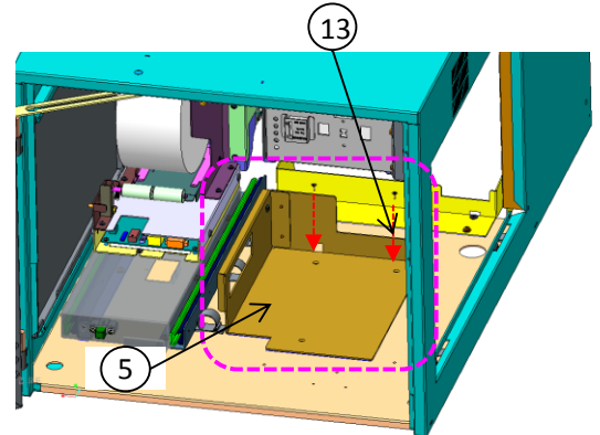
1-2. Install CE brkt Assy in the system - fasten 2 points(No.13)
