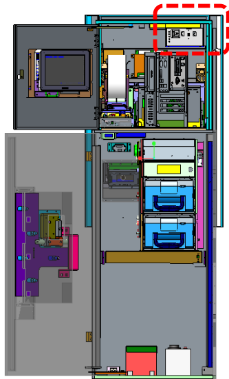
2-1. Install power supply in the system
