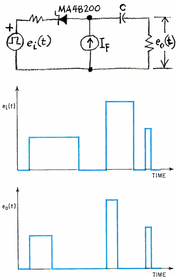
Pulse area limiter. The bias current I_F sets the stored charge and thus the area of the output pulse. Input pulses less than a critical area are passed unchanged, but pulses of greater area are limited to a fixed area, with the same amplitude but of less width.
