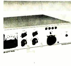
Power supply tester MPST-06 can simulate the full range of loading conditions faced by computer power supplies in actual use. It has a voltage slew rate of 5 v/ \mu sec and a typical current slew rate of 2.5 amps/ \mu sec. It can be used in either a rack or bench setup. Price is under $1,000; delivery, 30 to 45 days. Raytheon Computer, 2700 S. Fairview St., Santa Ana, Calif. [368]
