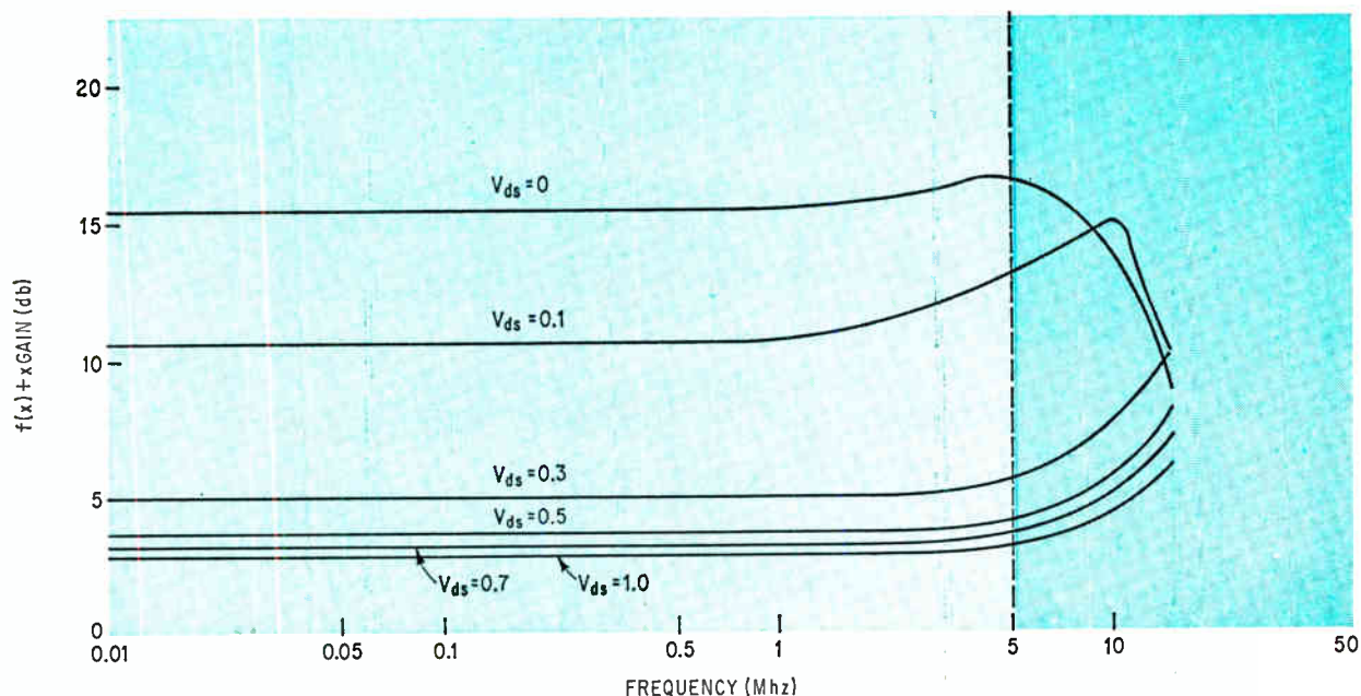
Biasing. Incremental gain curves show effect of bias from 0 to 1 volt.
