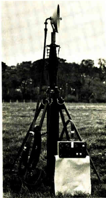
Line of sight. Gunn diode featured in receiver portion of new transceiver
