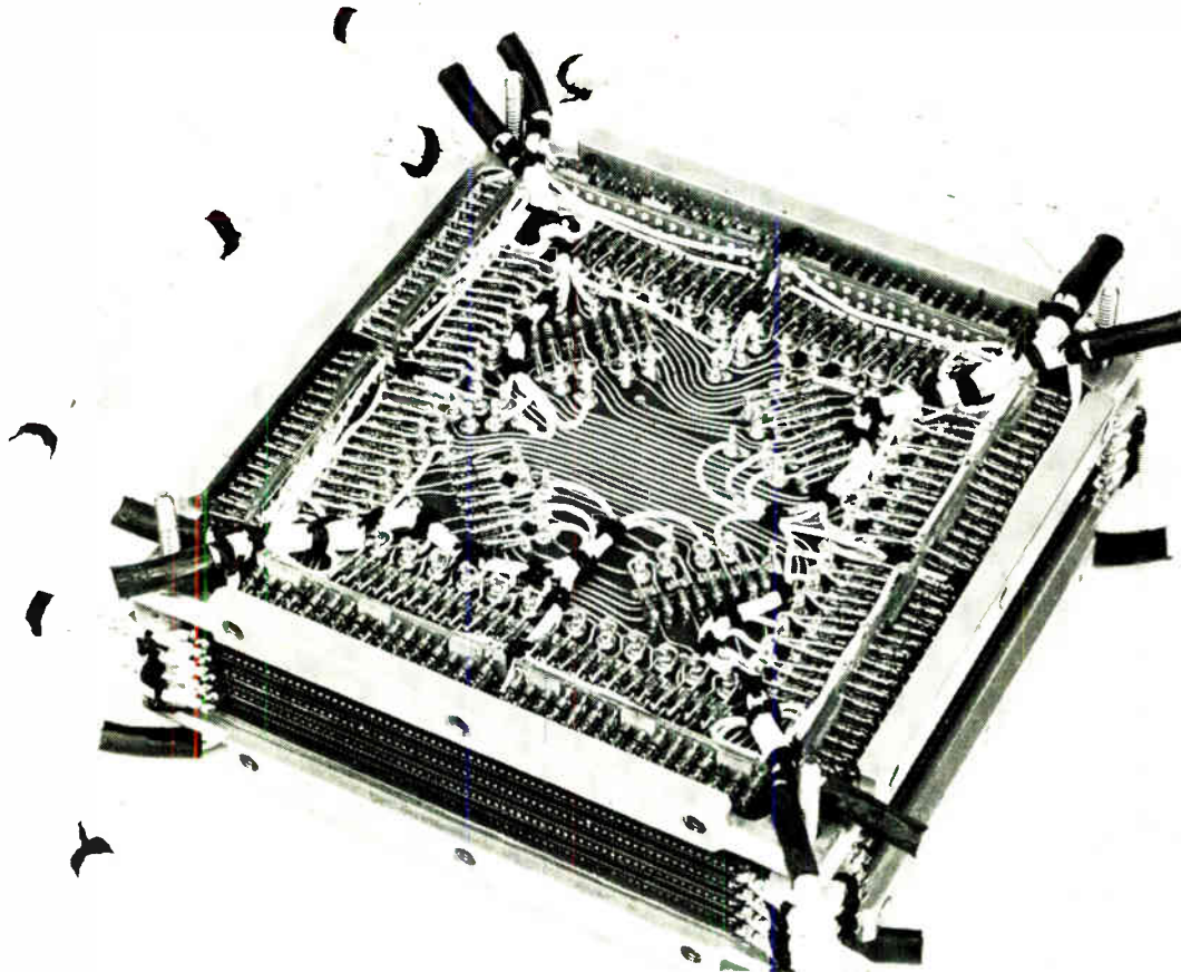
Battle ready. This memory stack, designed to withstand the stresses and strains of military applications, can store 4,096 words of eight bits each. Current-steering diodes are visible on the top layer.
