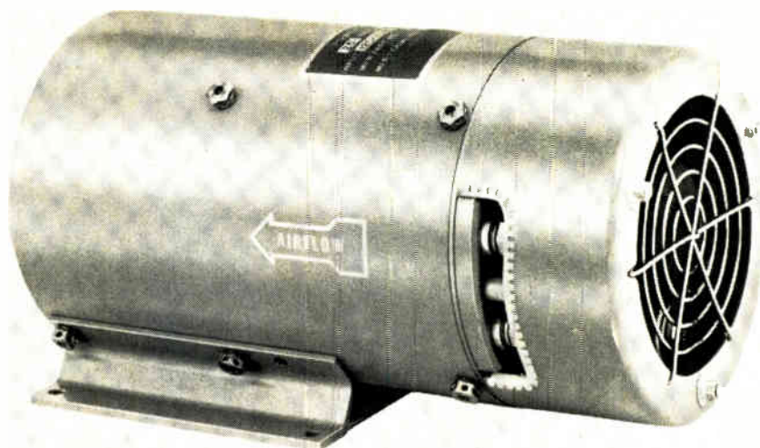
28G5P 47-65 Hz input (also style 28GP for 400 Hz), high-efficiency 28 V.D.C. output; lightest, most compact static unit.
