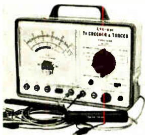
Multifunction instrument model LTC-901 is used for both in-circuit and out-of-circuit transistor checking. Beta and I_{CBO} of transistors as well as diode quality may be determined. A special section of the instrument performs the function of a signal tracer for both a-f and r-f applications. Price is $69. Leader Instruments Corp., 24-20 Jackson Ave., L.I.C., N.Y. 11101. [365]
