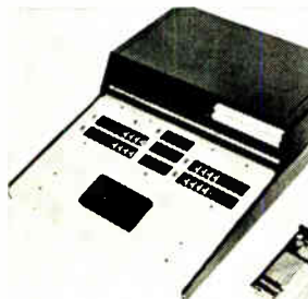
IC tester model 1740C features card programming capability with the added flexibility of thumb-wheel switches. It is designed for use in areas where both high speed testing and evaluation of IC parameters is needed such as incoming inspection, wafer sorting, and final inspection. Unit weighs about 40 lbs. Miracle-Hill Electronics Inc., 320 Martin Ave., Santa Clara, Calif. [366]
