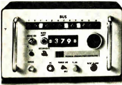
Watchdog. This module assures privacy when used with TCC's digital ship-to-ship communications system.
