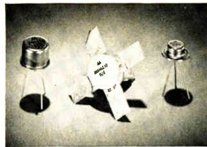
Package trio. The new devices come in TO-39 case, left; SOE (stripline-opposed emitter), center; and TO-107.
