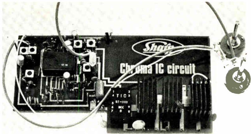
On the shelf. Color chroma circuits are part of an all-IC receiver made by a Japanese consortium; the set won't be marketed for several years.
