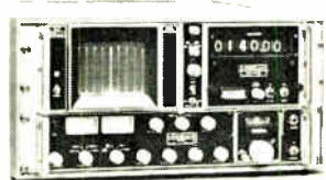
Scanning receiver system RS-160 uses a varactor-tuned preselector that covers 30-300 Mhz in four plug-in heads. It can be used in manual or sweep modes. A signal monitor displays the entire band or any portion of it, and a digital readout gives a direct frequency display and digital automatic frequency control. CEI div. of Watkins-Johnson Co., 6006 Executive Blvd., Rockville, Md. [388]
