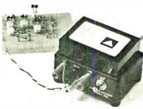
Manifold model 950 accepts plug-in d-c power supplies, and provides a safe and inexpensive source of ±15 v d-c power for breadboarding and general laboratory use. It comes with 4 feet of 3-wire line cord, on-off switch, fuse, socket for accepting the encapsulated supply, and 4 output terminals. Single units list for $16. Analog Devices Inc., 221 Fifth St., Cambridge, Mass. [387]
