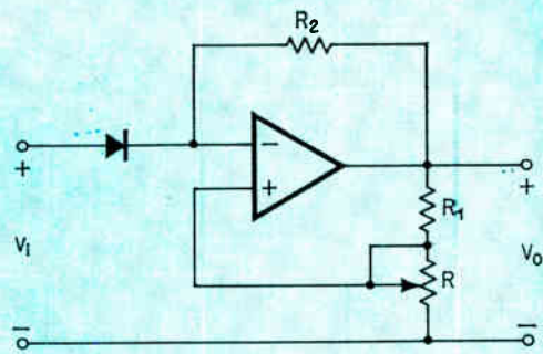
ANTI-LOGARITHMIC AMPLIFIER
