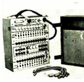
Portable data interface test set model 505-1 permits immediate isolation of trouble conditions in business machine circuits. It enables observation of many points simultaneously through convenient lamp readouts. The unit requires 117 v a-c power, and its 3,000 ohm test jack provides a maximum EIA load to any isolated lead. Pulse Communications Inc., Falls Church, Va. [367]
