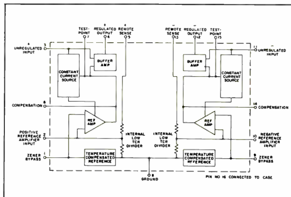
Functional Diagram
