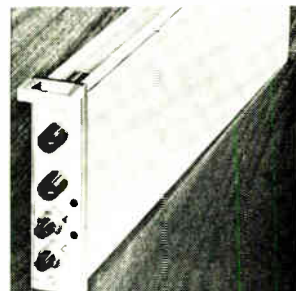
Triple mode differential amplifier model 7350 is designed to work from a wide variety of signal sources such as strain gauges, thermocouples, and piezoelectric transducers. It features a wide dynamic range of 60 db, ±20 v common-mode operating level, and isolated charge calibration circuitry. Dynamics Instrumentation Co., 513 Monterey Pass Rd., Monterey Park, Calif. [384]
