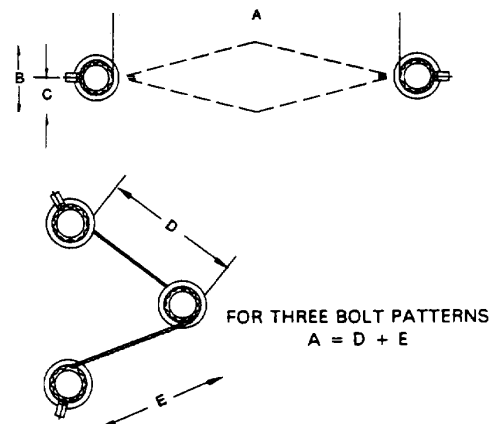
Figure 2-87. Safety Cable Flex Limits
