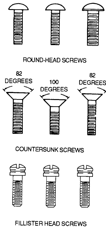
Figure 2-38. Machine Screws
