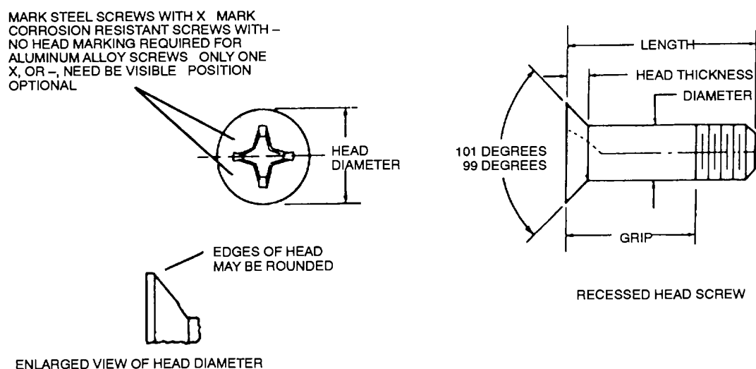
Figure 237. Flat-Head Screws
