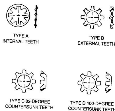
Figure 2-31. Teeth-Type Lockwashers
