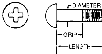
Figure 2-36. Structural Screw
