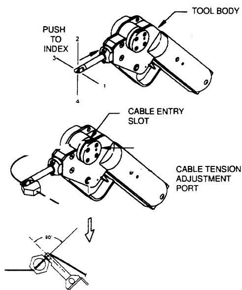
Figure 2-99. Pneumatic Safety Cable Application Tool
