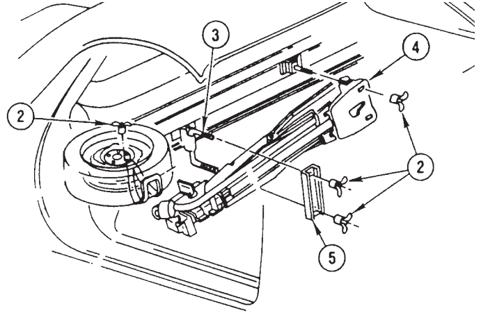
▶ 08-4200 Spare Tire and Jack Holder Kit Fits 1981-'88.
