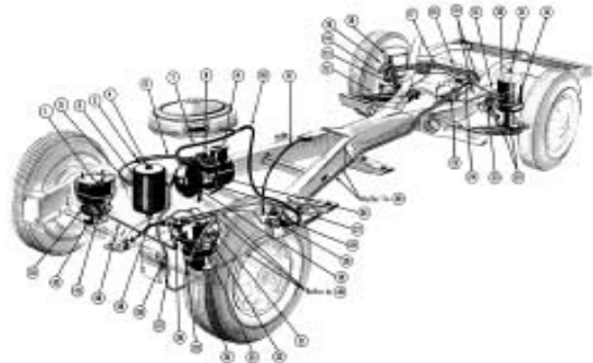
AIR SPRING LAYOUT—SERIES 1990 and CC Representative of 1988 and CC
