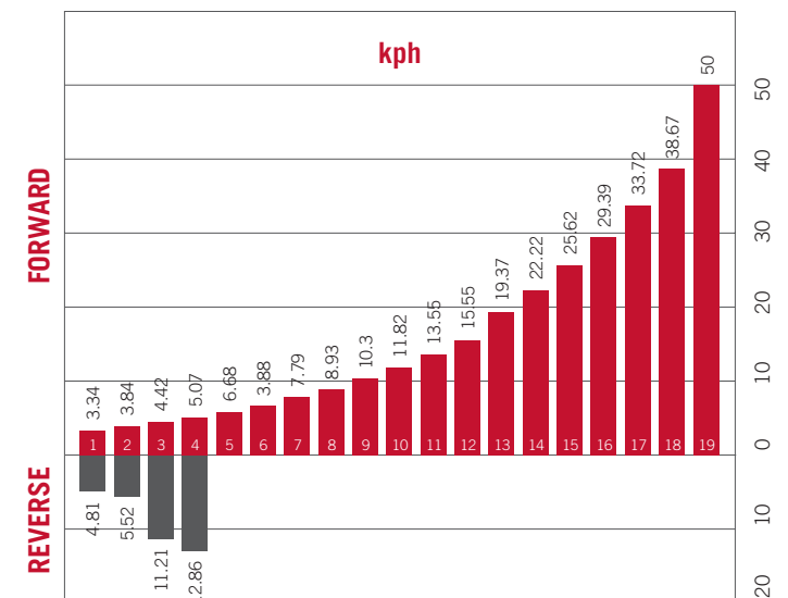
19x4 Full Powershift transmission 50 kph
