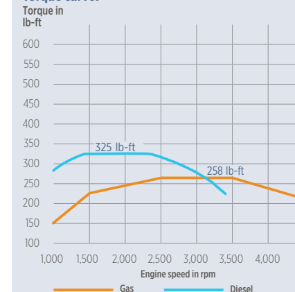
Torque curve:
