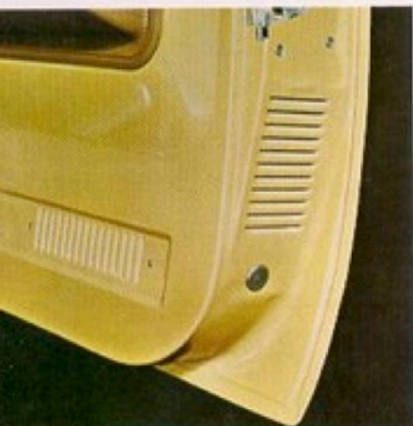
Full Time Power Ventilation on Pickups is standard with outside air supply through a large cowl-mounted plenum chamber. When ignition is on, air is routed through the cab for occupant comfort and exits through door-mounted valves that provide pressure relief when doors and windows are closed.
