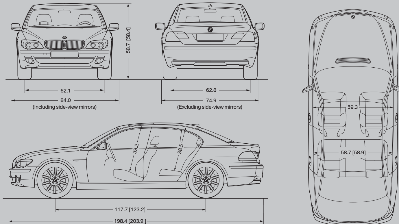
All dimensions shown in inches. Figures in [ ] apply to the 750Li/760Li; all other figures apply to 750i and 760i.
