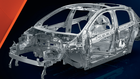
Very High Strength Steel (VHSS) body structure
