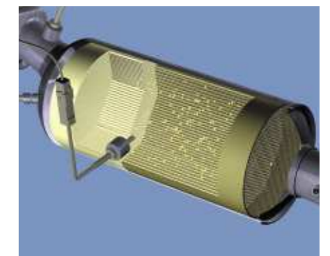
A state-of-the-art Diesel Particulate Filter System periodically burns off the particles that remain, virtually eliminating Diesel smoke, far exceeding current EU environmental standards.
