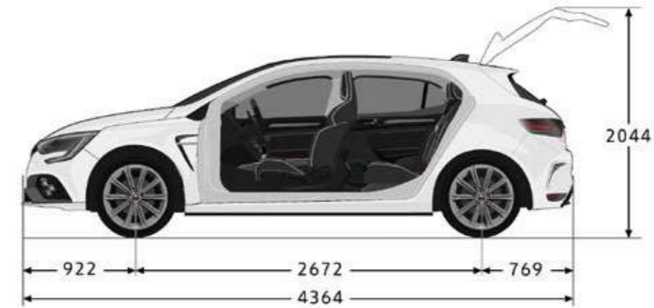
Dimensions (mm)
