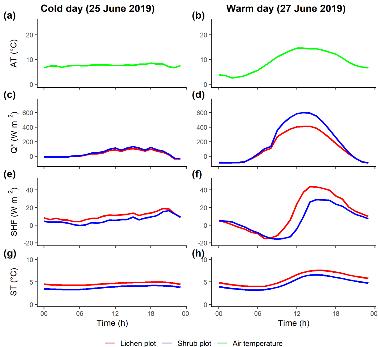
Figure 9: The reference air temperature (a,b) and difference in net radiation (c,d), soil heat flux (e,f) and soil temperature (g,h) between one lichen and paired shrub plot during a cold, cloudy day and a warm, sunny day. AT = reference air temperature, Q^* = net radiation, SHF = soil heat flux, and ST = soil temperature. The same paired plots are used for both days.
