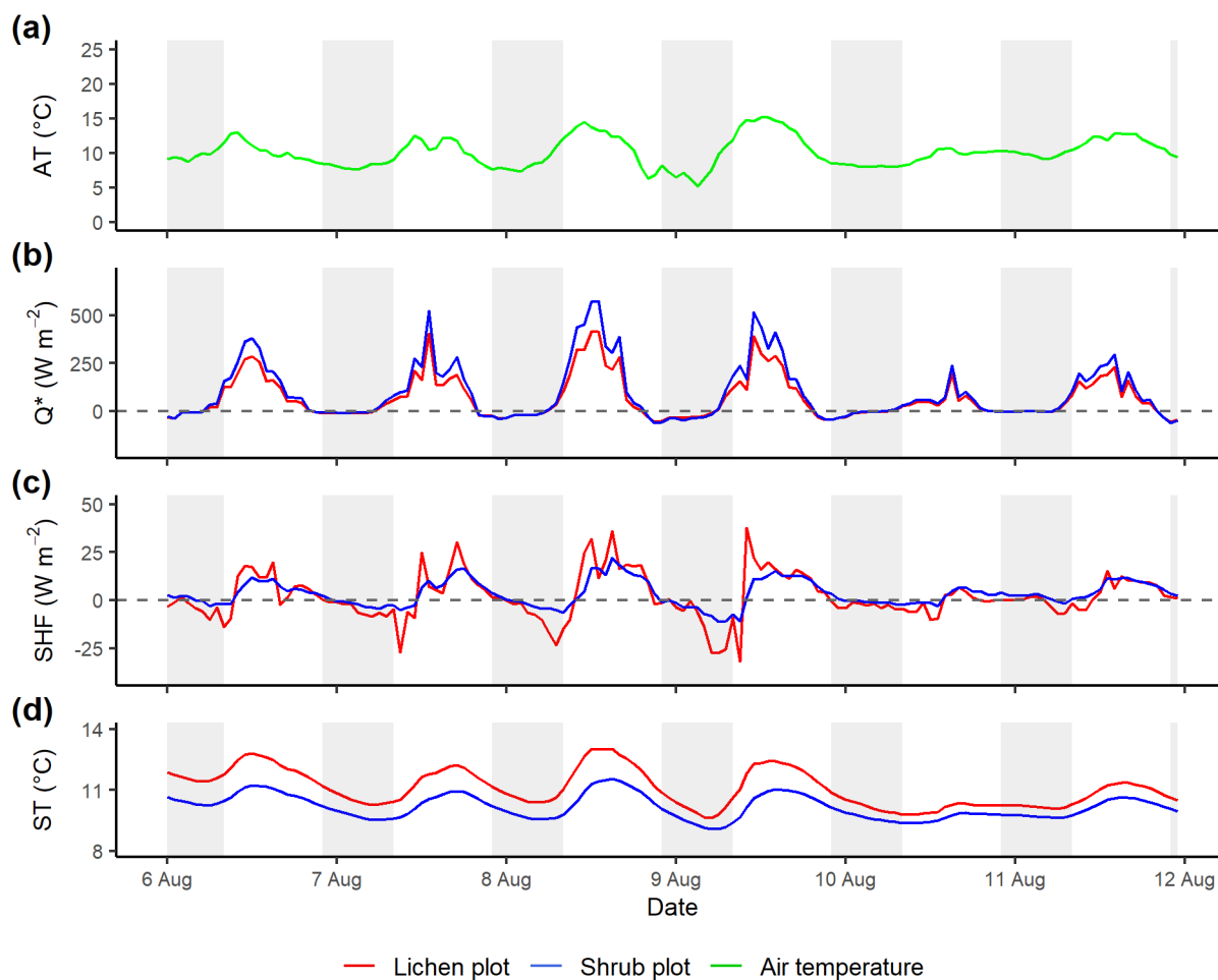
Figure D2: Time series of the reference air temperature (a), net radiation (b), soil heat flux (c) and soil temperature (d) between paired plots 3 of 2019. Time series are constructed with hourly averages. Shaded areas indicate nighttime (22:00–08:00 LT). AT = reference air temperature, Q^* = net radiation, SHF = soil heat flux, ST = soil temperature.
