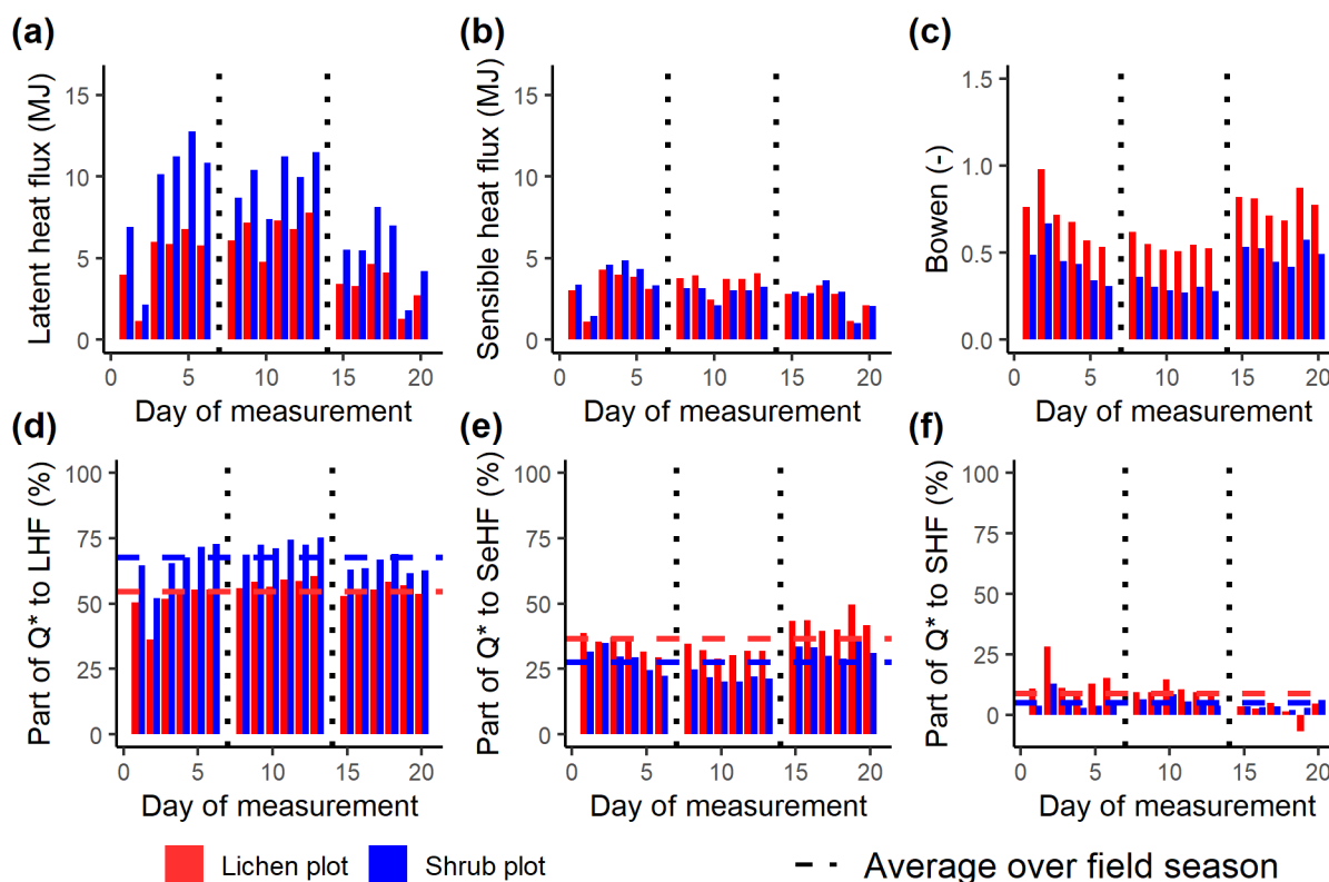
Figure F1: The calculated latent heat flux (a), sensible heat flux (b), Bowen ratio (c) and the fractions Q_E/Q^* (d), Q_H/Q^* (e) and Q_G/Q^* (f) per lichen and shrub plot of 2019. The vertical dotted lines indicate a plot change. LHF = latent heat flux, SeHF = sensible heat flux, SHF = soil heat flux, Q^* = net radiation. See Appendix C for the exact dates of the measurements of the three paired plots.
