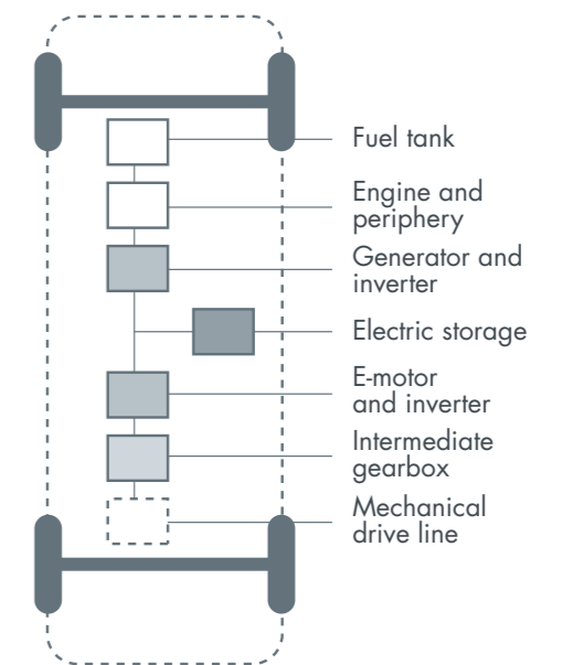
Trolley bus powertrain
