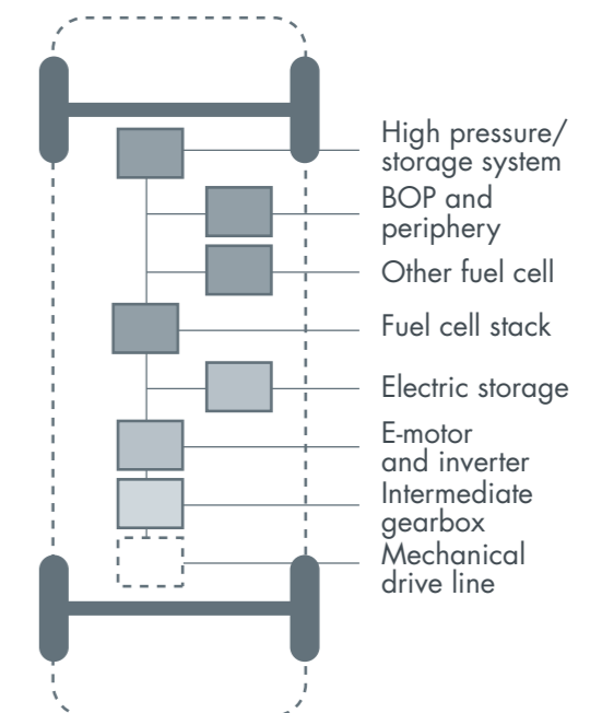
Serial hybrid powertrain
