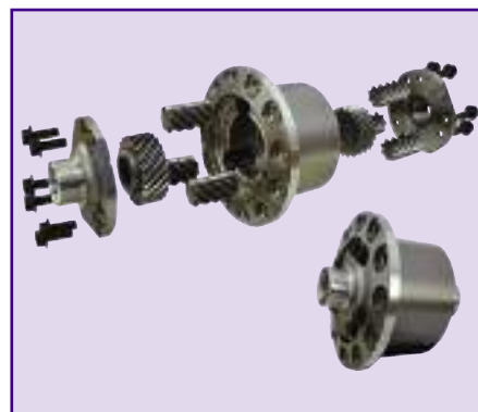
DETROIT TRUETRAC
