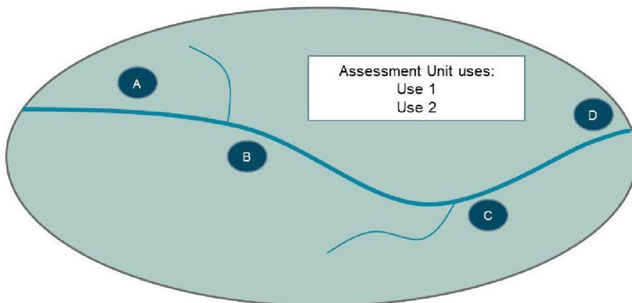
Figure 28. Process of composing overall AU category using site-level parameter assessments of beneficial use support.
