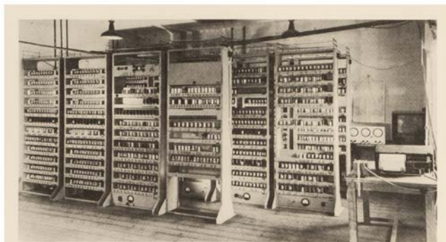
A general view of the EDSAC. The racks in the front row contain (from left to right): part of the store (two racks), pulse generator, and input-output units. Behind are three racks containing the control, and, in the rear, the remainder of the store (two racks) and the arithmetical unit (three racks). On the extreme right of the photograph may be seen the tapper for the input tape, and the teleprinter on which results are printed.
