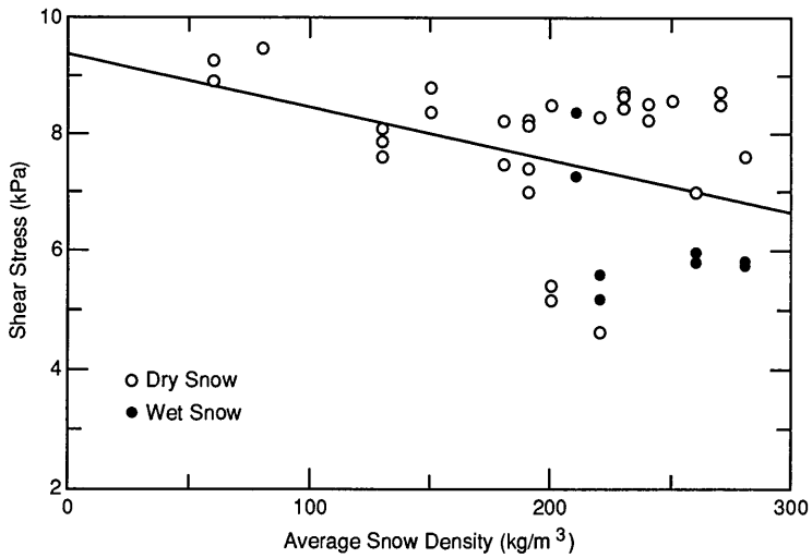
Figure 6 (cont'd). Shear stress versus initial snow density for various normal loads (shear annulus).
