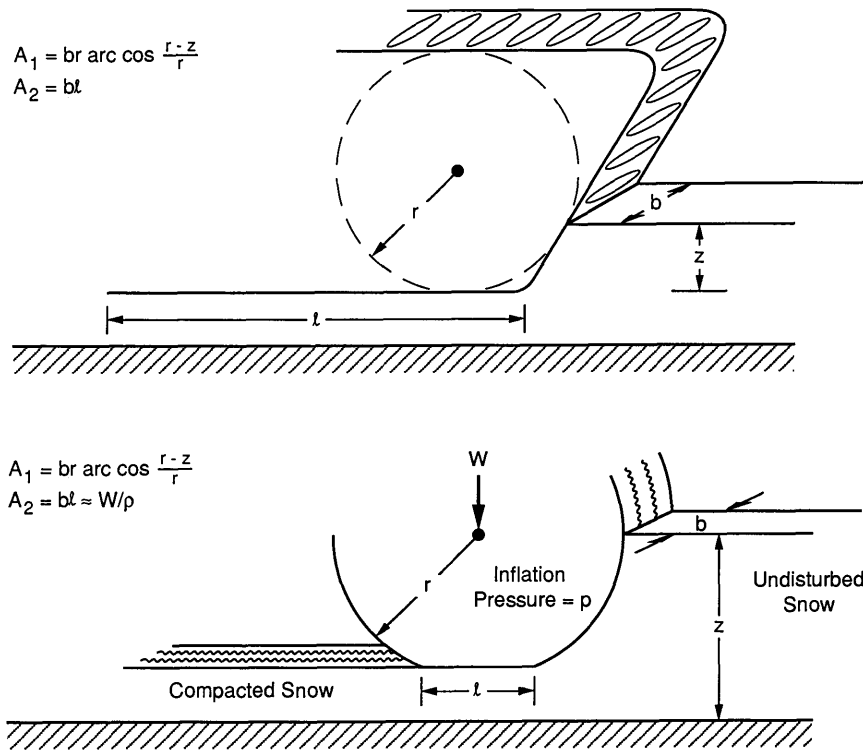
Figure A2. Tire and track contact areas for SSM1.0.
