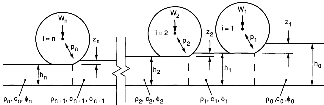
Figure A3. Depiction of progressive change in snow parameters with tire or track passage.
