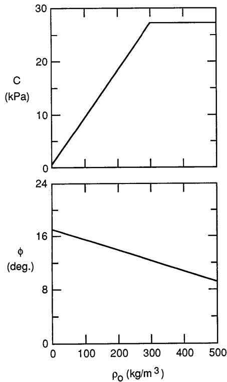
Figure A1. Relationship between snow strength and initial density as used in SSM1.0.
