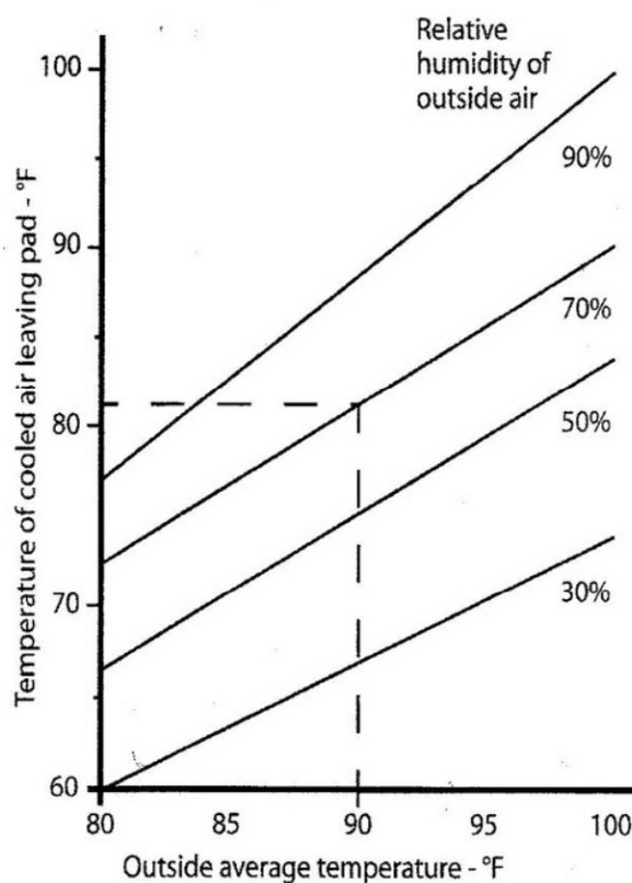
Effect of relative humidity of outside air on evaporative cooling
