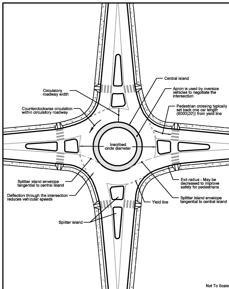
FIGURE IV-13. TYPICAL ROUNDABOUT
