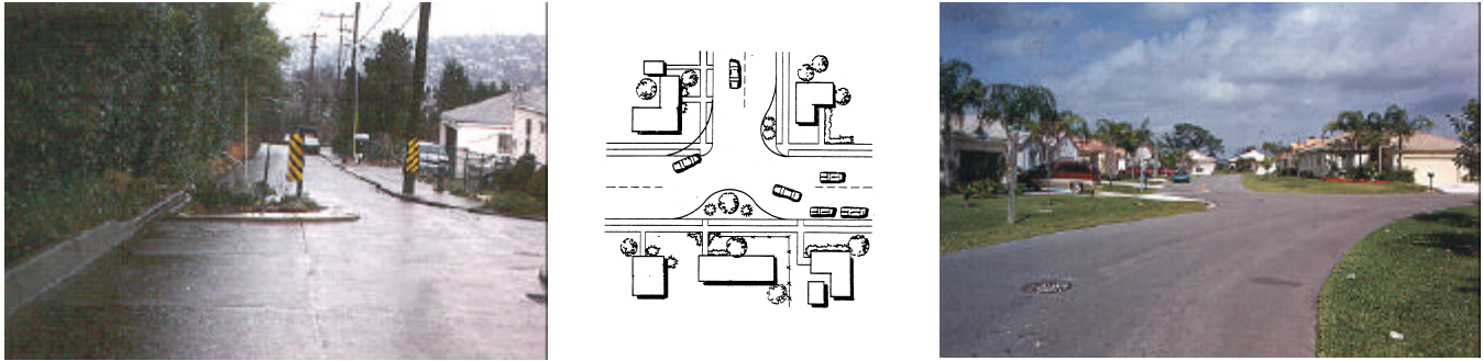
FIGURE III-14. REALIGNED INTERSECTIONS
