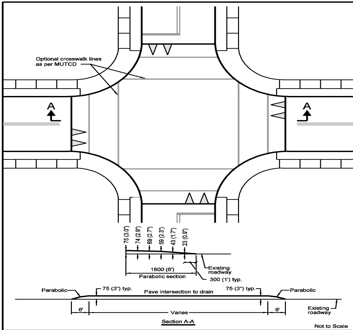
FIGURE IV-8. TYPICAL RAISED INTERSECTION
