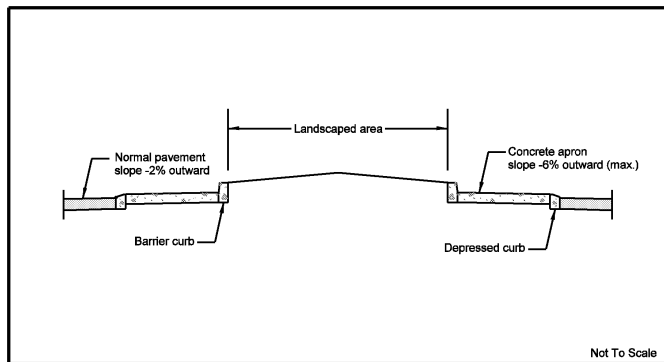
FIGURE IV-11. ISLAND SECTION
