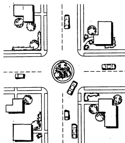
FIGURE III-10. MINI-TRAFFIC CIRCLES
