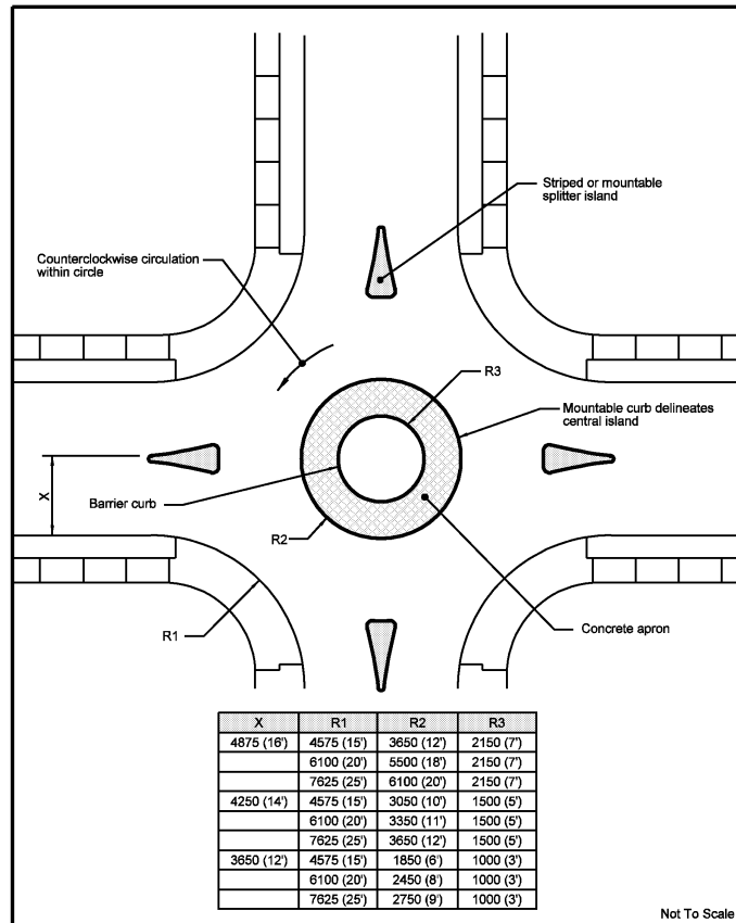
FIGURE IV-10. TYPICAL MINI-TRAFFIC CIRCLE
