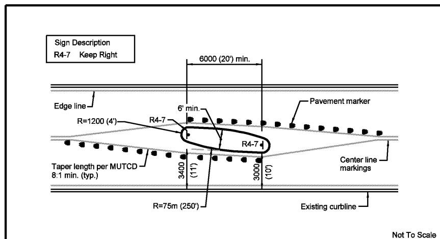
FIGURE IV-18. TYPICAL CENTER ISLAND NARROWING
