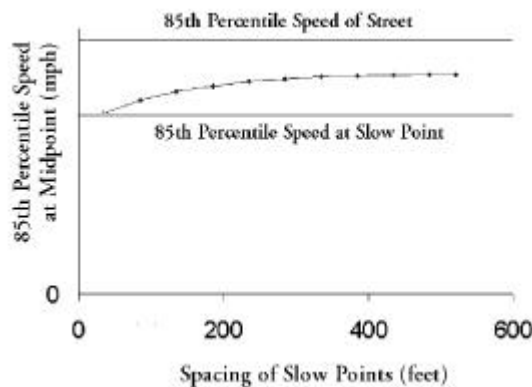
FIGURE IV-21. SPEED VS. SPACING OF SLOW POINTS
