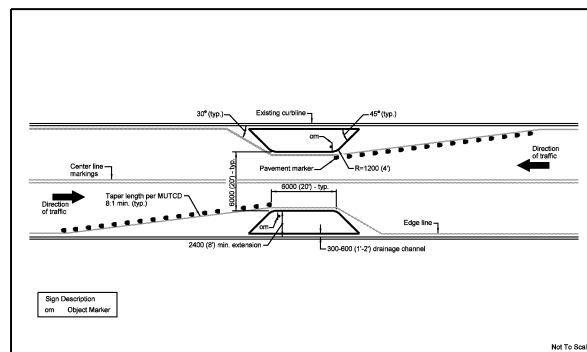
FIGURE IV-17. TYPICAL CHOKER
