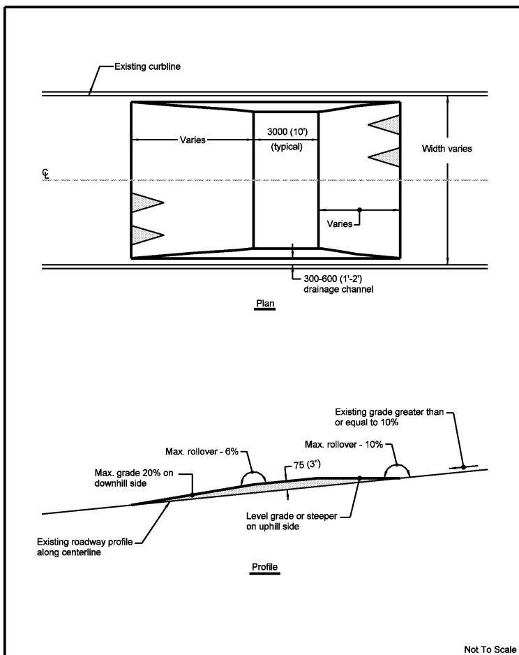
FIGURE IV-9. VERTICAL PROFILE MODIFIED TO BE SAFE AND EFFECTIVE ON A GRADE
