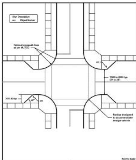
FIGURE IV-16. TYPICAL NECKDOWN
