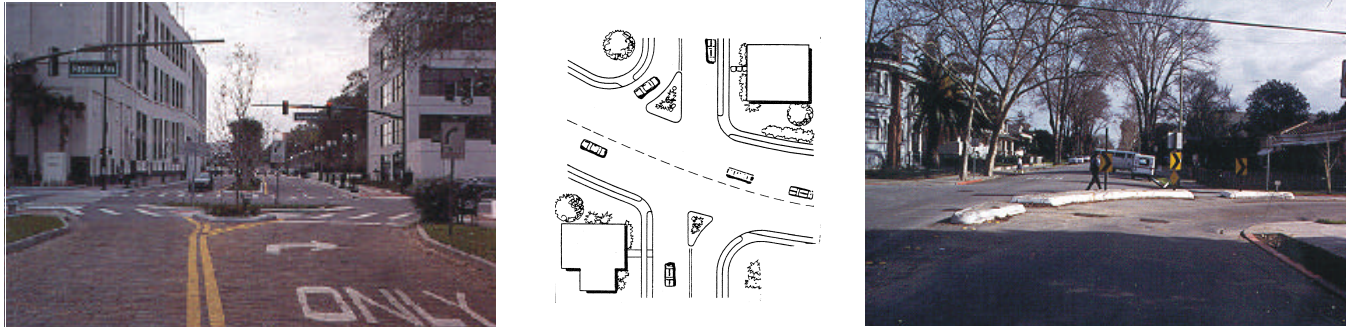
FIGURE III-5. FORCED TURN ISLANDS
