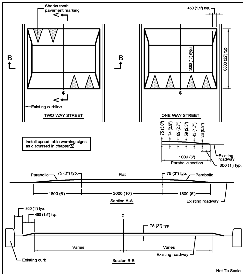
FIGURE IV-6. TYPICAL SPEED TABLE
