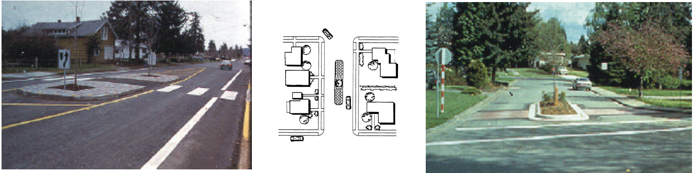
FIGURE III-17. CENTER ISLANDS
