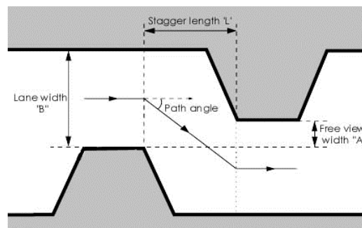
FIGURE IV-20. GEOMETRIC PARAMETERS AFFECTING CROSSING SPEEDS
