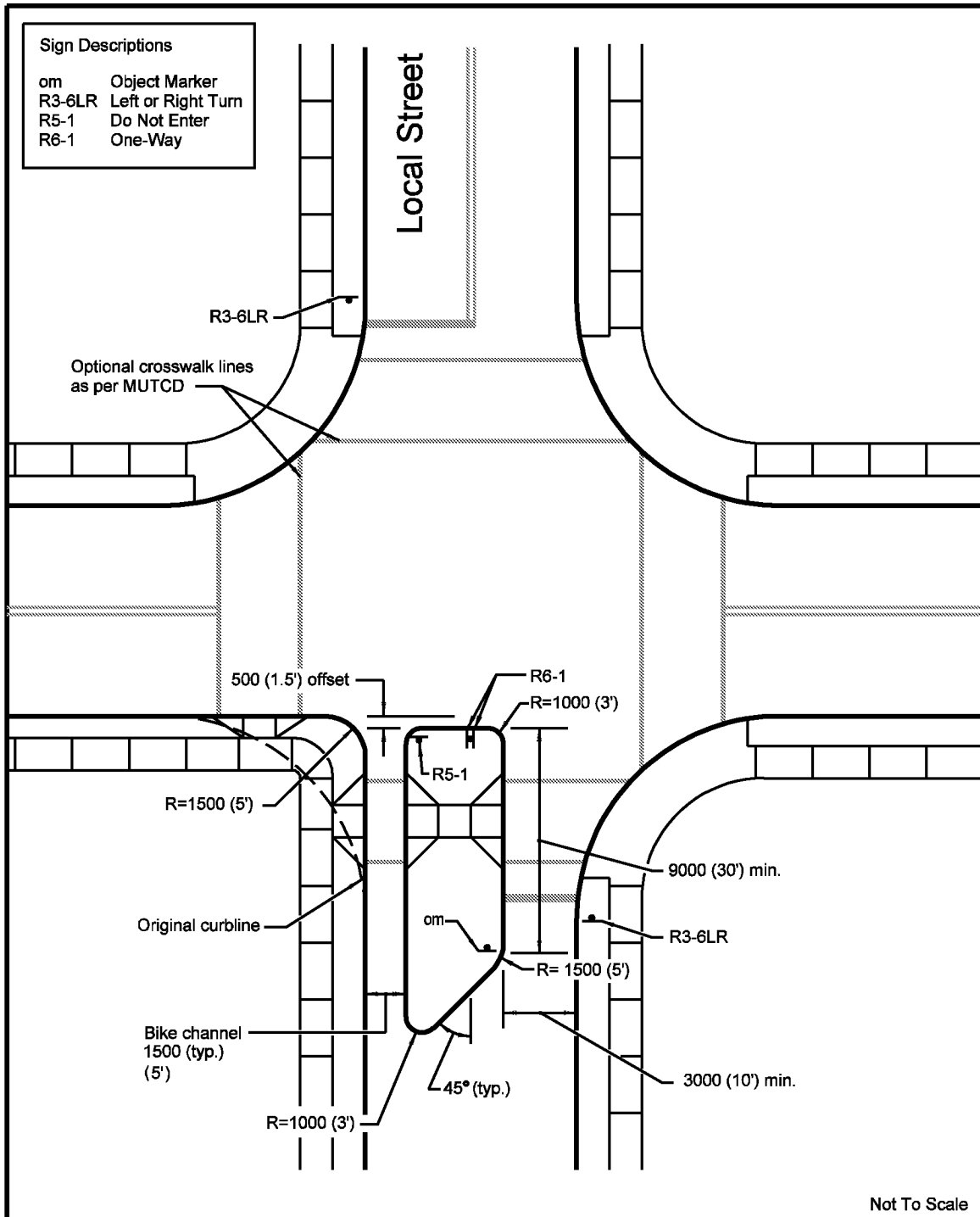
FIGURE IV-1. TYPICAL HALF CLOSURE
