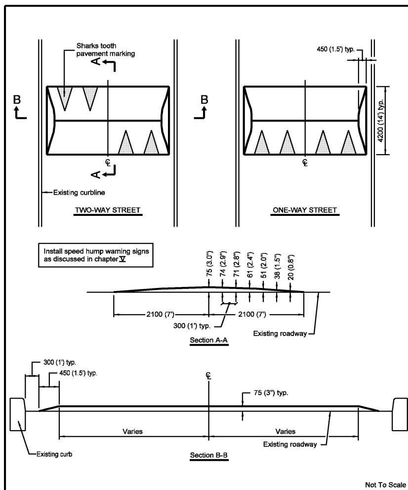
FIGURE IV-5. TYPICAL SPEED BUMP
