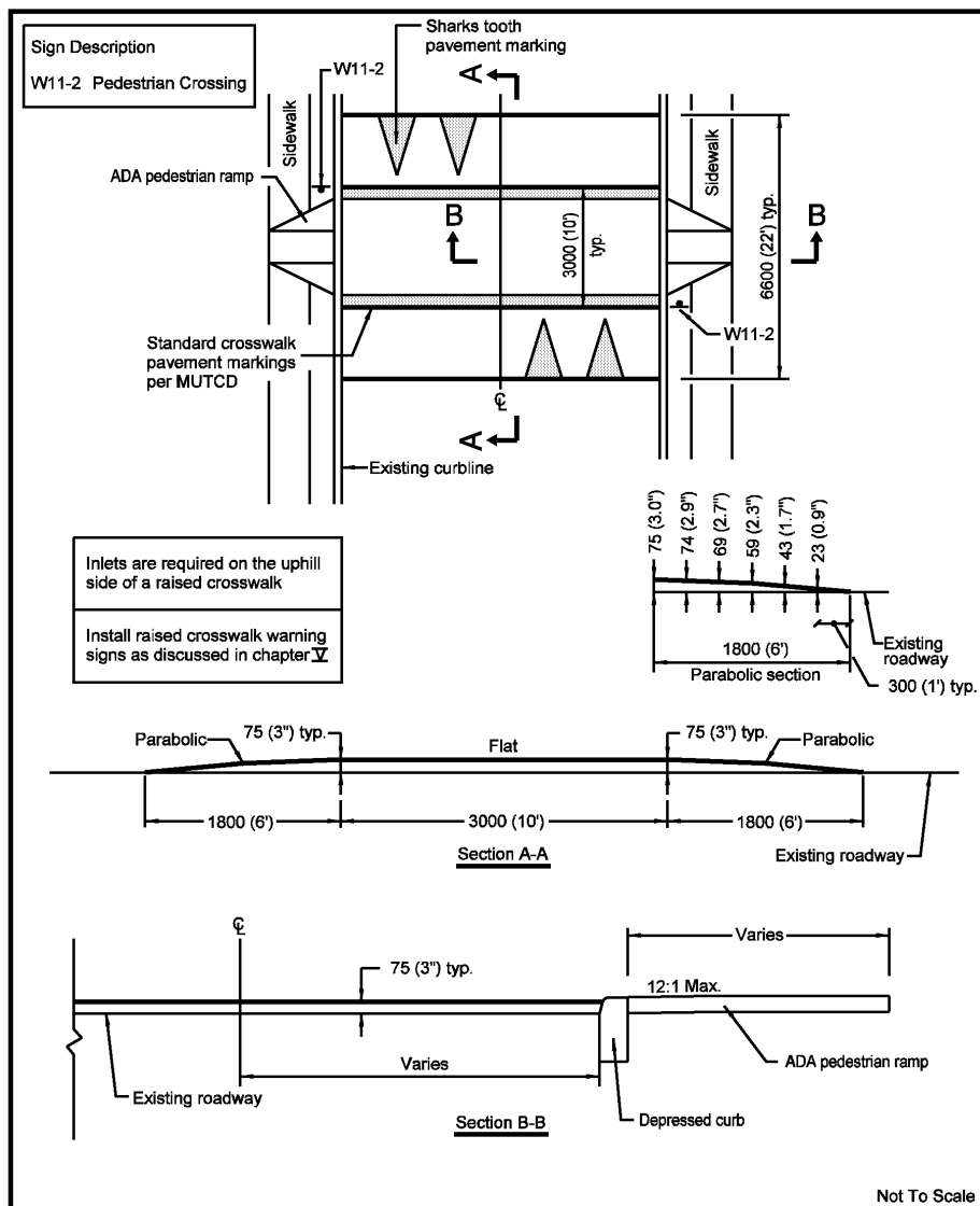
FIGURE IV-7. TYPICAL RAISED CROSSWALK
