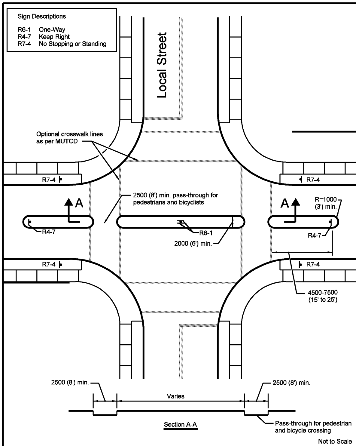
FIGURE IV-3. TYPICAL MEDIAN BARRIER
