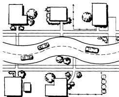
FIGURE III-13. CHICANES
