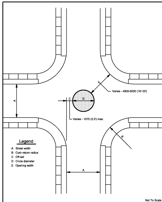
FIGURE IV-12. ALTERNATIVE DESIGN FOR A MINI-CIRCLE
