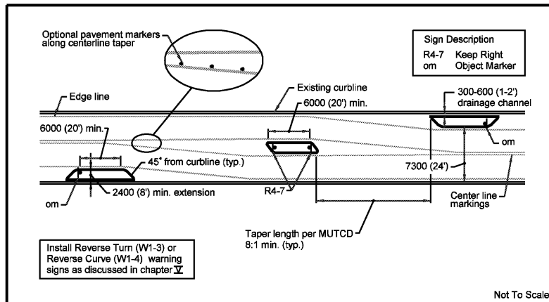
FIGURE IV-15. TYPICAL LATERAL SHIFT
