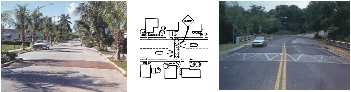
FIGURE III-6. SPEED HUMPS
