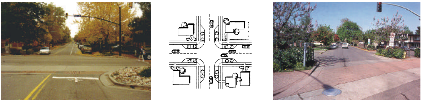
FIGURE III-15. NECKDOWNS
