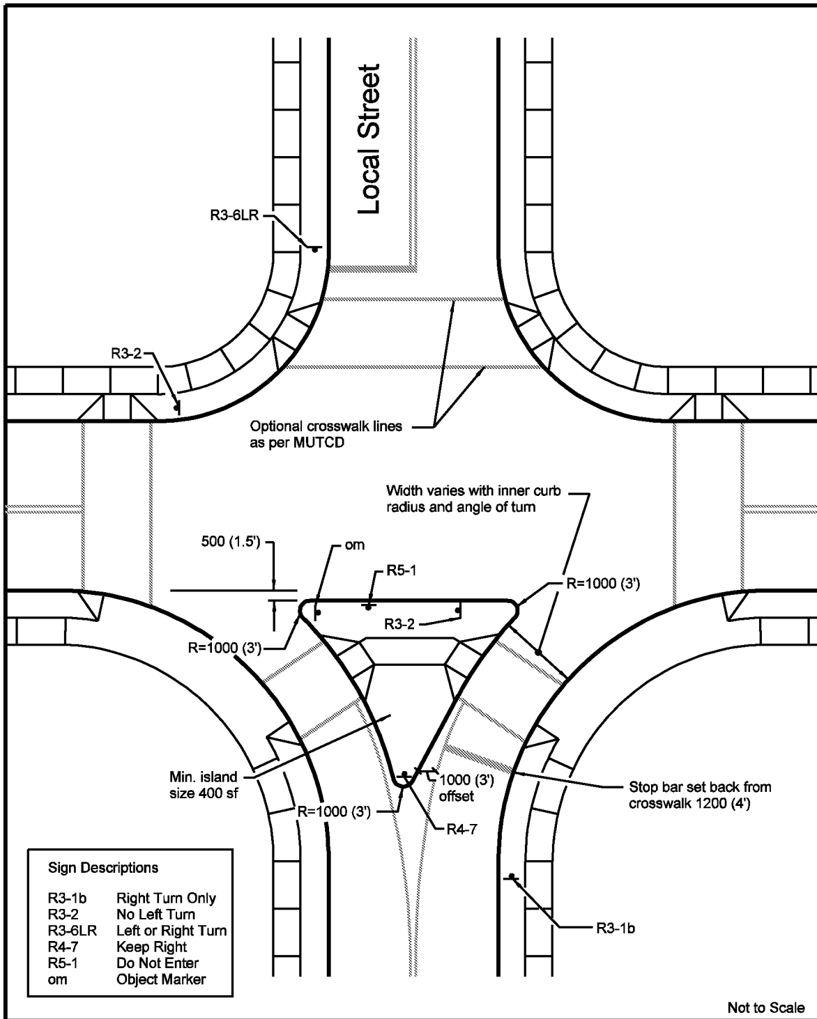
FIGURE IV-4. TYPICAL FORCED TURN ISLAND
