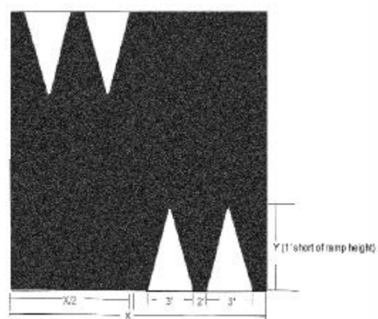
FIGURE V-10. STANDARD MARKING PATTERN FOR VERTICAL MEASURES
