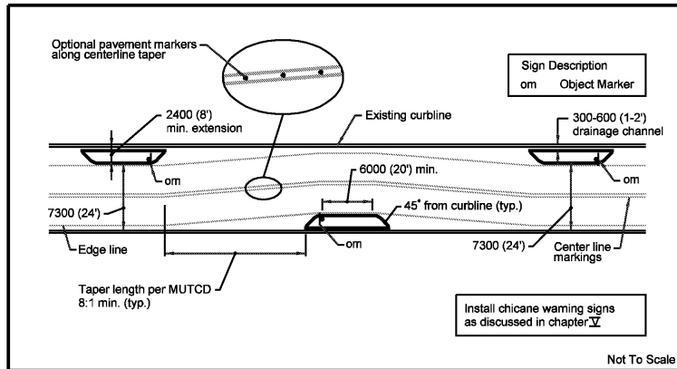
FIGURE IV-14. TYPICAL CHICANE
