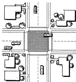
FIGURE III-9. RAISED INTERSECTIONS
