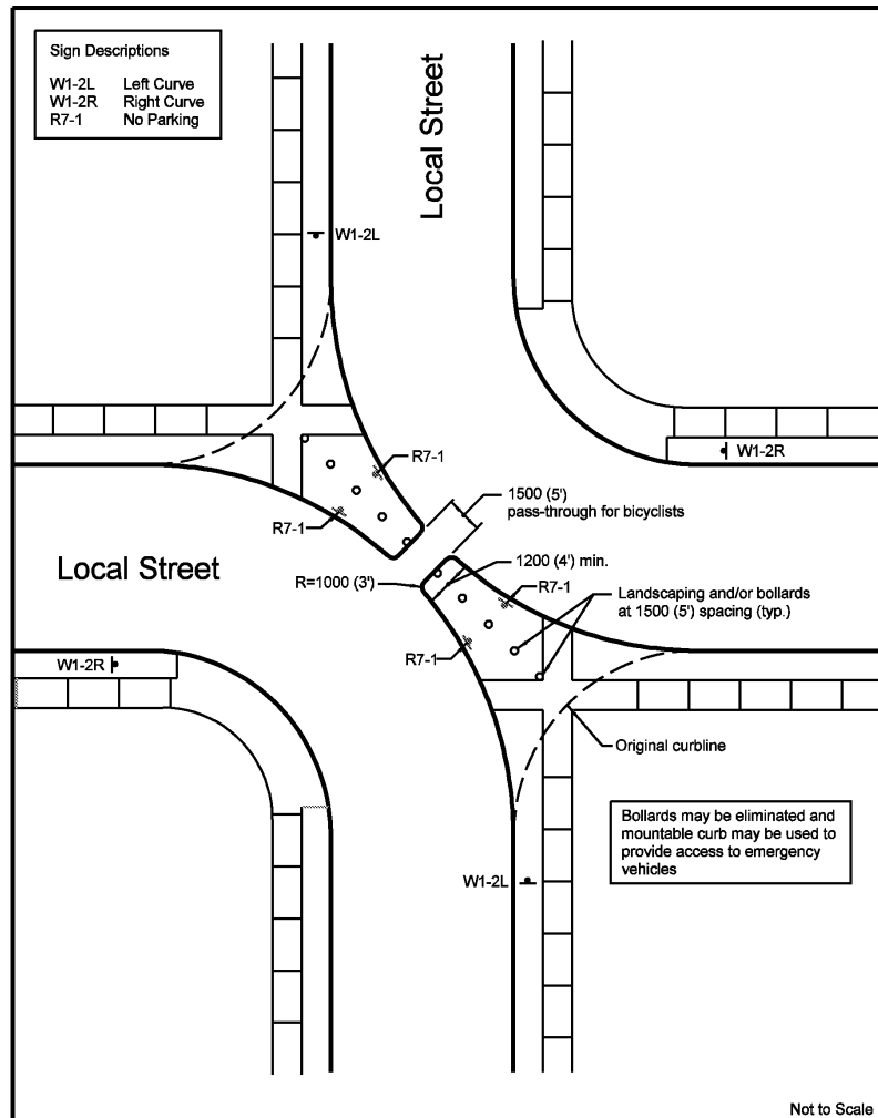
FIGURE IV-2. TYPICAL DIAGONAL DIVERTER
