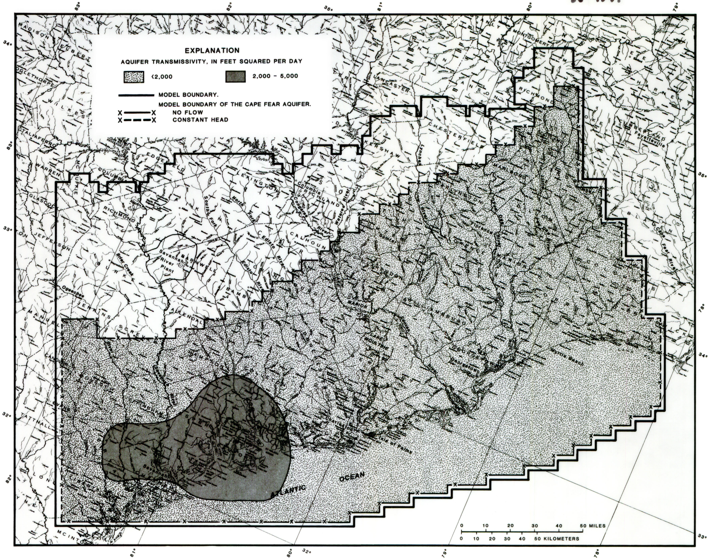
Figure 27.— Simulated transmissivity of the Cape Fear aquifer.
