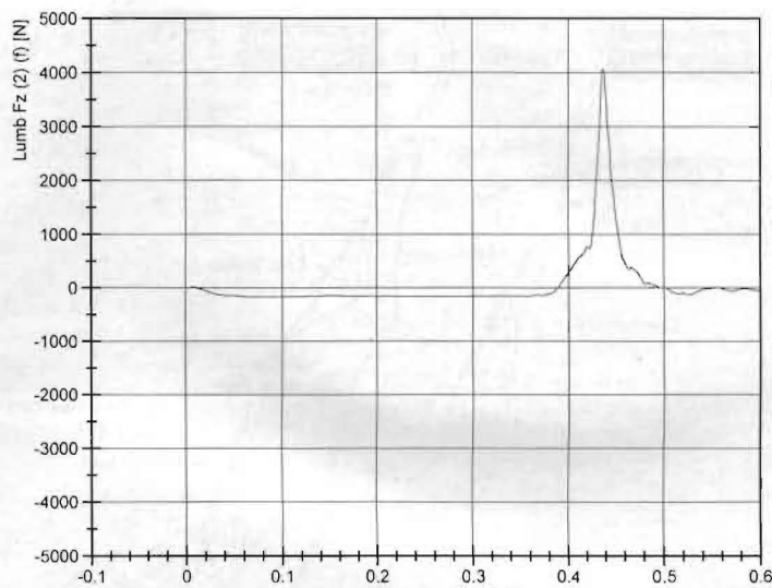
Above: In the last test, number G06, when failure of the undercarriage occurred, a sharply-peaking force with a high rate of rise was felt in the lumbar spine Z axis in the rear cockpit. It was much greater than the load in the spine of the front pilot
