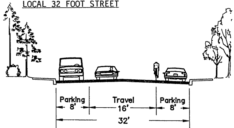
LOCAL 32 FOOT STREET
