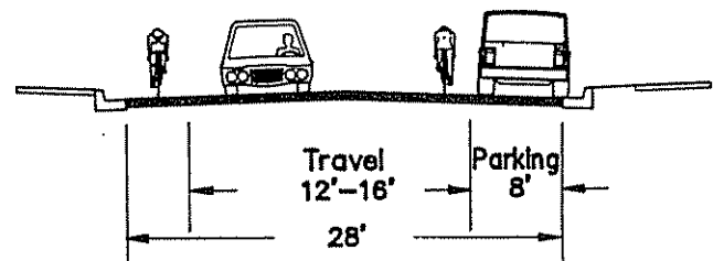
LOCAL 28 FOOT STREET
