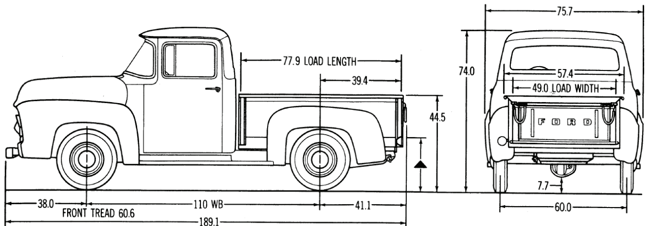
ALL DIMENSIONS WITH 6.70 x 15-4 P.R. TIRES (LOADED)
