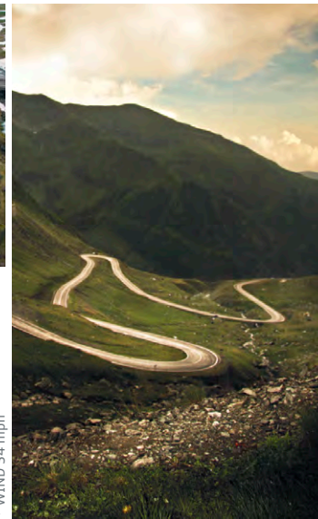
▼ WIND 54 mph
